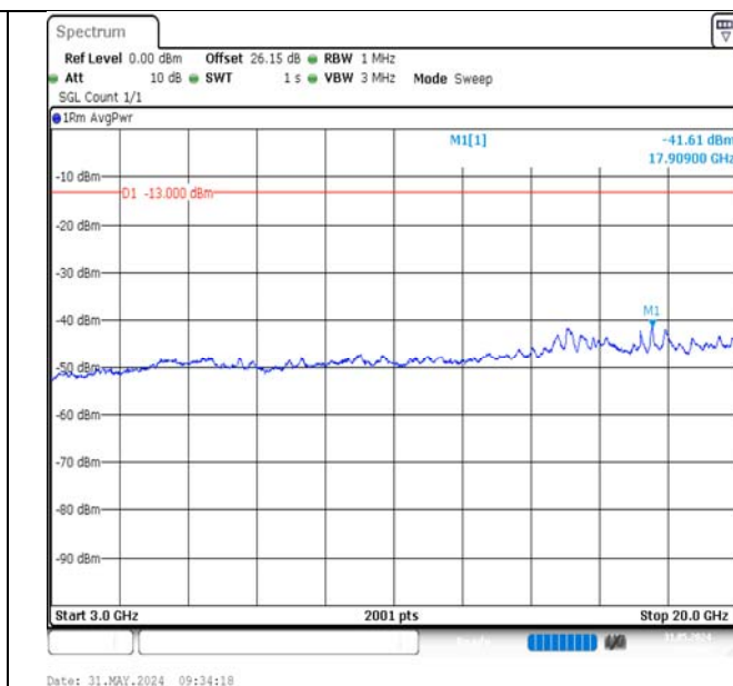
Band2-20MHz-16QAM-19100-1RB#0-3000~20000-PASS
