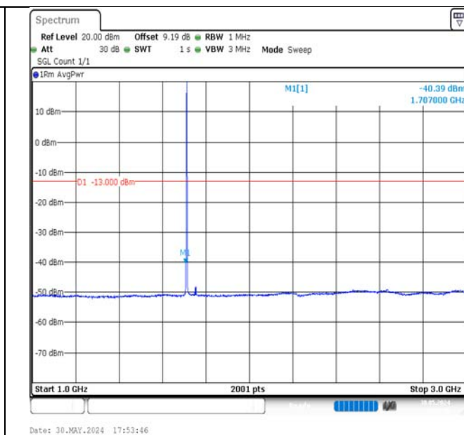
Band4-1.4MHz-QPSK-19957-1RB#5-1000~3000-PASS
