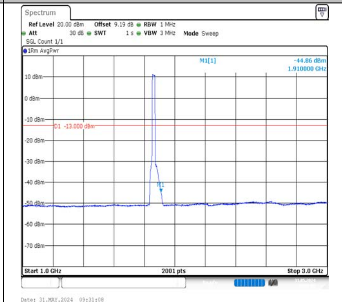
Band2-20MHz-16QAM-18700-100RB#0-1000~3000-PASS
