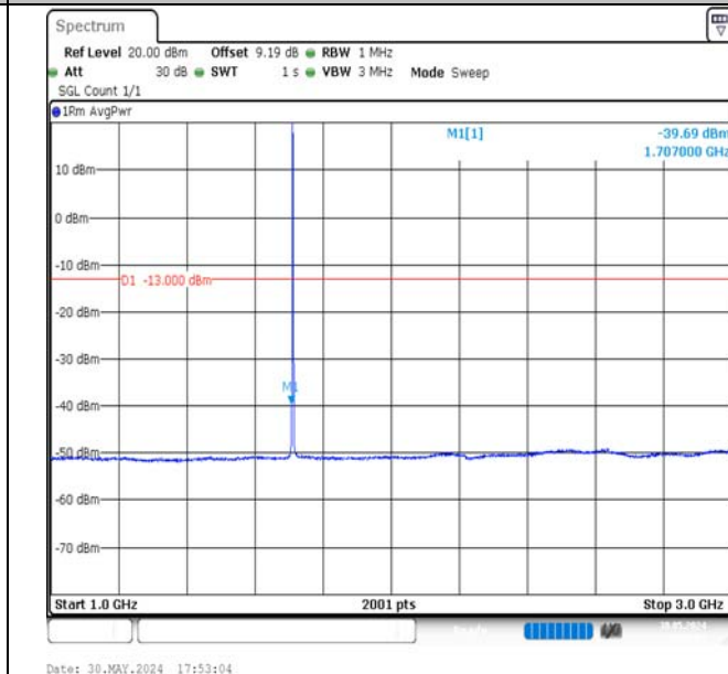
Band4-1.4MHz-QPSK-19957-1RB#0-1000~3000-PASS
