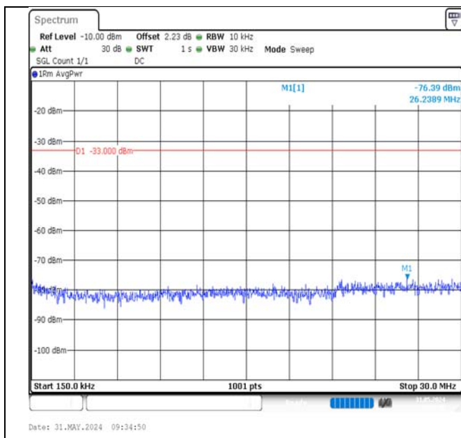
Band2-20MHz-16QAM-19100-1RB#99-0.15~30-PASS
