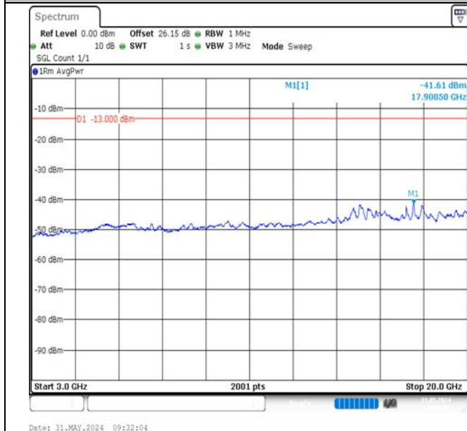
Band2-20MHz-16QAM-18900-1RB#0-3000~20000-PASS
