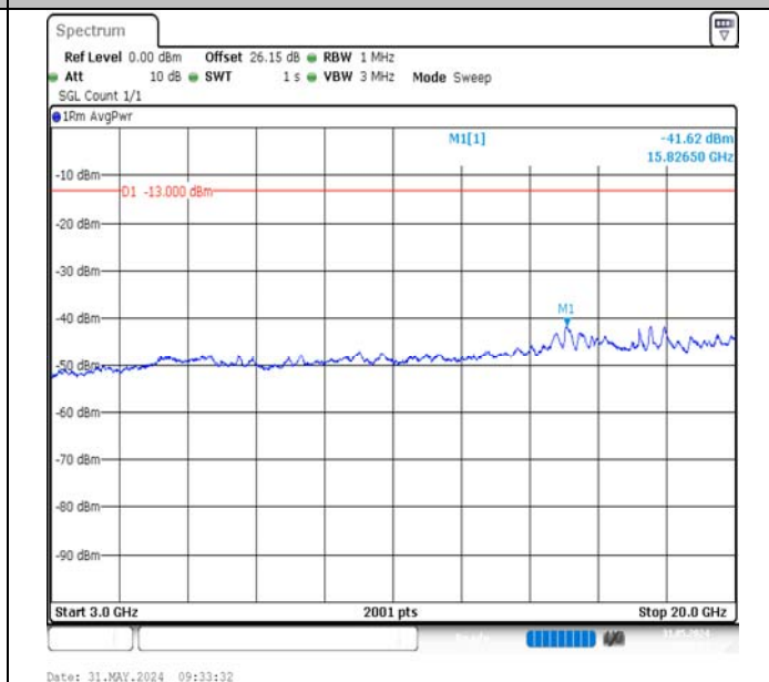
Band2-20MHz-16QAM-18900-100RB#0-3000~20000-PASS
