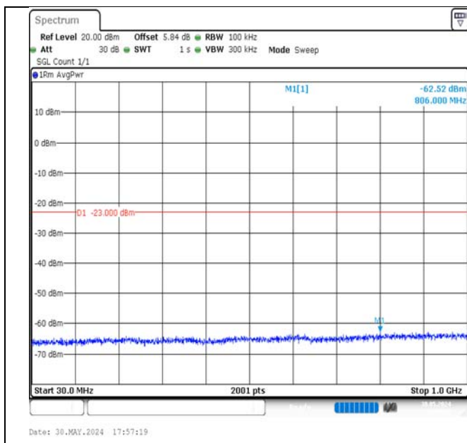
Band4-1.4MHz-QPSK-20393-1RB#0-30~1000-PASS
