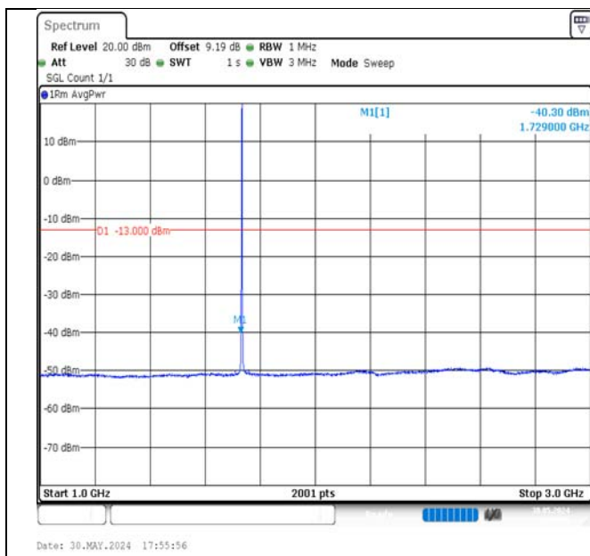
Band4-1.4MHz-QPSK-20175-1RB#5-1000~3000-PASS
