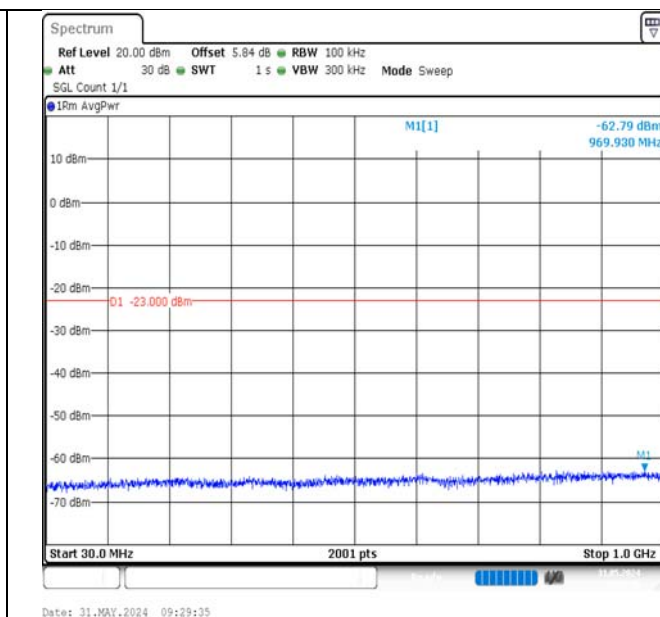
Band2-20MHz-16QAM-18700-1RB#0-30~1000-PASS
