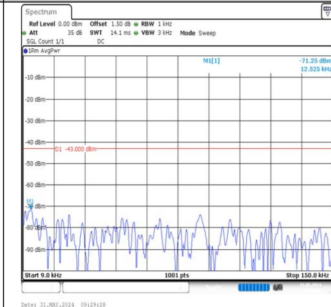
Band2-20MHz-16QAM-18700-1RB#0-0.009~0.15-PASS
