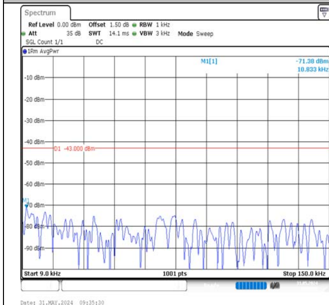
Band2-20MHz-16QAM-19100-100RB#0-0.009~0.15-PASS
