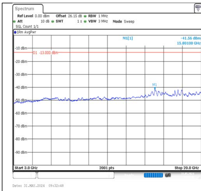
Band2-20MHz-16QAM-18900-1RB#99-3000~20000-PASS
