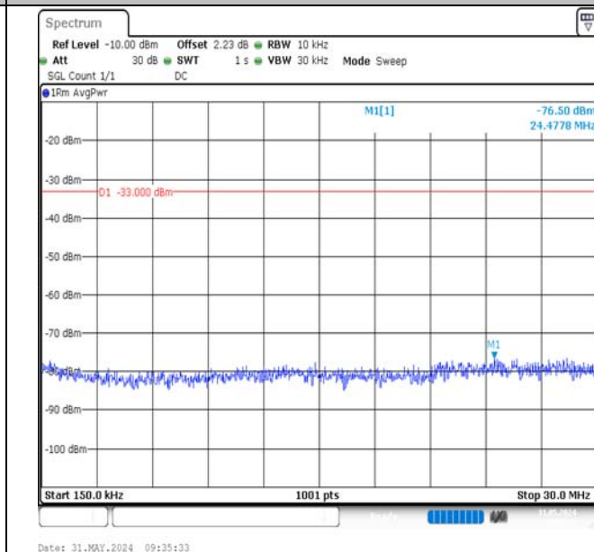
Band2-20MHz-16QAM-19100-100RB#0-0.15~30-PASS
