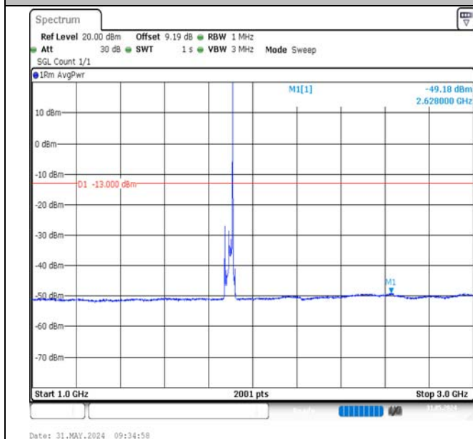
Band2-20MHz-16QAM-19100-1RB#99-1000~3000-PASS
