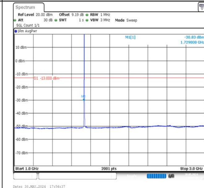
Band4-1.4MHz-QPSK-20175-6RB#0-1000~3000-PASS
