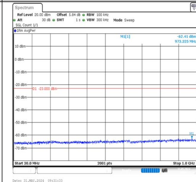
Band2-20MHz-QPSK-18900-1RB#0-30~1000-PASS
