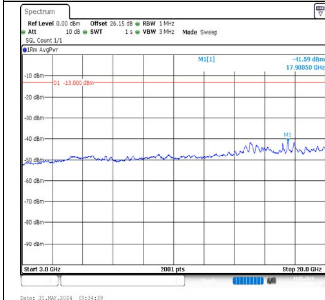
Band2-20MHz-QPSK-19100-1RB#99-3000~20000-PASS
