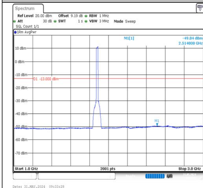
Band2-20MHz-16QAM-18900-100RB#0-1000~3000-PASS
