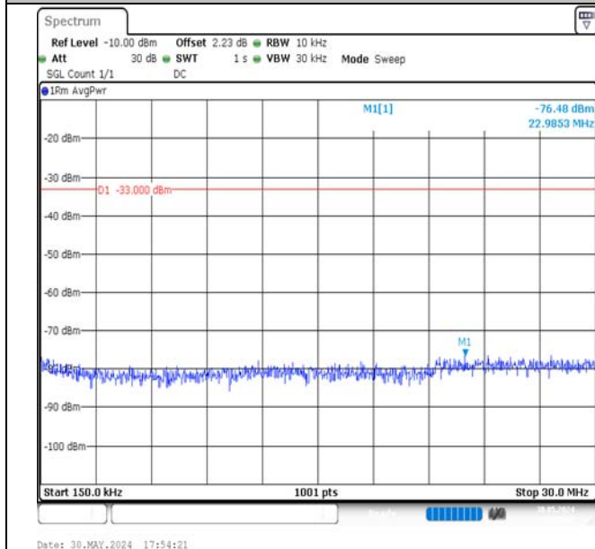
Band4-1.4MHz-QPSK-19957-6RB#0-0.15~30-PASS
