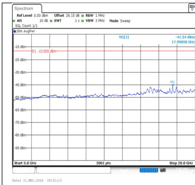
Band2-20MHz-16QAM-18700-100RB#0-3000~20000-PASS
