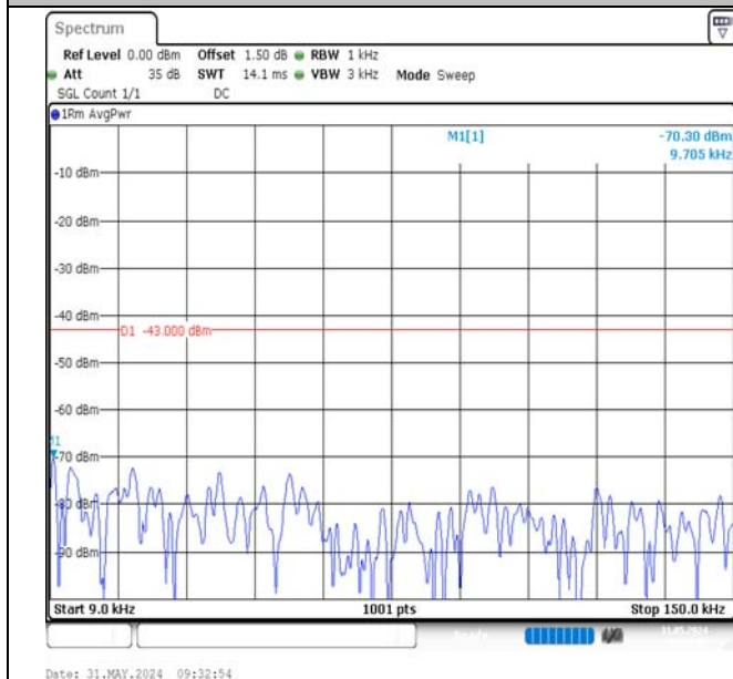
Band2-20MHz-QPSK-18900-100RB#0-0.009~0.15-PASS
