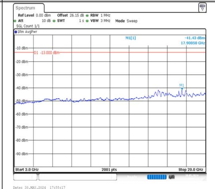
Band4-1.4MHz-QPSK-20175-1RB#0-3000~20000-PASS
