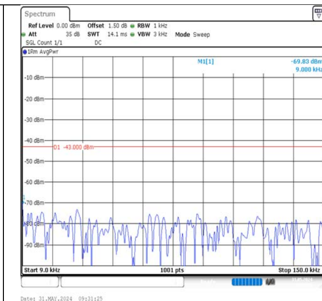
Band2-20MHz-QPSK-18900-1RB#0-0.009~0.15-PASS
