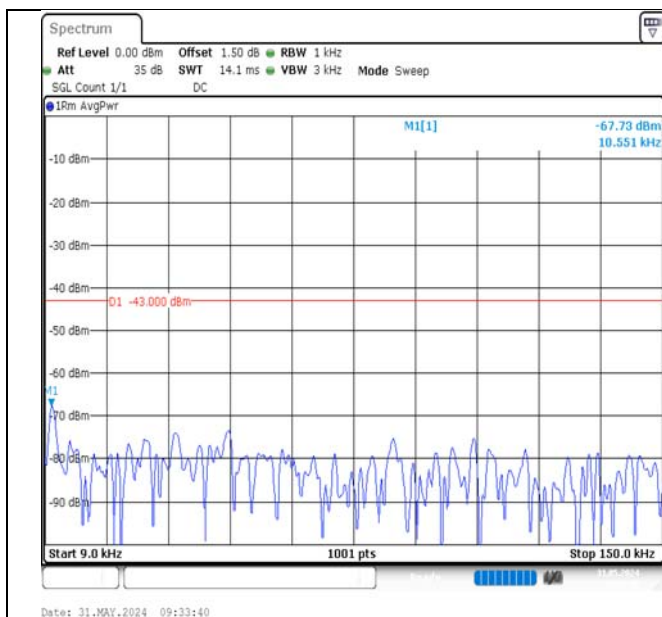
Band2-20MHz-QPSK-19100-1RB#0-0.009~0.15-PASS
