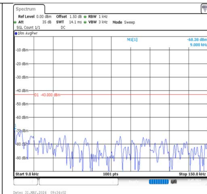
Band2-20MHz-16QAM-19100-1RB#0-0.009~0.15-PASS
