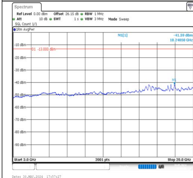
Band4-1.4MHz-QPSK-20393-1RB#0-3000~20000-PASS
