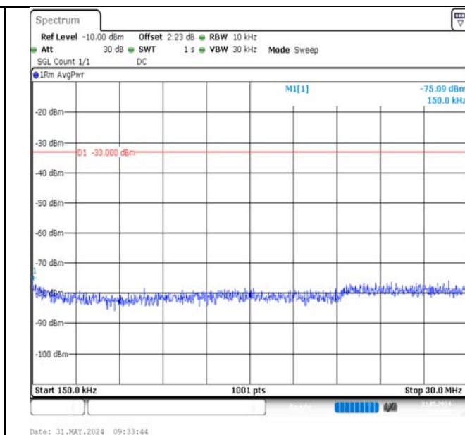
Band2-20MHz-QPSK-19100-1RB#0-0.15~30-PASS
