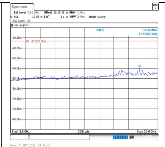
Band2-20MHz-QPSK-18900-1RB#0-3000~20000-PASS
