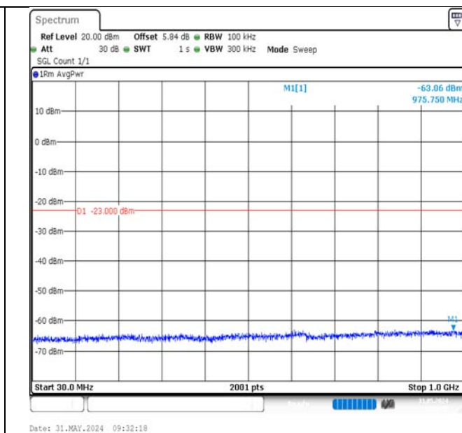
Band2-20MHz-QPSK-18900-1RB#99-30~1000-PASS
