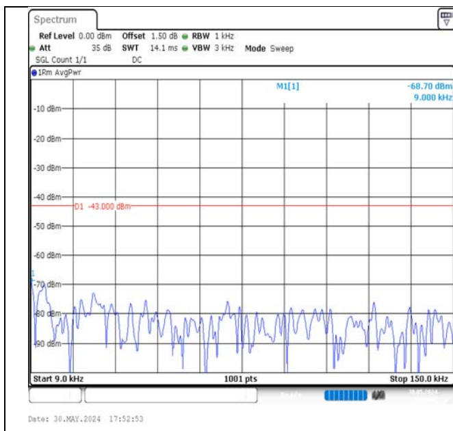
Band4-1.4MHz-QPSK-19957-1RB#0-0.009~0.15-PASS
