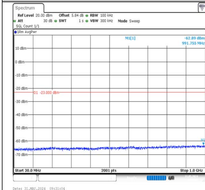
Band2-20MHz-16QAM-18700-100RB#0-30~1000-PASS
