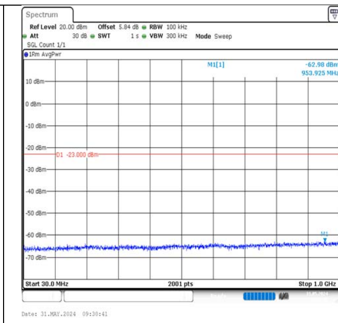
Band2-20MHz-QPSK-18700-100RB#0-30~1000-PASS
