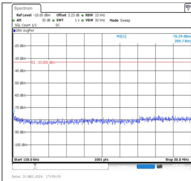
Band4-1.4MHz-QPSK-20393-6RB#0-0.15~30-PASS
