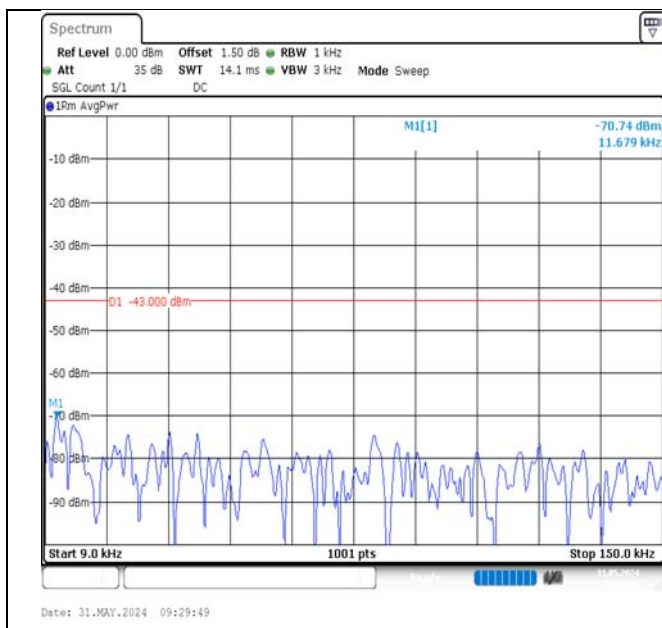
Band2-20MHz-QPSK-18700-1RB#99-0.009~0.15-PASS
