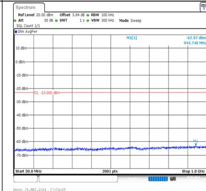
Band4-1.4MHz-QPSK-19957-6RB#0-30~1000-PASS
