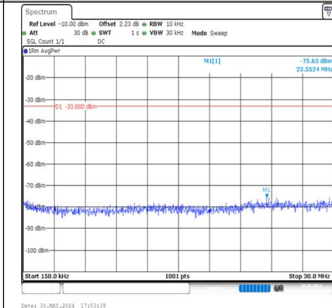
Band4-1.4MHz-QPSK-19957-1RB#5-0.15~30-PASS
