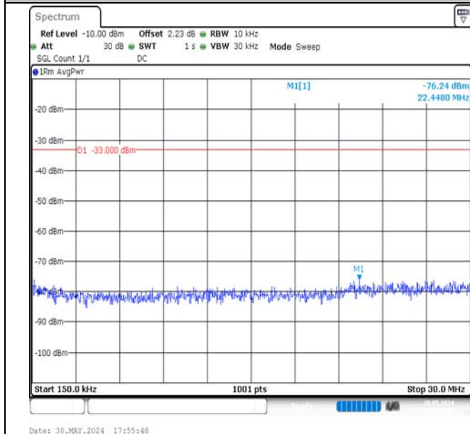
Band4-1.4MHz-QPSK-20175-1RB#5-0.15~30-PASS
