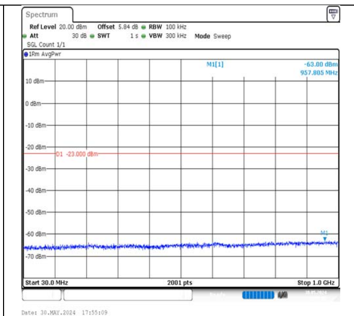
Band4-1.4MHz-QPSK-20175-1RB#0-30~1000-PASS
