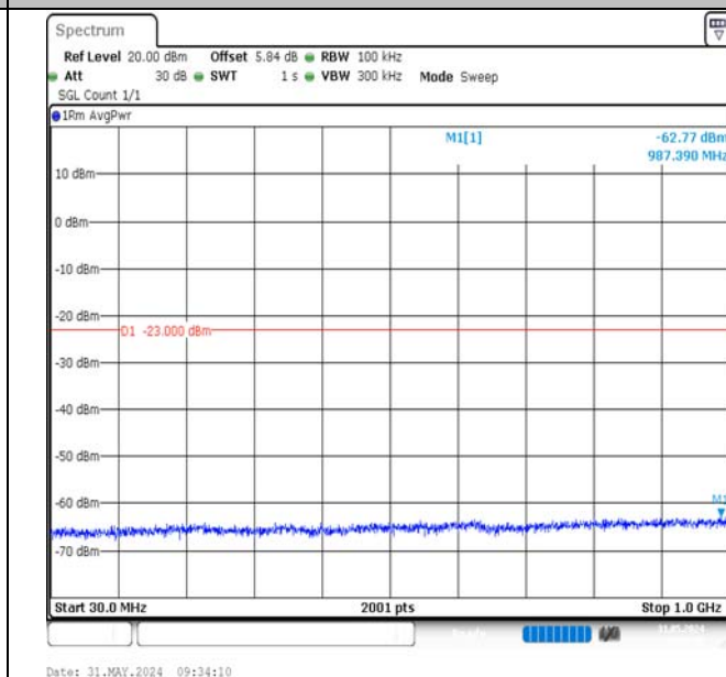
Band2-20MHz-16QAM-19100-1RB#0-30~1000-PASS
