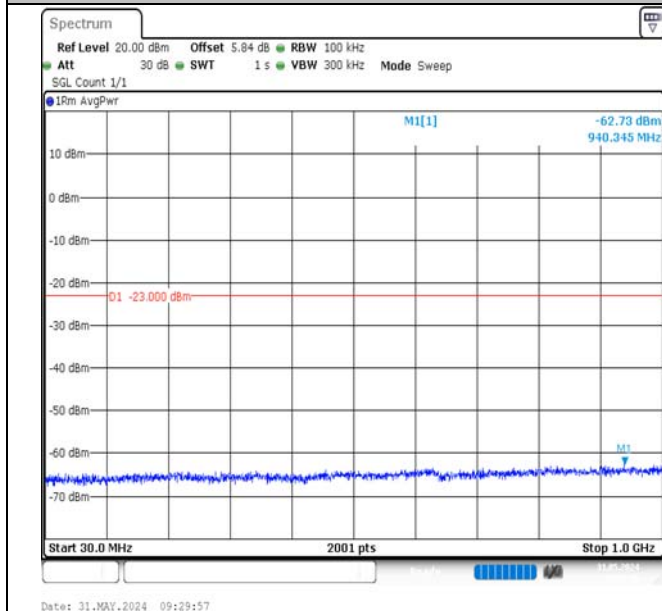
Band2-20MHz-QPSK-18700-1RB#99-30~1000-PASS
