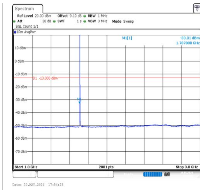
Band4-1.4MHz-QPSK-19957-6RB#0-1000~3000-PASS
