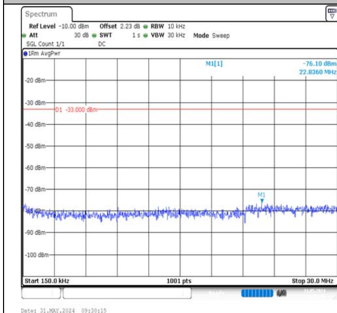
Band2-20MHz-16QAM-18700-1RB#99-0.15~30-PASS
