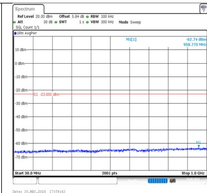
Band4-1.4MHz-QPSK-20393-6RB#0-30~1000-PASS
