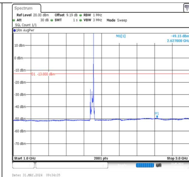
Band2-20MHz-QPSK-19100-1RB#99-1000~3000-PASS
