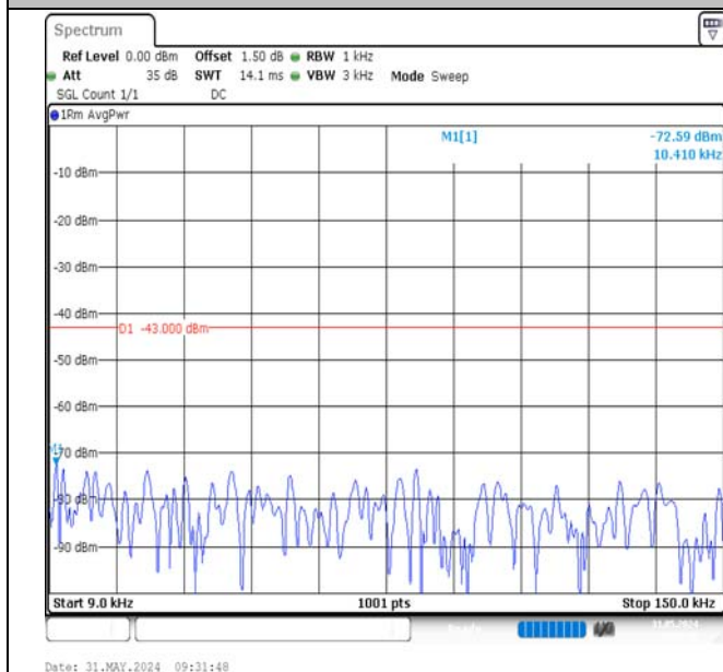
Band2-20MHz-16QAM-18900-1RB#0-0.009~0.15-PASS
