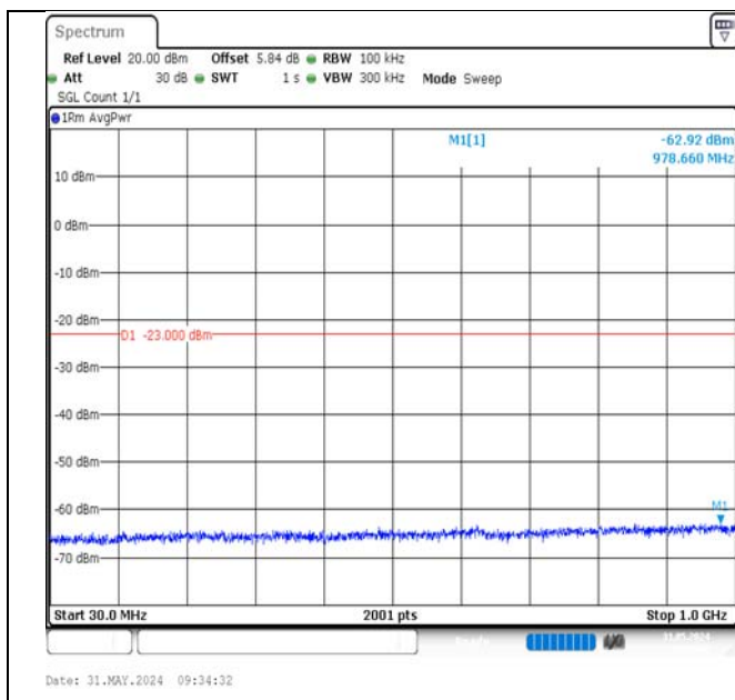
Band2-20MHz-QPSK-19100-1RB#99-30~1000-PASS
