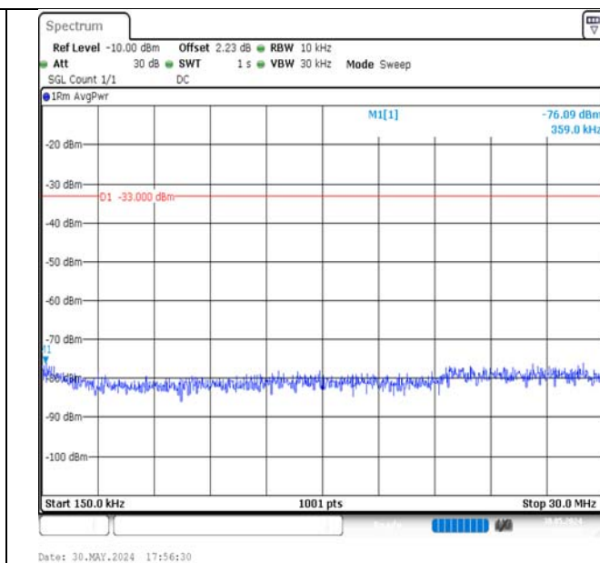
Band4-1.4MHz-QPSK-20175-6RB#0-0.15~30-PASS
