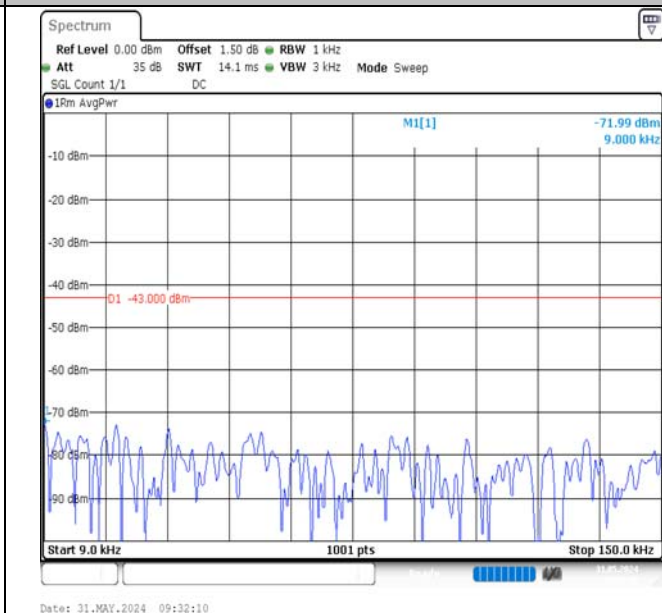
Band2-20MHz-QPSK-18900-1RB#99-0.009~0.15-PASS
