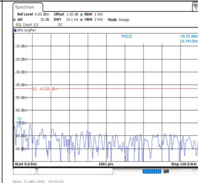
Band2-20MHz-16QAM-18900-100RB#0-0.009~0.15-PASS
