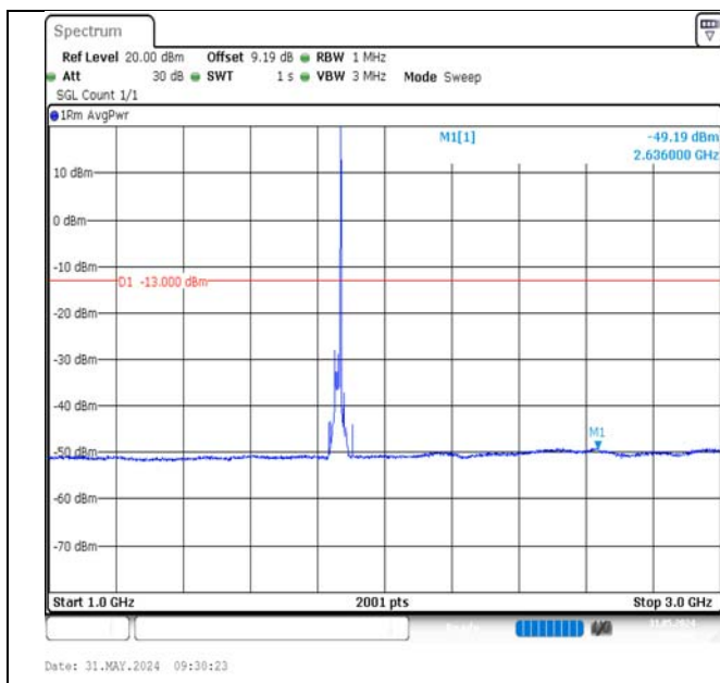
Band2-20MHz-16QAM-18700-1RB#99-1000~3000-PASS
