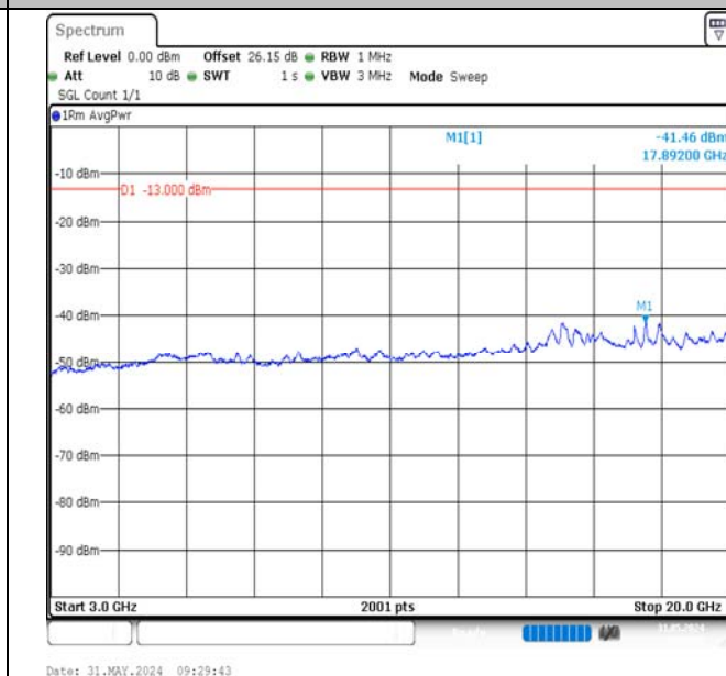
Band2-20MHz-16QAM-18700-1RB#0-3000~20000-PASS
