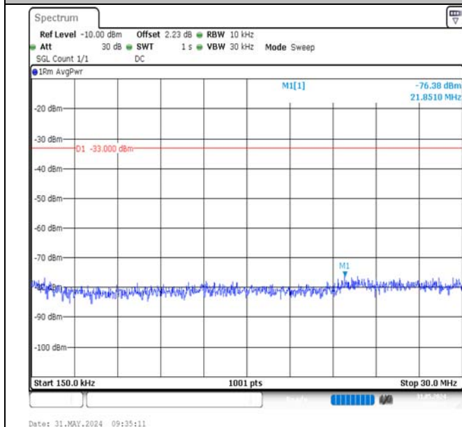
Band2-20MHz-QPSK-19100-100RB#0-0.15~30-PASS
