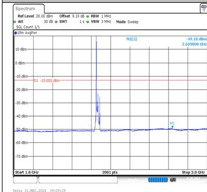
Band2-20MHz-16QAM-18700-1RB#0-1000~3000-PASS
