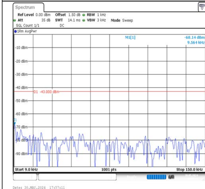
Band4-1.4MHz-QPSK-20393-1RB#0-0.009~0.15-PASS
