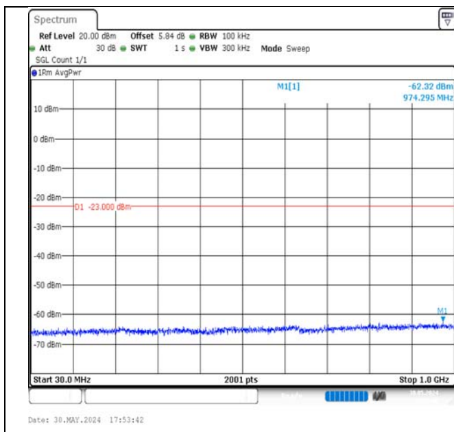
Band4-1.4MHz-QPSK-19957-1RB#5-30~1000-PASS
