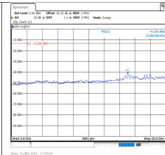
Band4-1.4MHz-QPSK-20175-1RB#5-3000~20000-PASS
