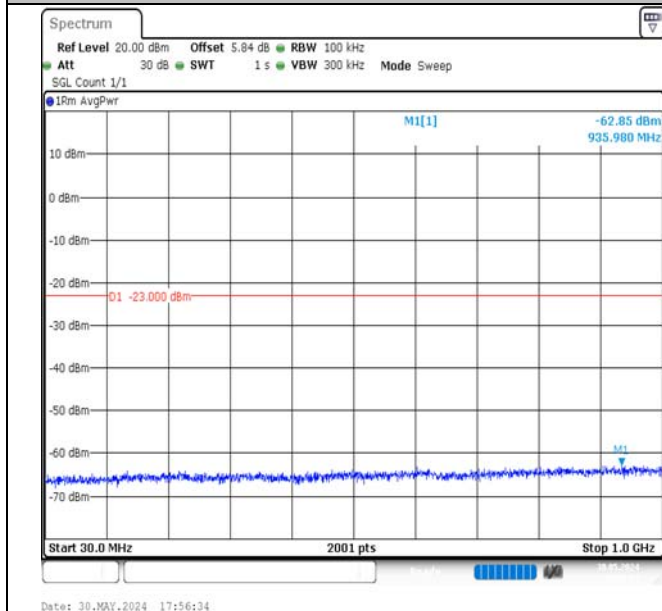
Band4-1.4MHz-QPSK-20175-6RB#0-30~1000-PASS
