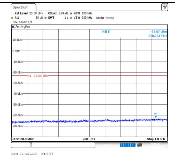
Band2-20MHz-16QAM-19100-1RB#99-30~1000-PASS
