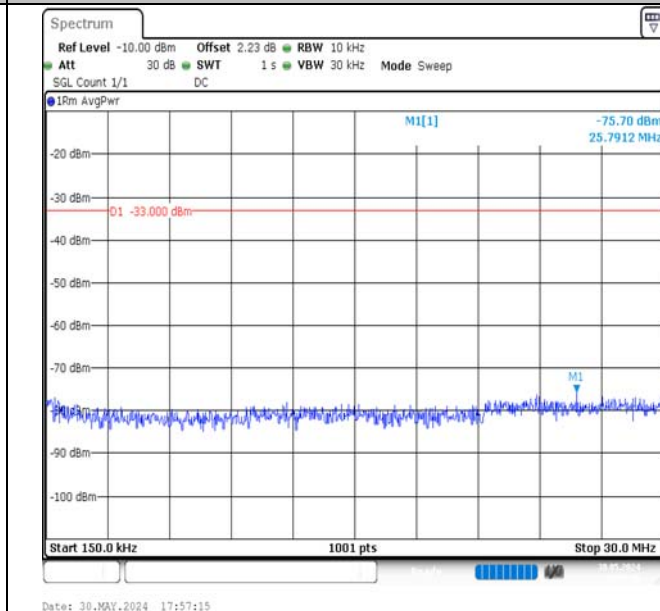
Band4-1.4MHz-QPSK-20393-1RB#0-0.15~30-PASS
