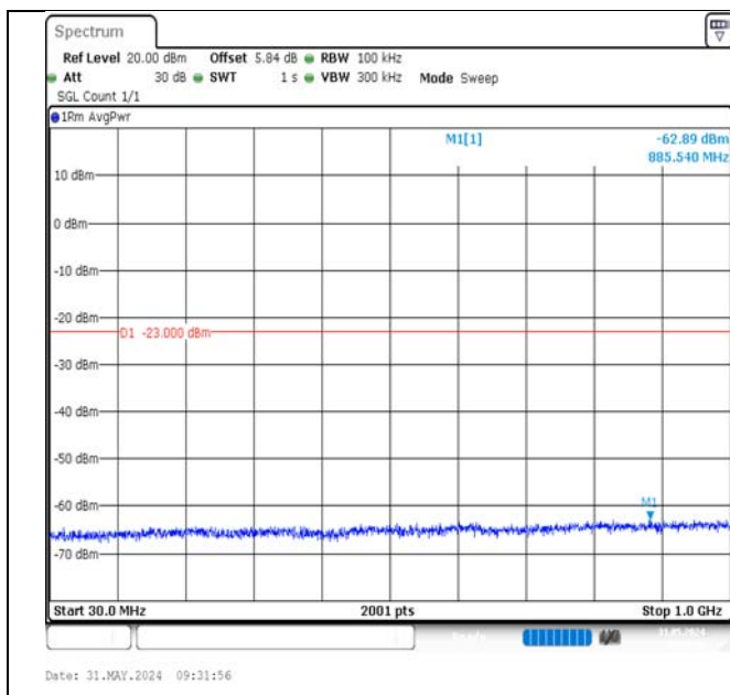
Band2-20MHz-16QAM-18900-1RB#0-30~1000-PASS
