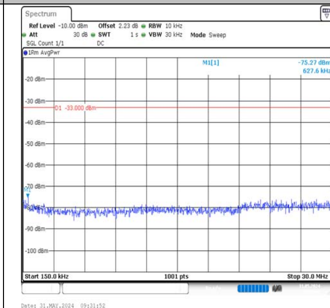
Band2-20MHz-16QAM-18900-1RB#0-0.15~30-PASS
