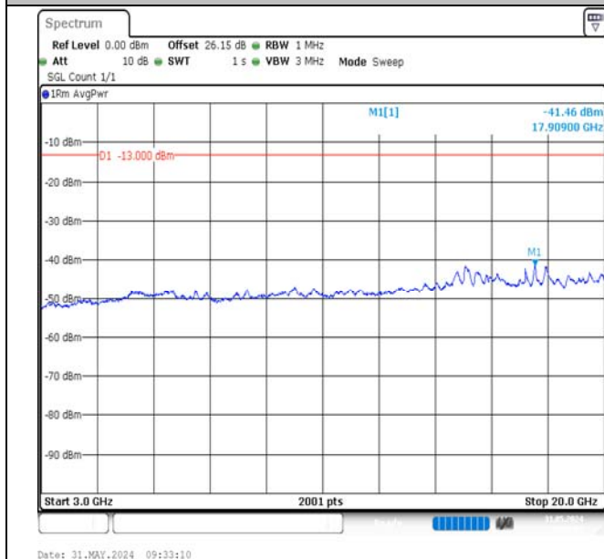
Band2-20MHz-QPSK-18900-100RB#0-3000~20000-PASS
