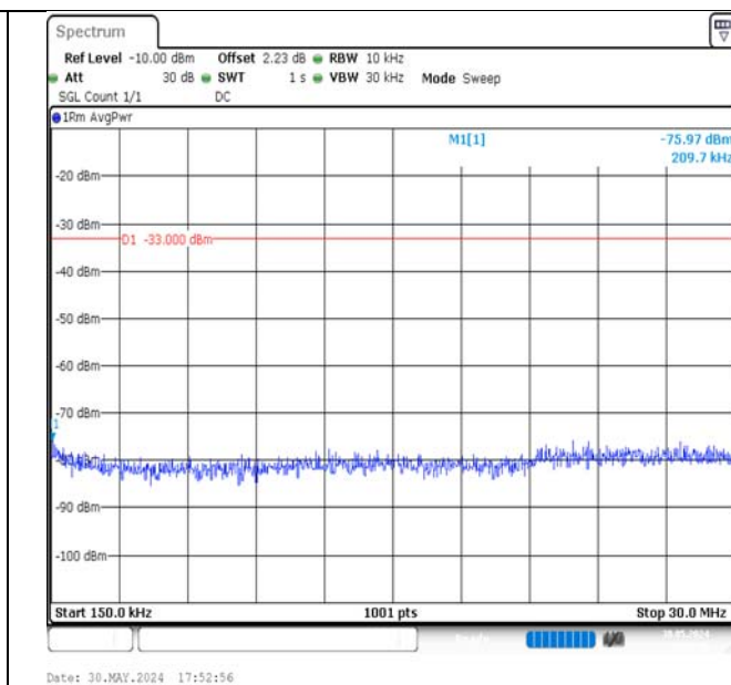
Band4-1.4MHz-QPSK-19957-1RB#0-0.15~30-PASS
