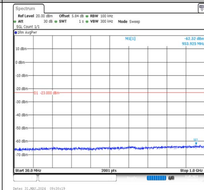
Band2-20MHz-16QAM-18700-1RB#99-30~1000-PASS
