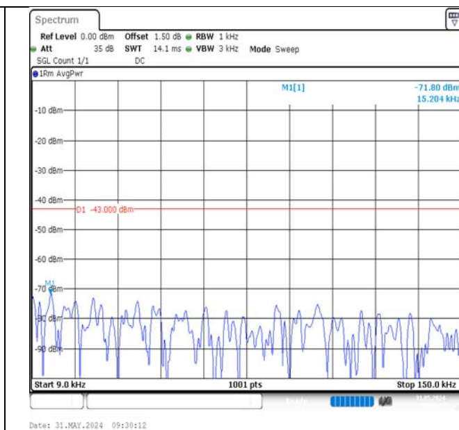
Band2-20MHz-16QAM-18700-1RB#99-0.009~0.15-PASS
