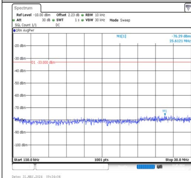
Band2-20MHz-16QAM-19100-1RB#0-0.15~30-PASS
