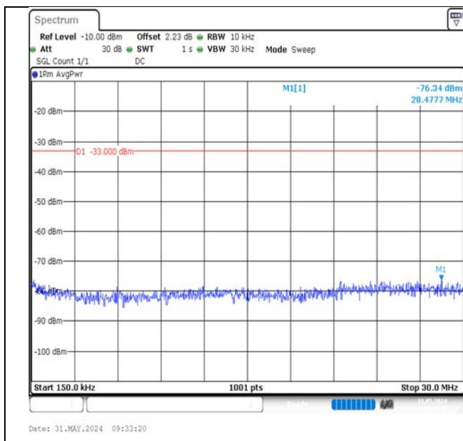
Band2-20MHz-16QAM-18900-100RB#0-0.15~30-PASS
