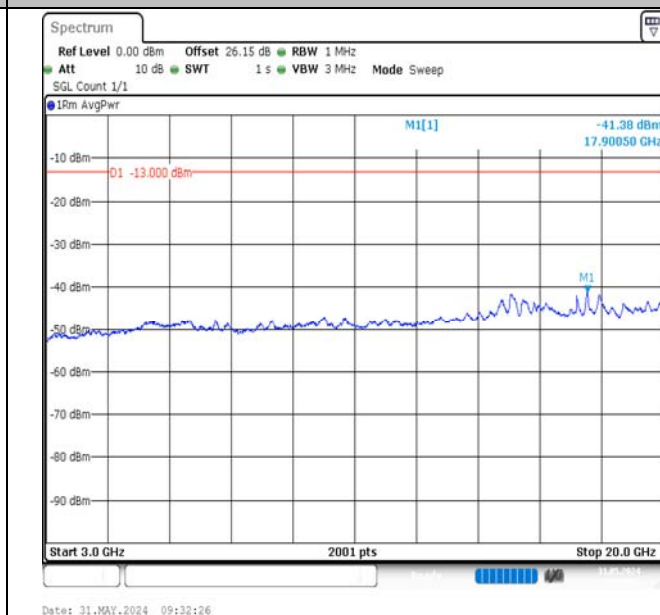
Band2-20MHz-QPSK-18900-1RB#99-3000~20000-PASS
