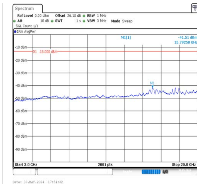
Band4-1.4MHz-QPSK-19957-6RB#0-3000~20000-PASS
