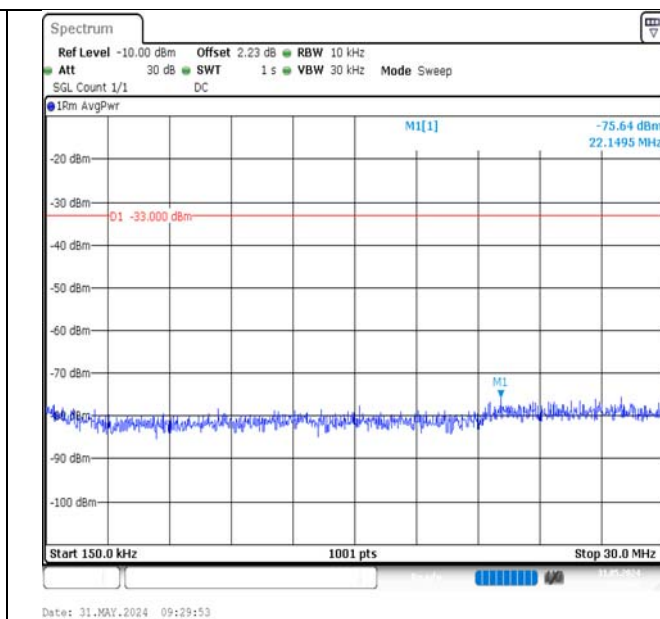
Band2-20MHz-QPSK-18700-1RB#99-0.15~30-PASS
