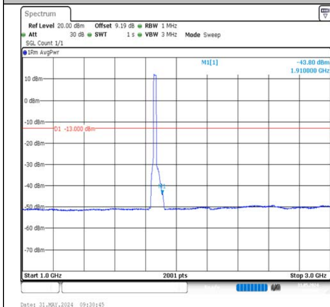
Band2-20MHz-QPSK-18700-100RB#0-1000~3000-PASS
