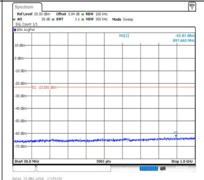
Band4-1.4MHz-QPSK-20175-1RB#5-30~1000-PASS
