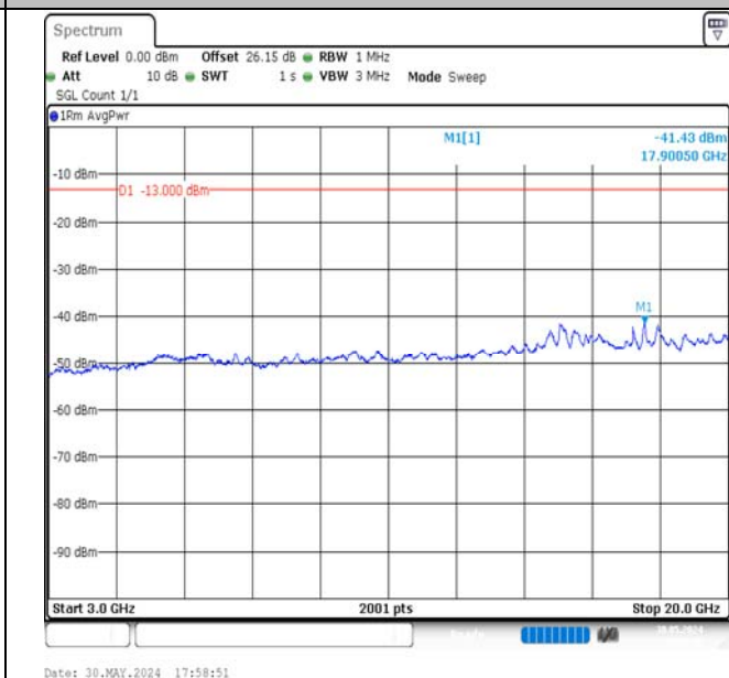
Band4-1.4MHz-QPSK-20393-6RB#0-3000~20000-PASS
