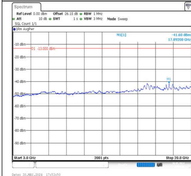
Band4-1.4MHz-QPSK-19957-1RB#5-3000~20000-PASS
