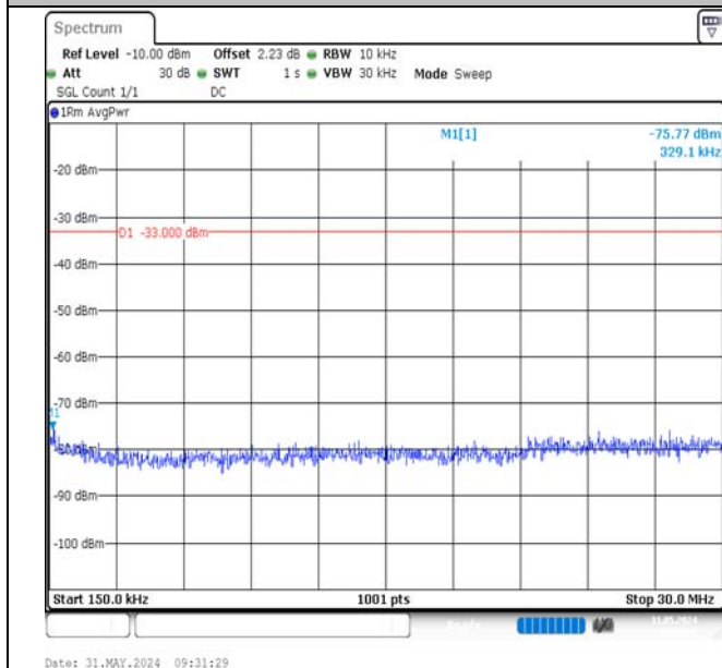
Band2-20MHz-QPSK-18900-1RB#0-0.15~30-PASS
