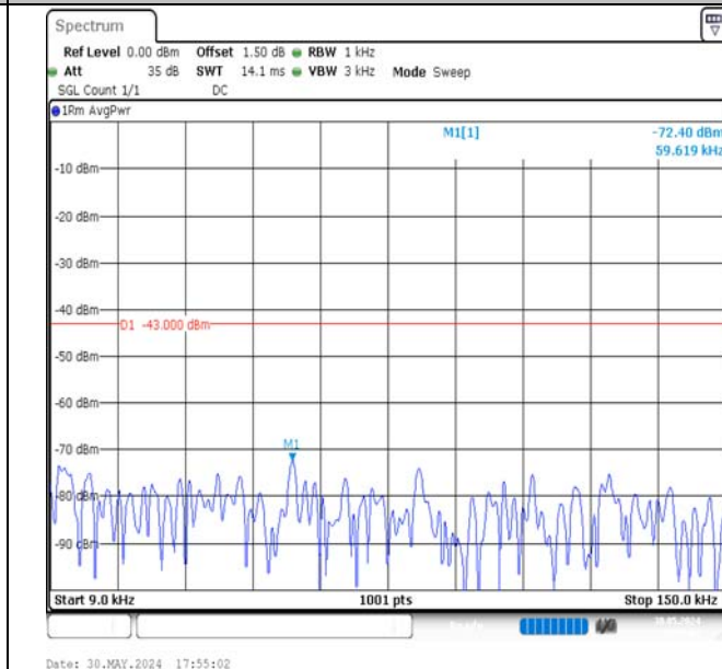
Band4-1.4MHz-QPSK-20175-1RB#0-0.009~0.15-PASS
