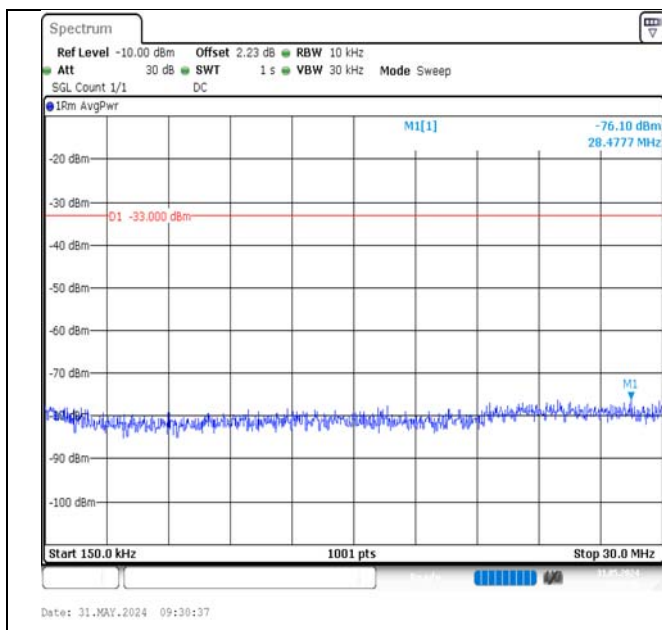
Band2-20MHz-QPSK-18700-100RB#0-0.15~30-PASS
