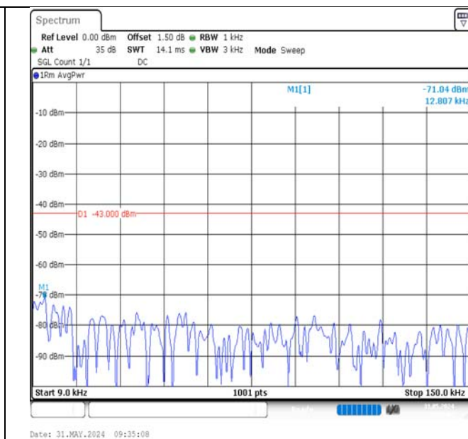
Band2-20MHz-QPSK-19100-100RB#0-0.009~0.15-PASS
