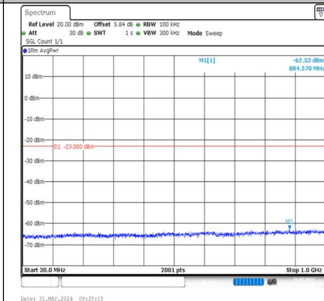
Band2-20MHz-QPSK-19100-100RB#0-30~1000-PASS
