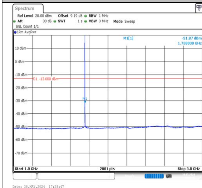
Band4-1.4MHz-QPSK-20393-6RB#0-1000~3000-PASS
