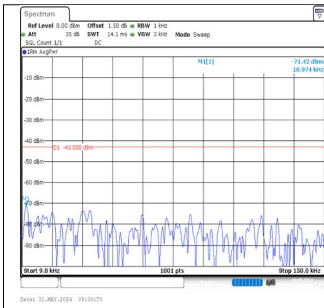
Band2-20MHz-16QAM-18700-100RB#0-0.009~0.15-PASS
