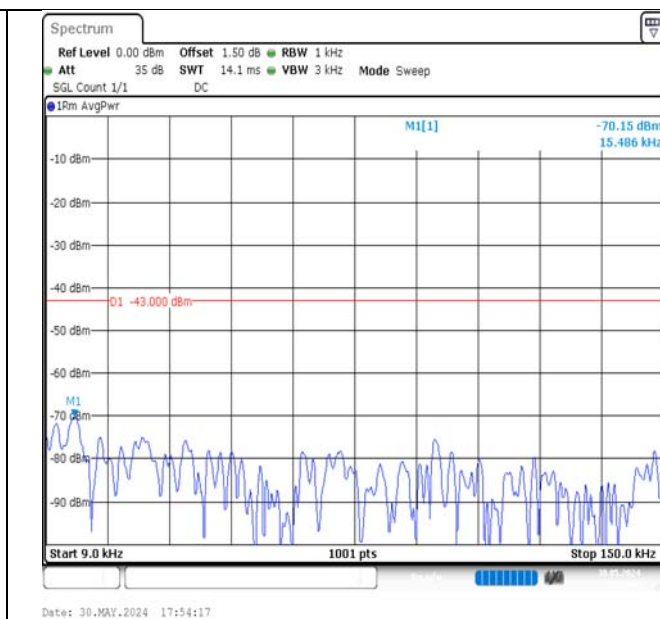
Band4-1.4MHz-QPSK-19957-6RB#0-0.009~0.15-PASS
