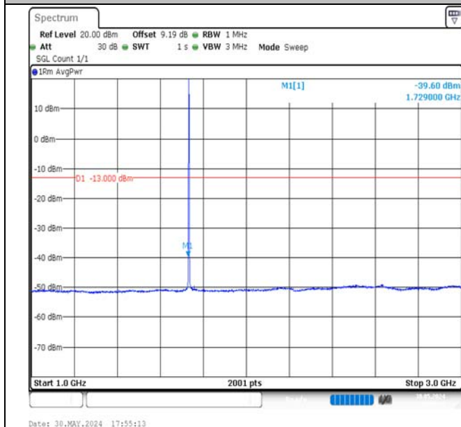
Band4-1.4MHz-QPSK-20175-1RB#0-1000~3000-PASS
