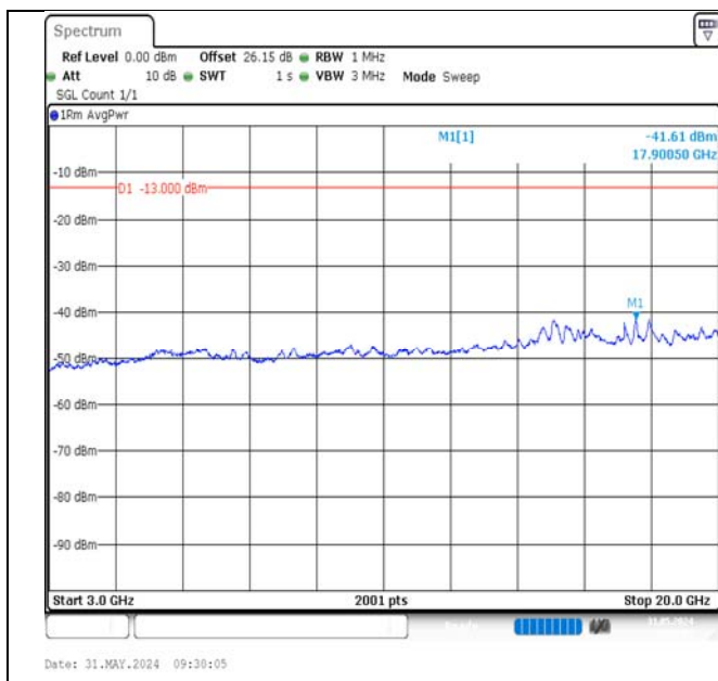
Band2-20MHz-QPSK-18700-1RB#99-3000~20000-PASS
