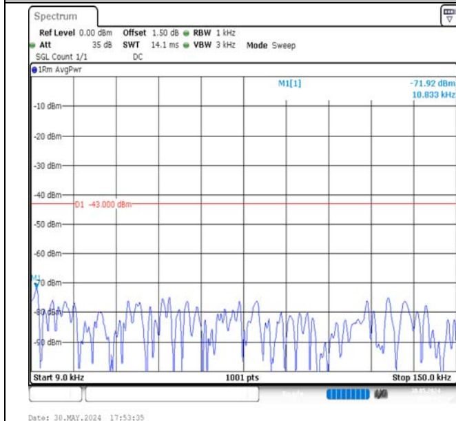
Band4-1.4MHz-QPSK-19957-1RB#5-0.009~0.15-PASS
