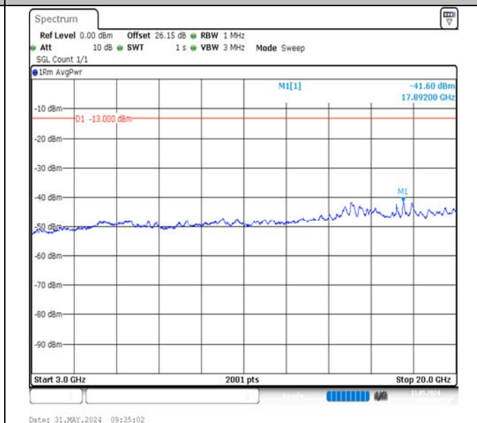
Band2-20MHz-16QAM-19100-1RB#99-3000~20000-PASS
