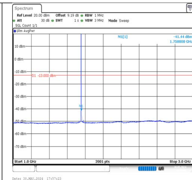
Band4-1.4MHz-QPSK-20393-1RB#0-1000~3000-PASS
