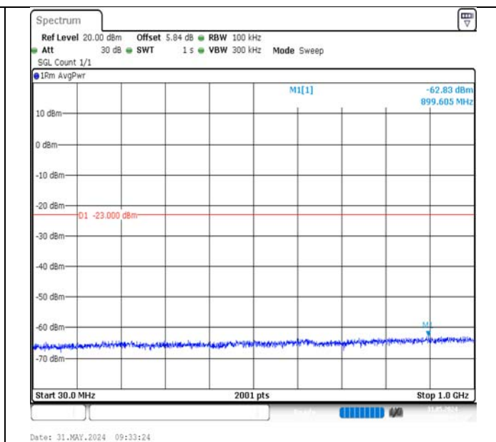
Band2-20MHz-16QAM-18900-100RB#0-30~1000-PASS
