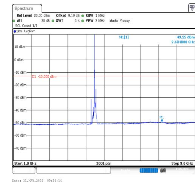
Band2-20MHz-16QAM-19100-1RB#0-1000~3000-PASS
