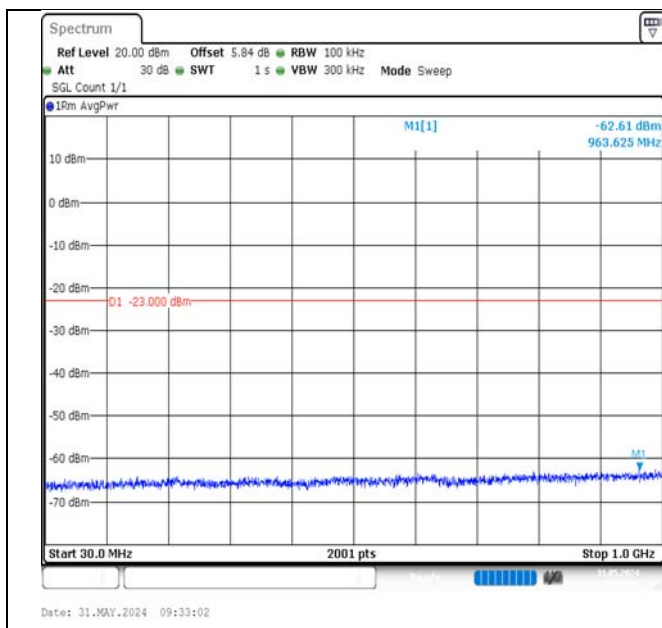
Band2-20MHz-QPSK-18900-100RB#0-30~1000-PASS
