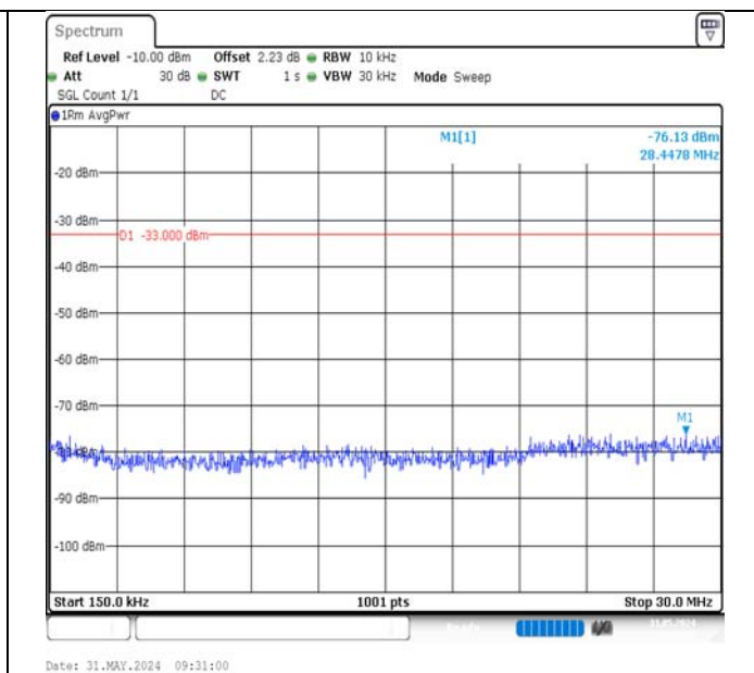
Band2-20MHz-16QAM-18700-100RB#0-0.15~30-PASS
