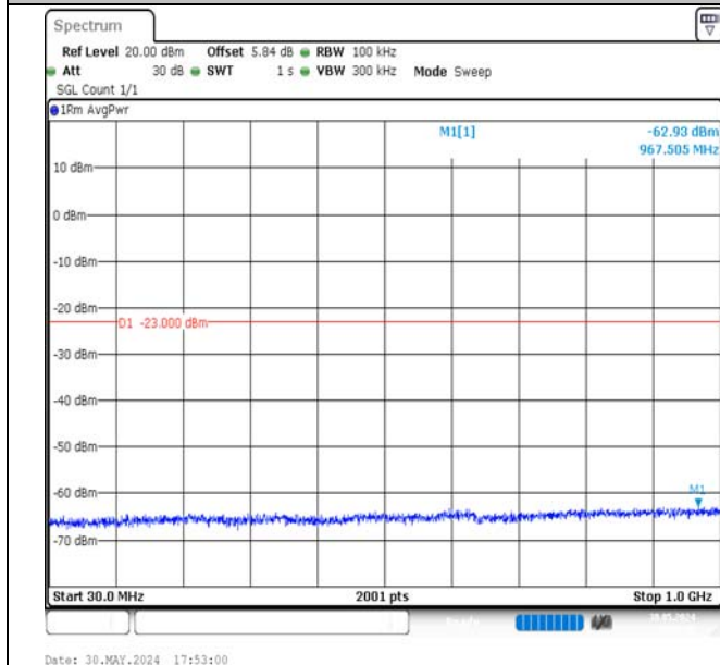
Band4-1.4MHz-QPSK-19957-1RB#0-30~1000-PASS
