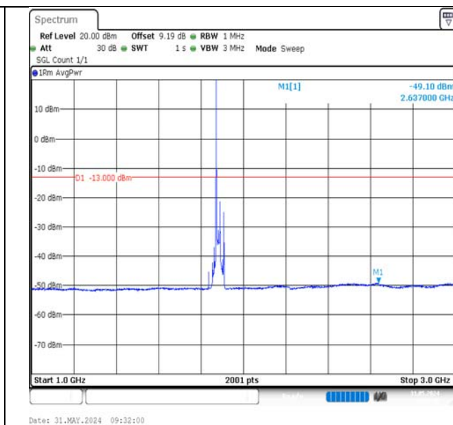
Band2-20MHz-16QAM-18900-1RB#0-1000~3000-PASS
