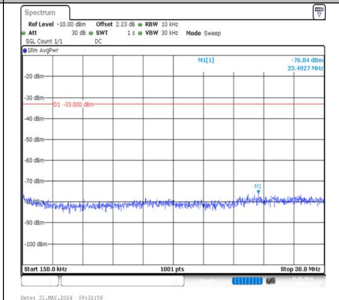
Band2-20MHz-QPSK-18900-100RB#0-0.15~30-PASS
