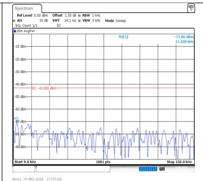
Band4-1.4MHz-QPSK-20175-1RB#5-0.009~0.15-PASS
