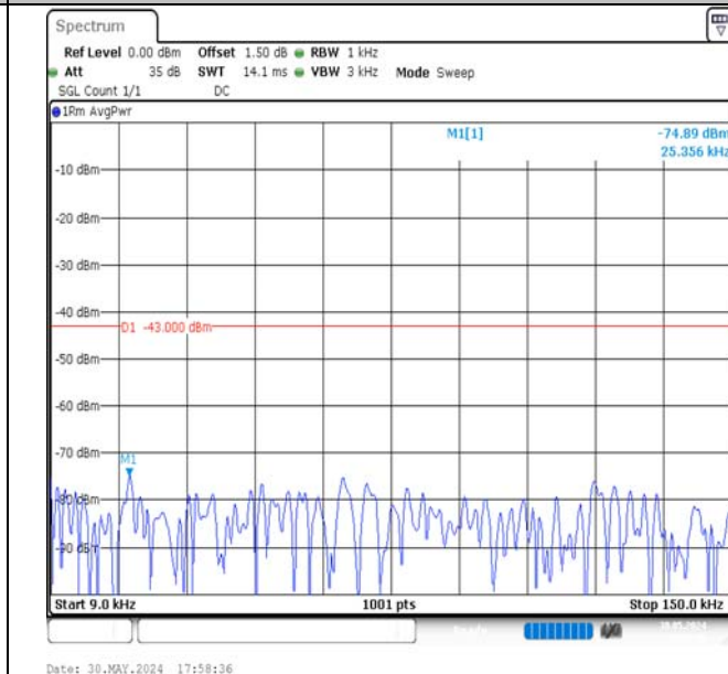
Band4-1.4MHz-QPSK-20393-6RB#0-0.009~0.15-PASS
