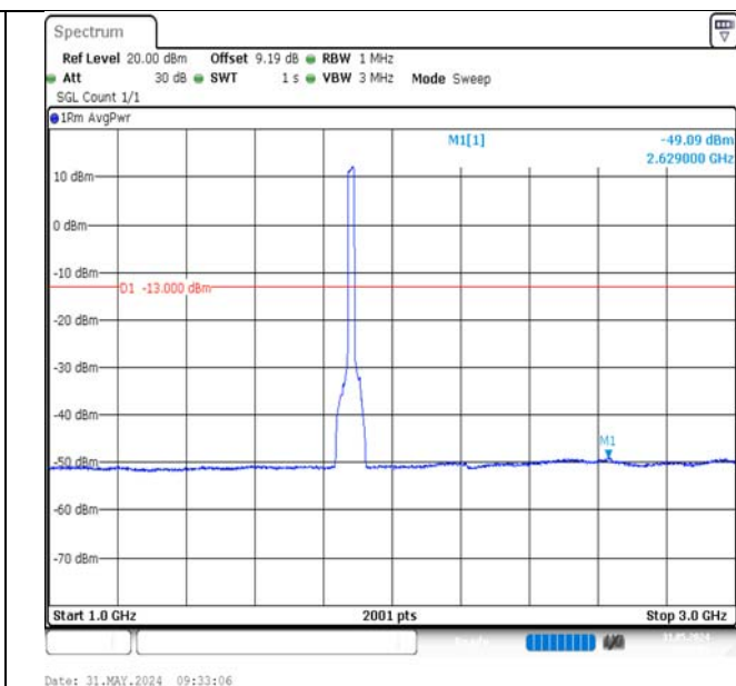
Band2-20MHz-QPSK-18900-100RB#0-1000~3000-PASS
