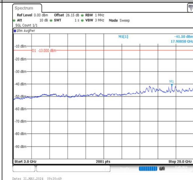
Band2-20MHz-QPSK-18700-100RB#0-3000~20000-PASS
