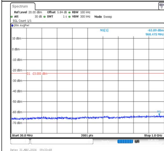
Band2-20MHz-QPSK-19100-1RB#0-30~1000-PASS
