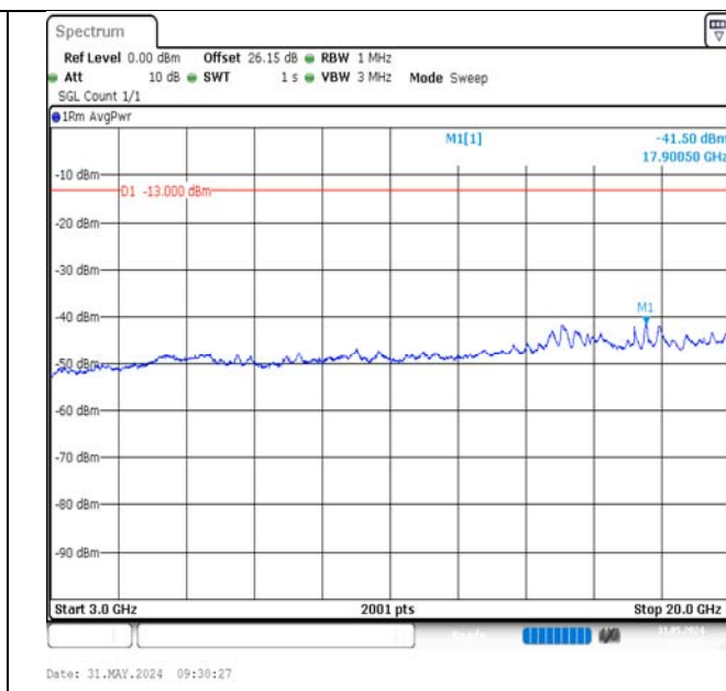
Band2-20MHz-16QAM-18700-1RB#99-3000~20000-PASS
