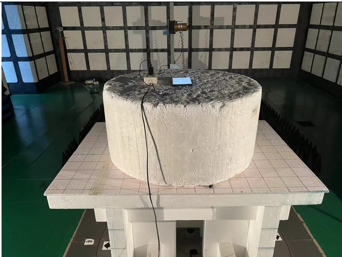
Above 1GHz
