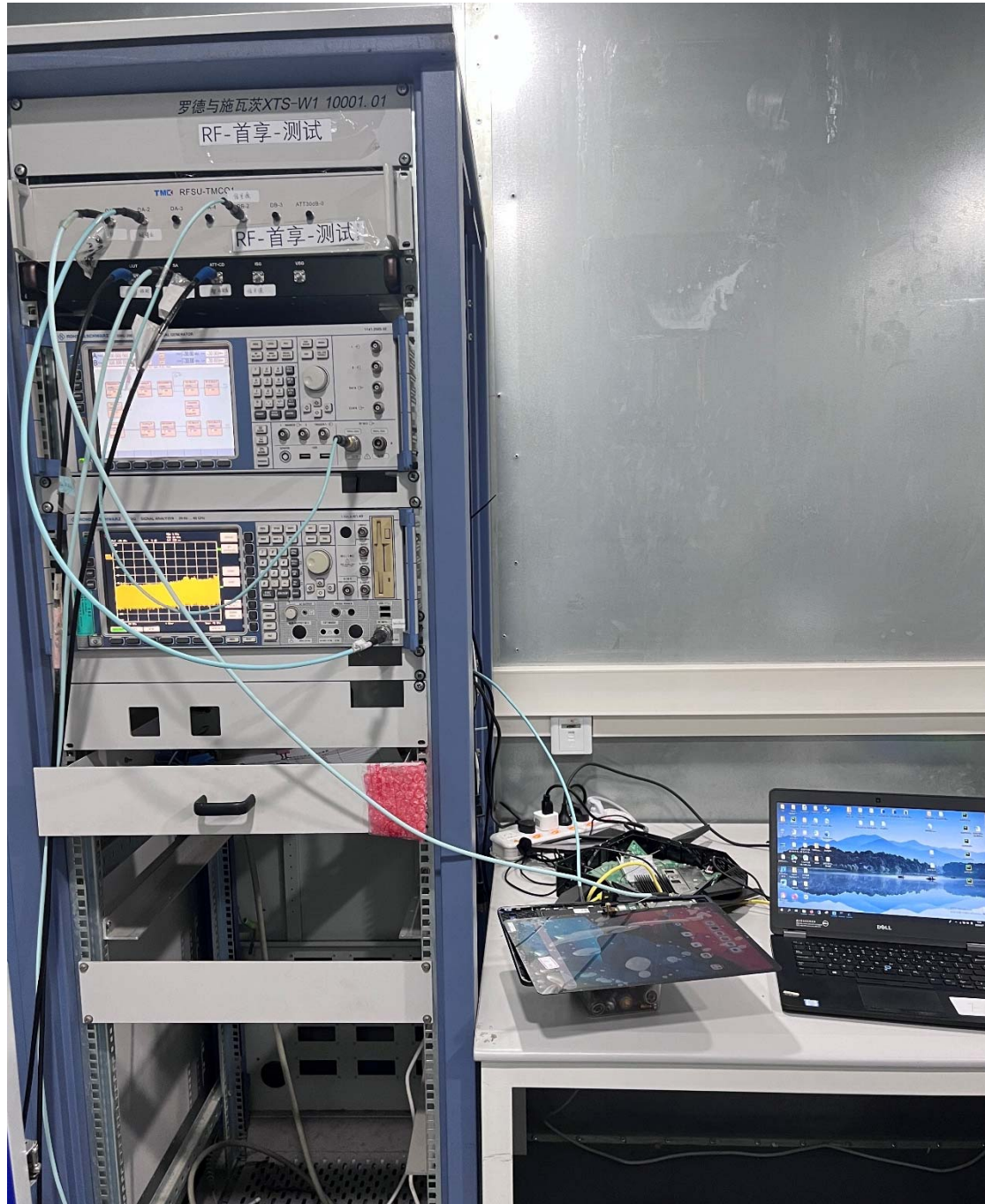
DFS test setup photo
