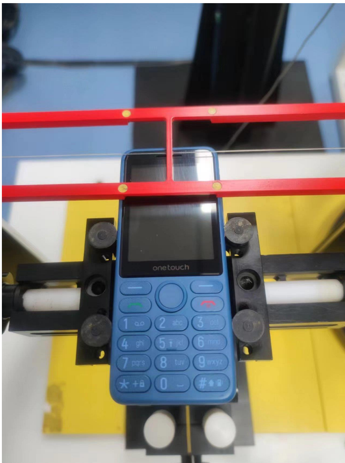
Picture 2: EUT Positioning for RF/T-coil
