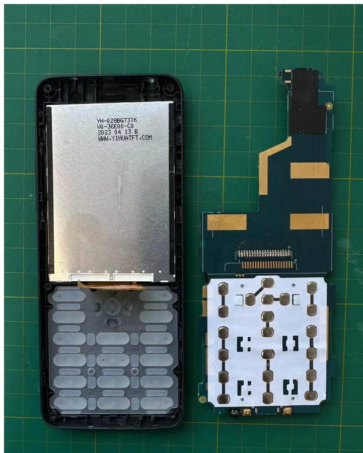
T312E mobile phone Disassembly
