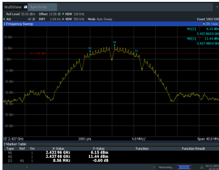
Fig.A.4.2 DTS Bandwidth (802.11b, Ch 6)
