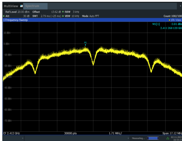
16:55:21 02.11.2023 Fig.A.3.1 Power Spectral Density(802.11b,Ch1)
