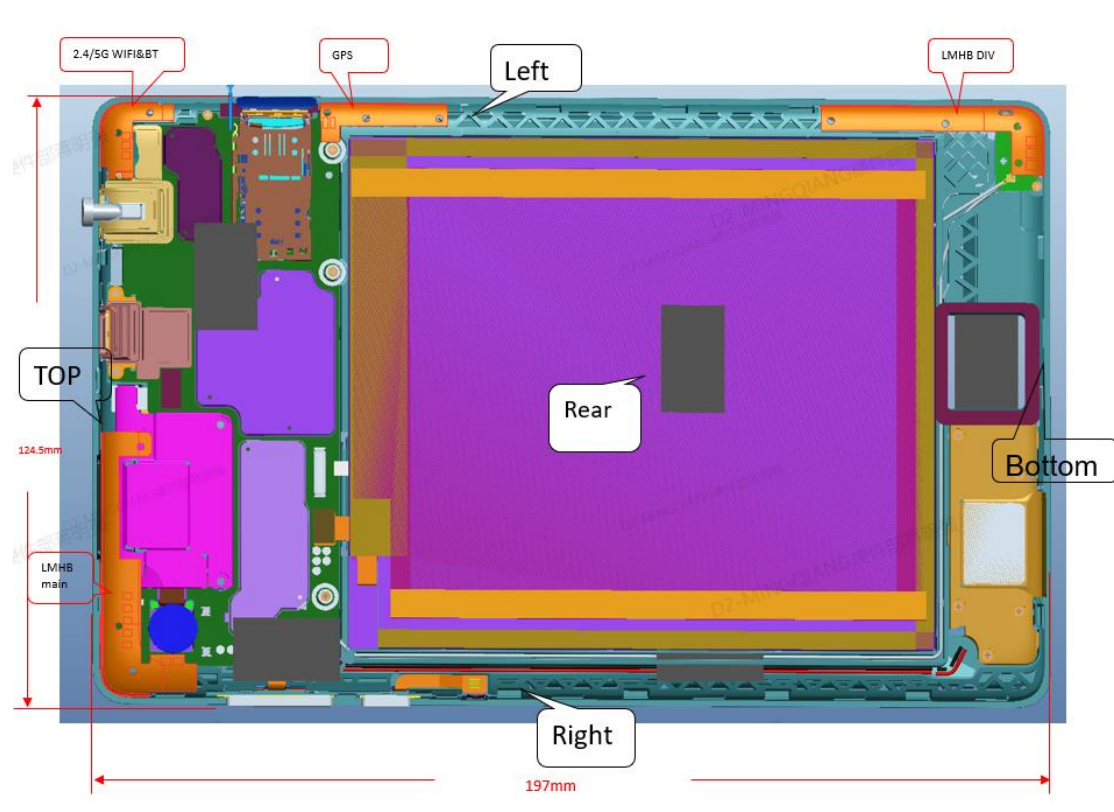
Picture 11 Antenna location
