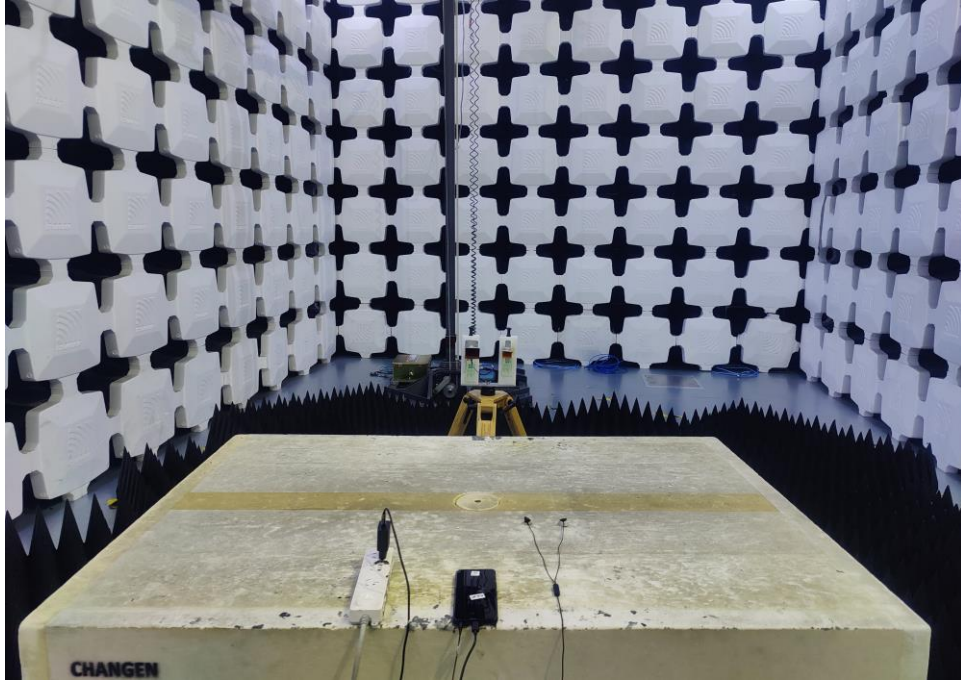
3. Radiated Emissions (Part 15B, Video Player, 18GHz-26.5GHz)
