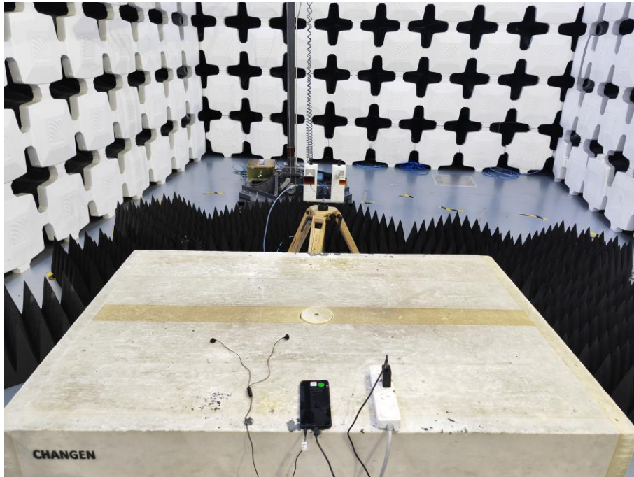
7. Radiated Emissions (Part 15B, Camera, 18GHz-26.5GHz)
