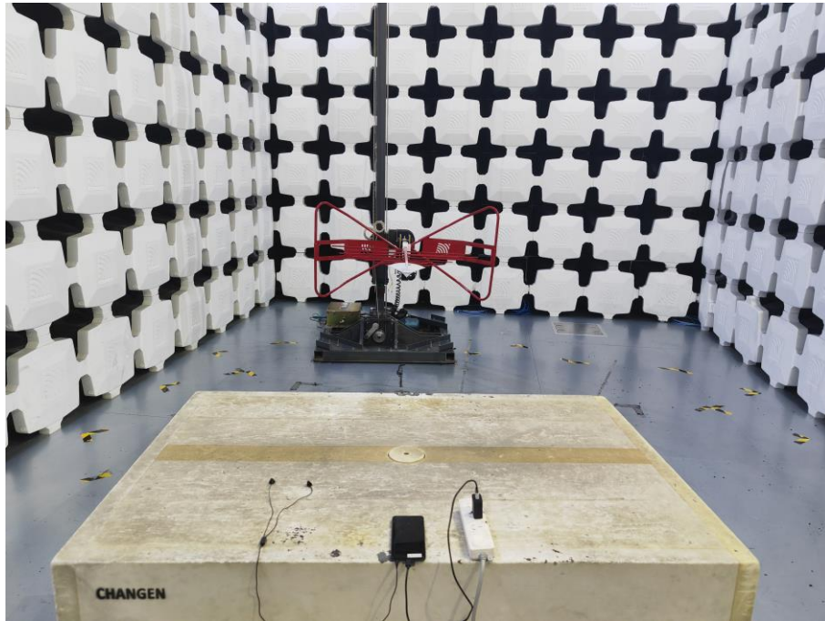
5. Radiated Emissions (Part 15B, Camera, 30MHz-1GHz)
