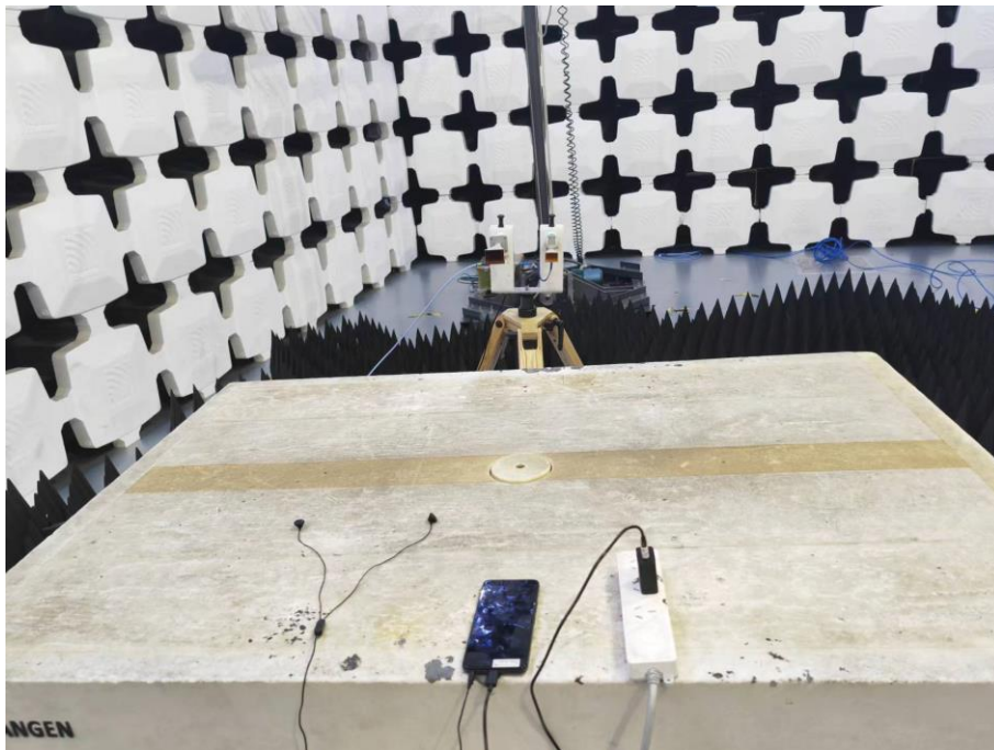
8. Radiated Emissions (Part 15B, Camera, 26.5GHz-40GHz)
