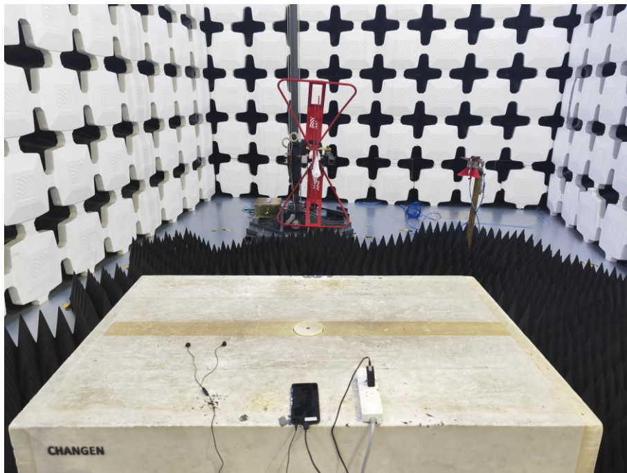
6. Radiated Emissions (Part 15B, Camera, 1GHz-18GHz)
