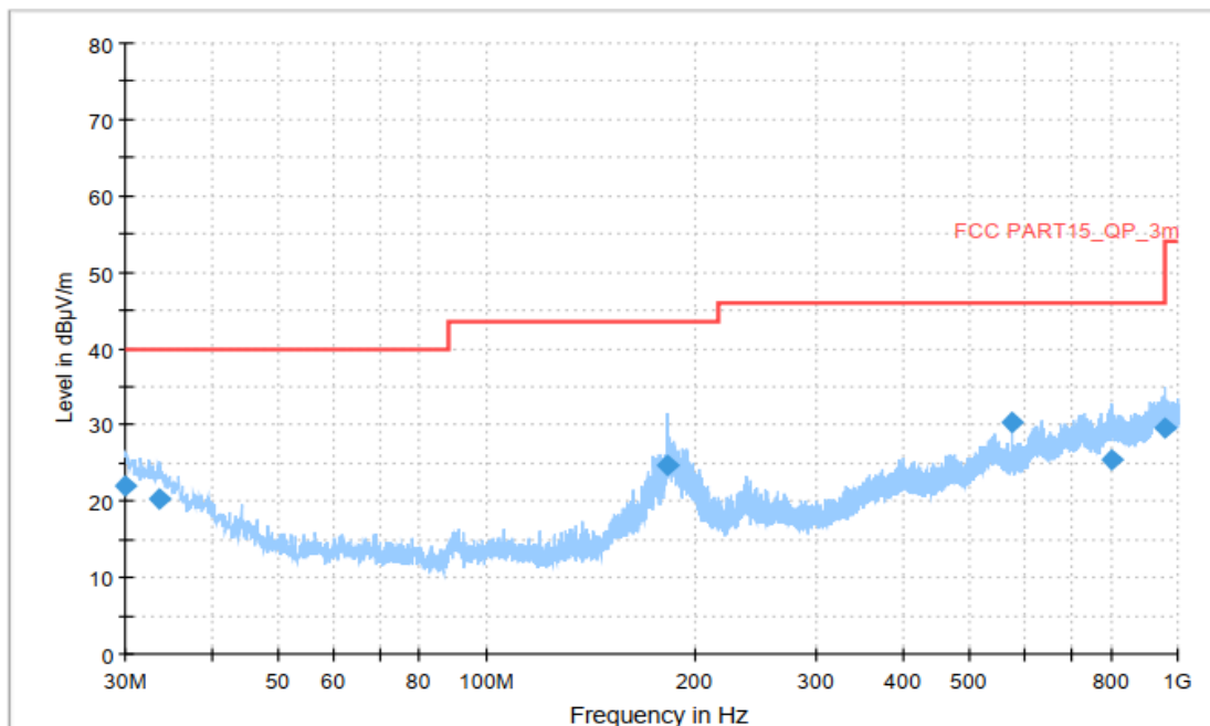
Figure A.1.17. Radiated Emission (Data Transfer: TF Card TO PC, 30MHz to 1GHz) Final_Results
