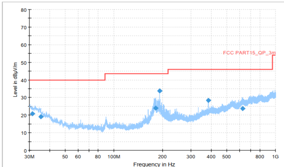
Figure A.1.9. Radiated Emission (Data Transfer: EUT TO PC, 30MHz to 1GHz)
