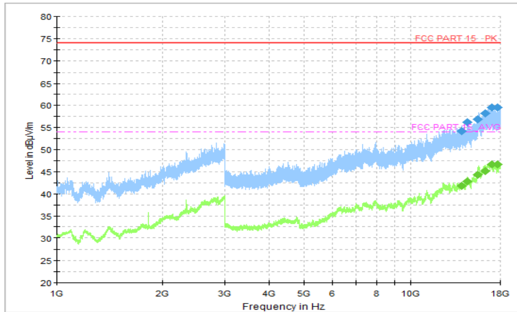
Figure A.1.14. Radiated Emission (Data Transfer: PC TO TF Card, 1GHz to 18GHz) Final_Results_PK
