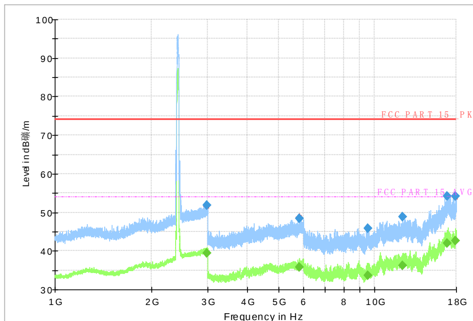
Fig.60 Radiated Spurious Emission (802.11n HT40, CH3, 1GHz~18GHz)
