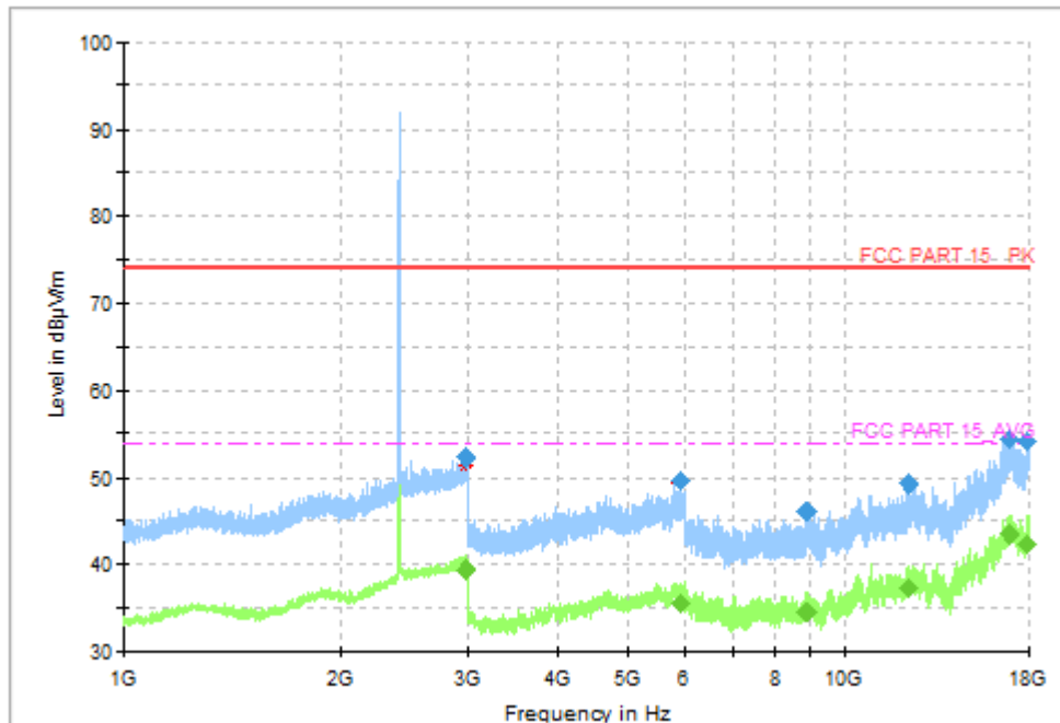
Fig.51 Radiated Spurious Emission (802.11g, CH6, 1GHz-18GHz)
