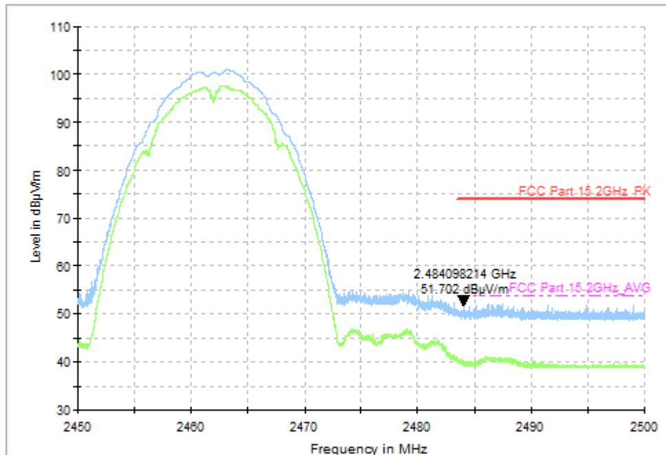
Fig.49 Radiated Restricted Band (802.11b, CH11, 2.45GHz~2.5GHz)
