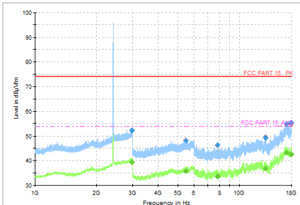
Fig.50 Radiated Spurious Emission (802.11g, CH1, 1GHz~18GHz)
