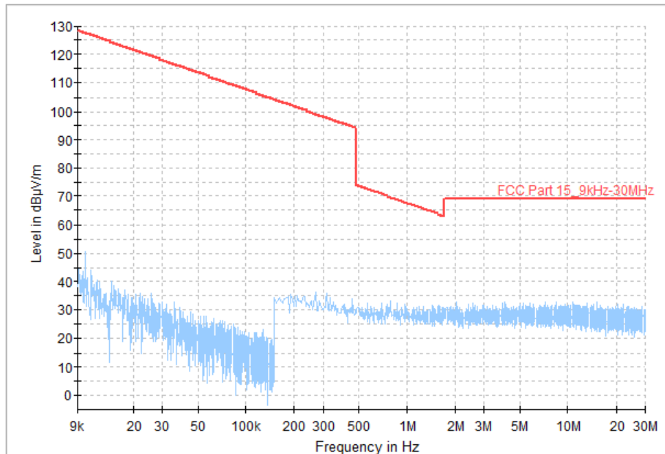
Fig.65 Radiated Spurious Emission (All Channels, 9KHz-30MHz)
