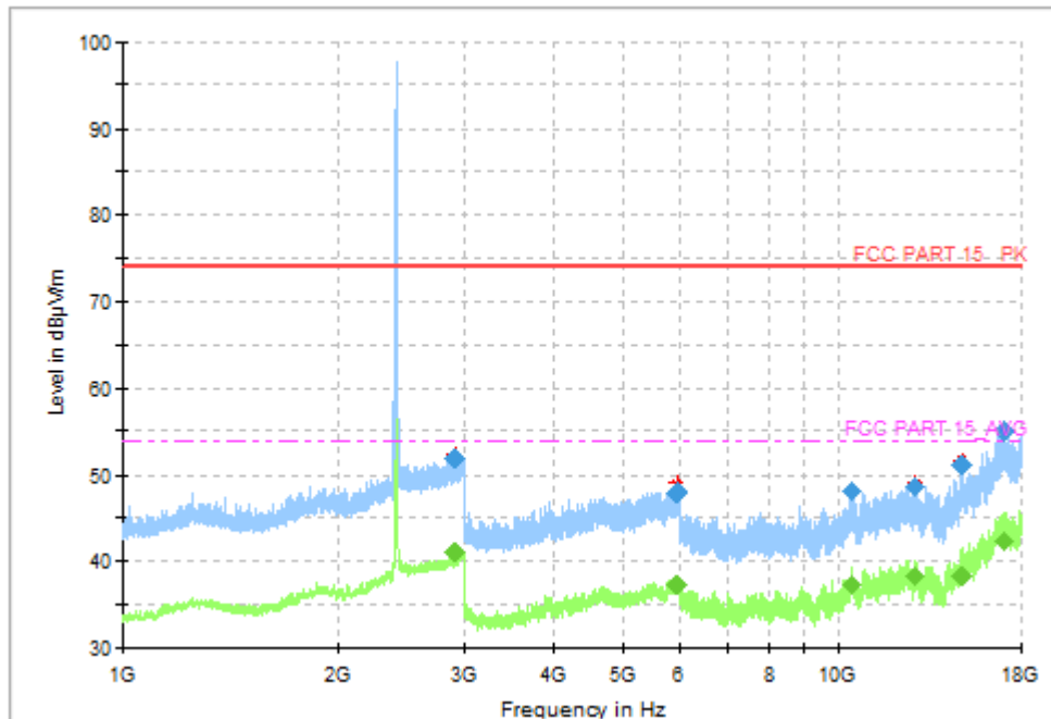
Fig.55 Radiated Spurious Emission (802.11n HT20, CH1, 1GHz-18GHz)
