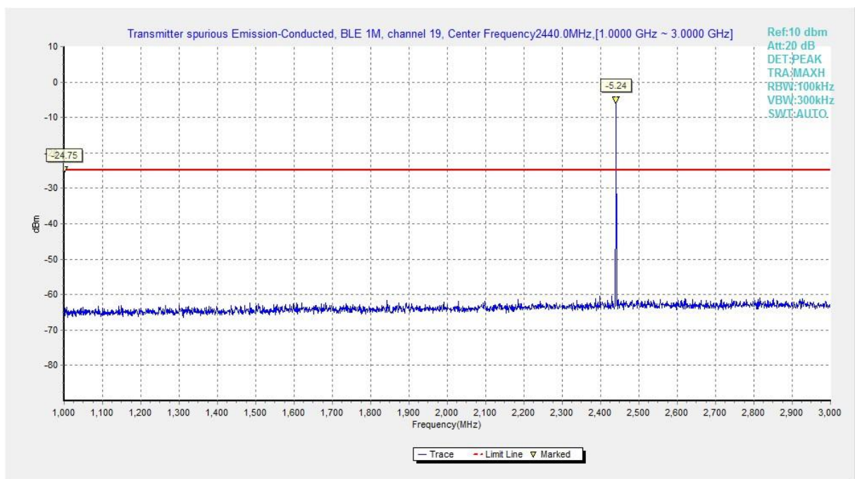
Fig.11 Conducted Spurious Emission (Ch19, 1GHz-3GHz), LE 1M
