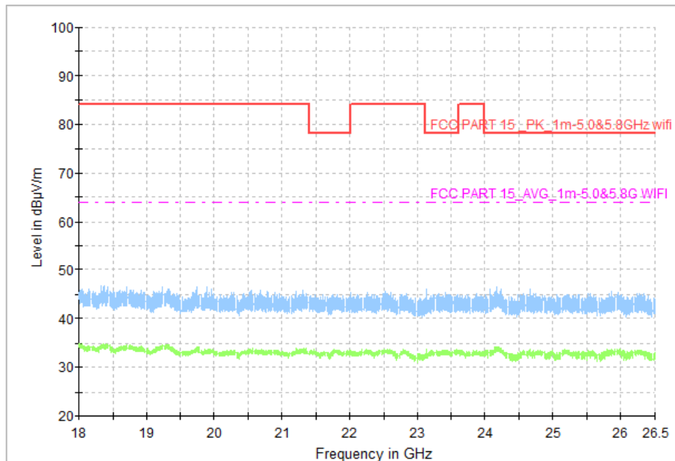
Fig.21 Radiated Spurious Emission (Ch19, 18GHz - 26.5GHz), 1M
