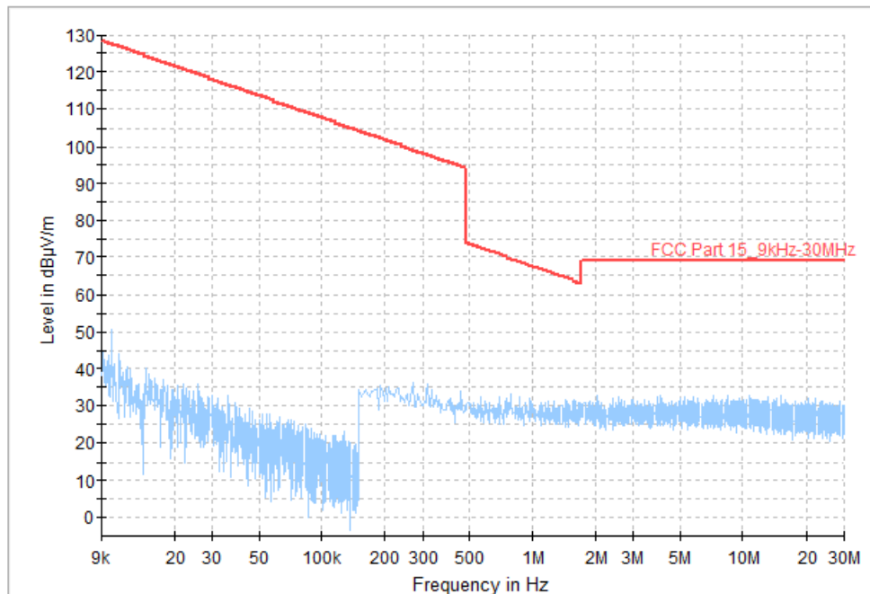
Fig.18 Radiated Spurious Emission (Ch19, 9kHz - 30MHz), 1M
