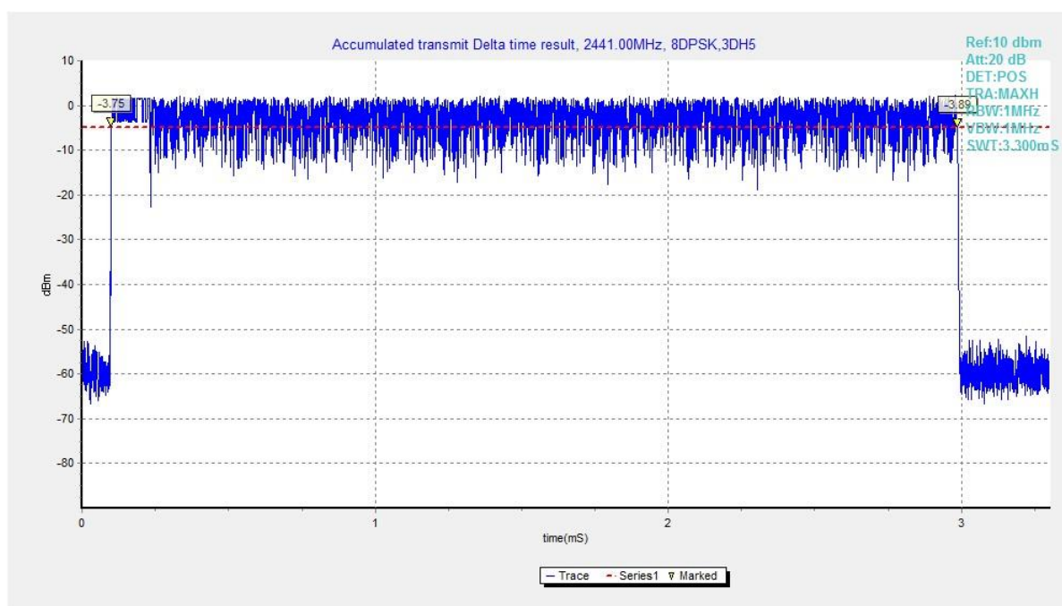
Fig. 64 Time of Occupancy(Dwell Time) (8DPSK, Ch39)
