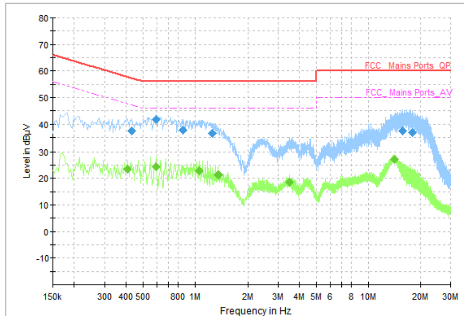
Fig. 75 AC Powerline Conducted Emission (Traffic, AE3, 120V)
