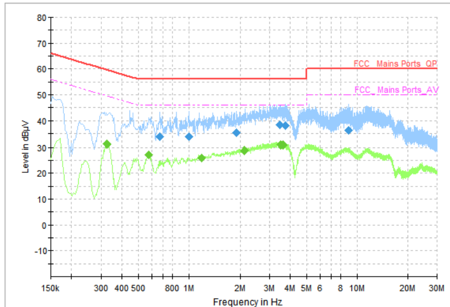
Fig. 76 AC Power line Conducted Emission (Idle, AE3, 120V)
