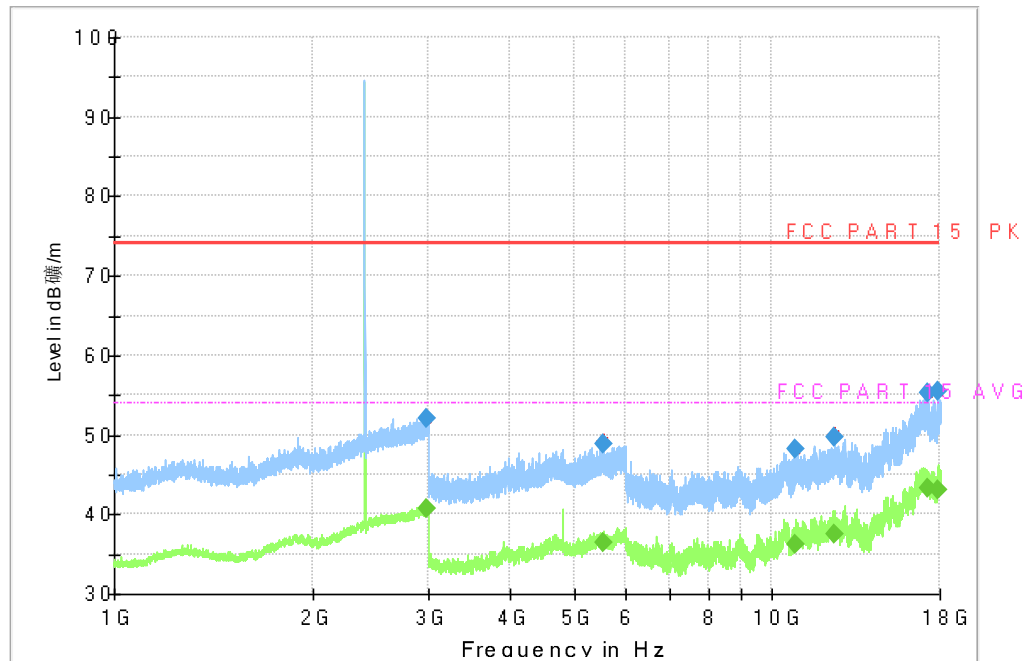
Fig. 33 Radiated Spurious Emission (GFSK, Ch0, 1GHz ~ 18GHz)
