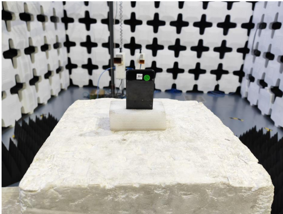
16. Radiated Emissions (Part 22/24/27, 26.5GHz-40GHz)
