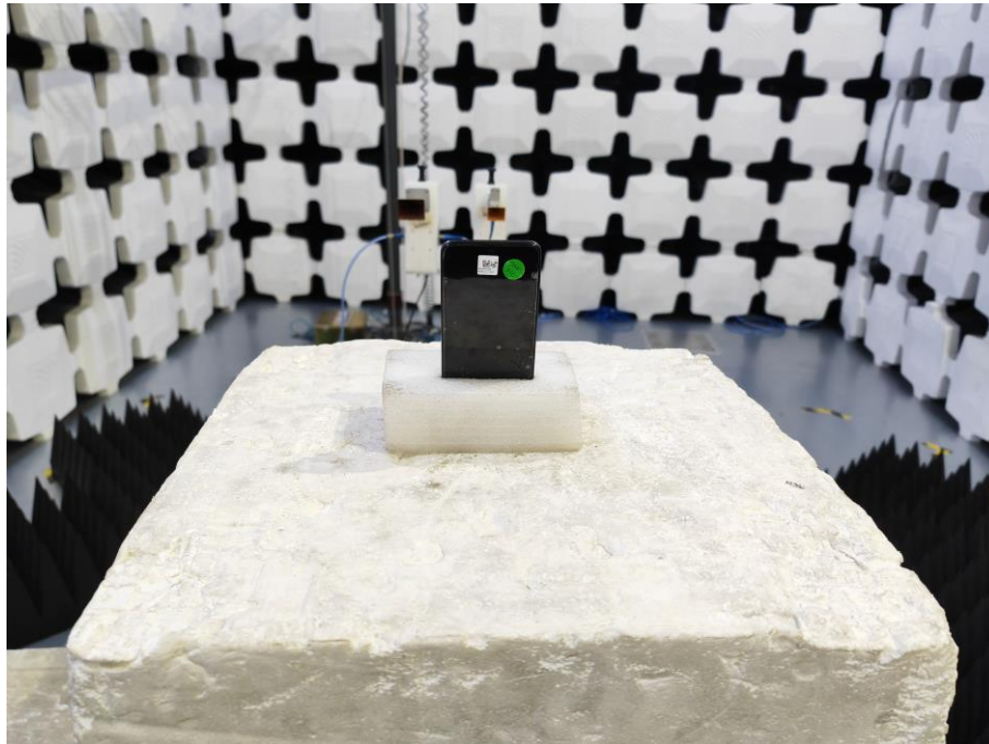
13. Radiated Emissions (Part 15C&Part 15E, 26.5GHz -40GHz)
