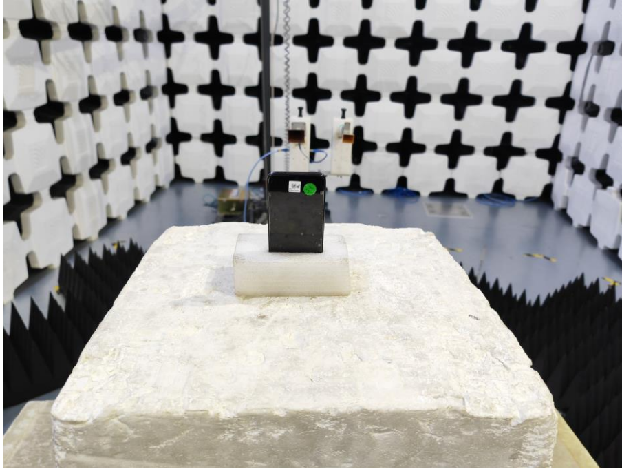
15. Radiated Emissions (Part 22/24/27, 18GHz-26.5GHz)
