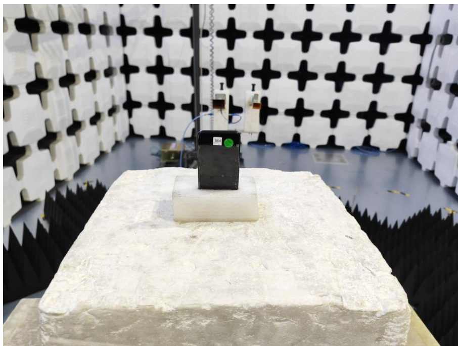
12. Radiated Emissions (Part 15C&Part 15E, 18GHz -26.5GHz)
