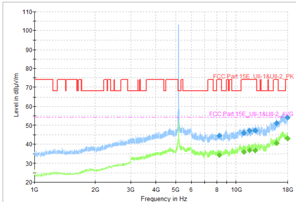
Fig. 65 Transmitter Spurious Emission (802.11a, CH36 5180MHz)
