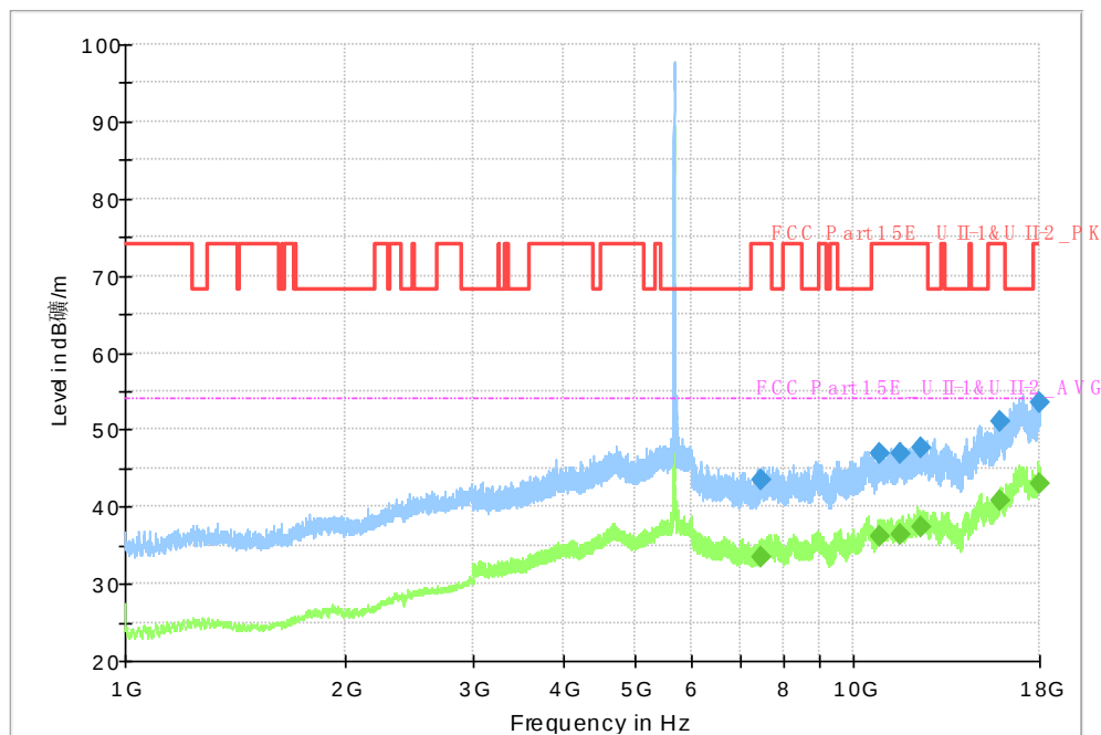
Fig. 82 Transmitter Spurious Emission (802.11n-HT40, CH134 5670MHz)
