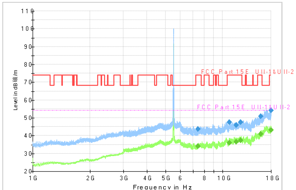
Fig. 81 Transmitter Spurious Emission (802.11n-HT40, CH102 5510MHz)
