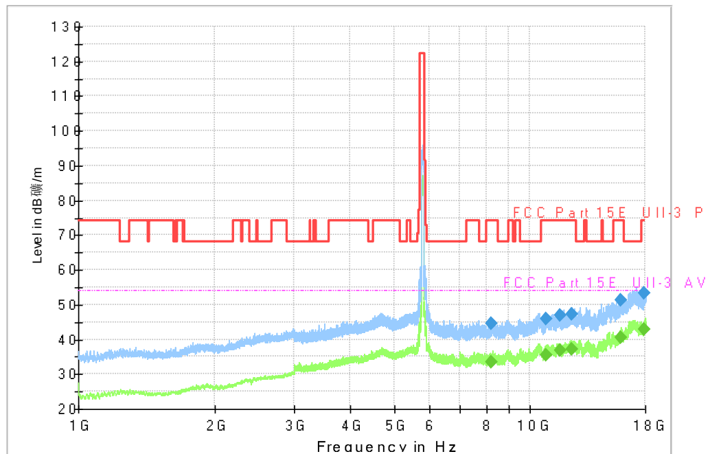
Fig. 88 Transmitter Spurious Emission (802.11ac-VHT80, CH155 5775MHz)
