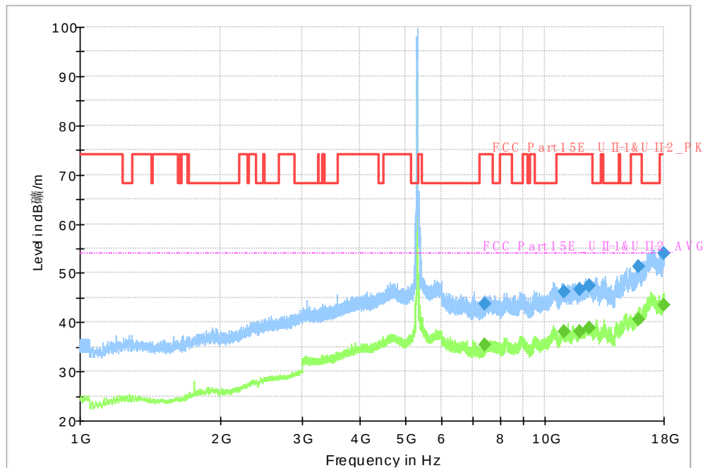
Fig. 80 Transmitter Spurious Emission (802.11n-HT40, CH62 5310MHz)
