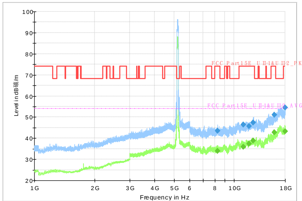
Fig. 85 Transmitter Spurious Emission (802.11ac-VHT80, CH42 5210MHz)
