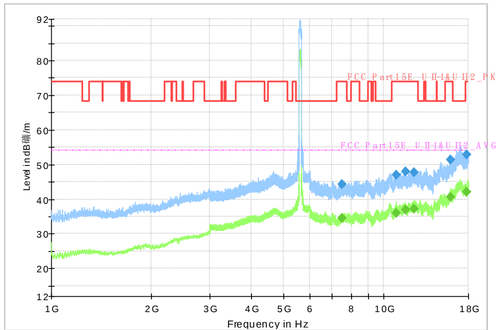
Fig. 87 Transmitter Spurious Emission (802.11ac-VHT80, CH122 5610MHz)
