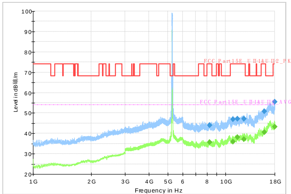
Fig. 79 Transmitter Spurious Emission (802.11n-HT40, CH54 5270MHz)
