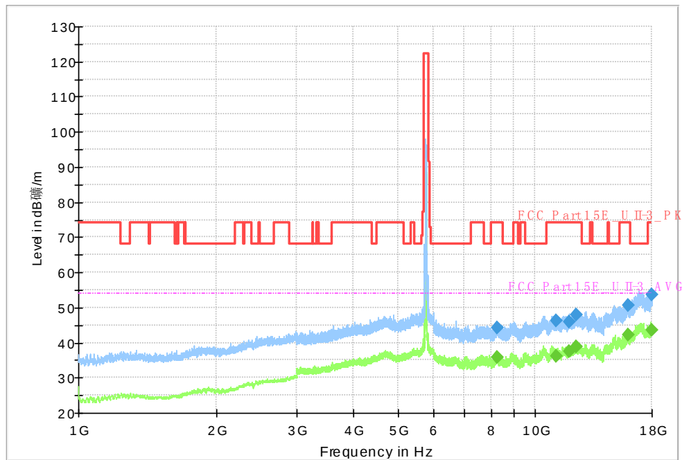
Fig. 83 Transmitter Spurious Emission (802. 11ac-VHT40, CH151 5755MHz)
