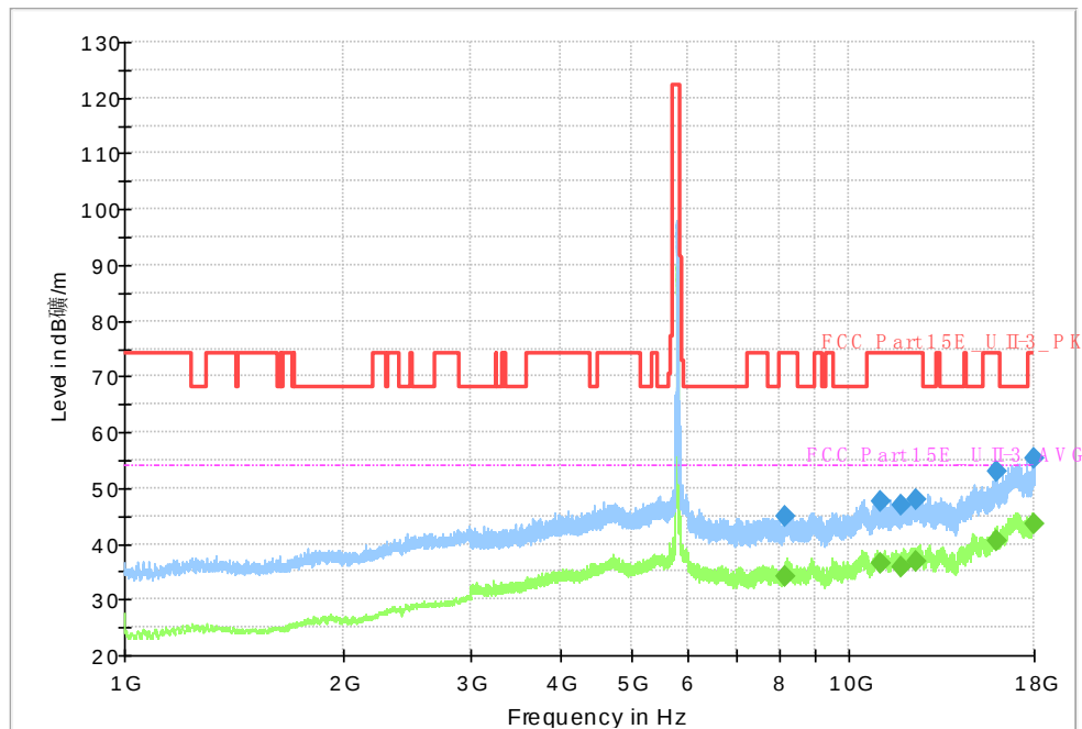
Fig. 84 Transmitter Spurious Emission (802. 11ac-VHT40, CH159 5795MHz)
