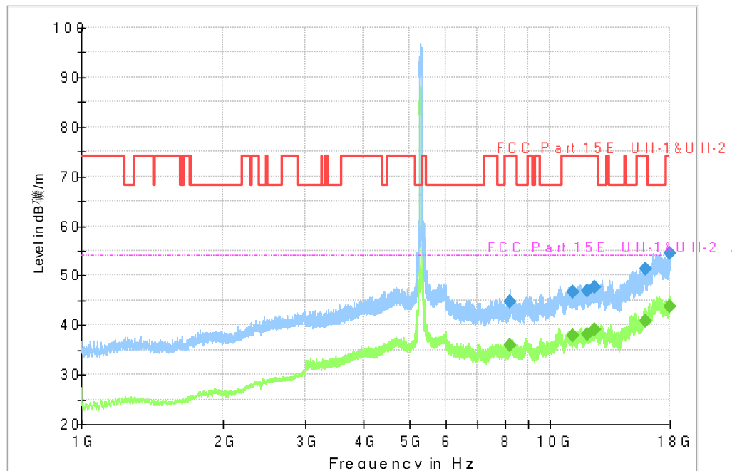
Fig. 86 Transmitter Spurious Emission (802.11ac-VHT80, CH58 5290MHz)
