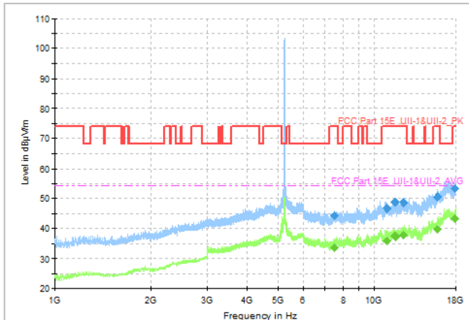
Fig. 67 Transmitter Spurious Emission (802.11a, CH48 5240MHz)
