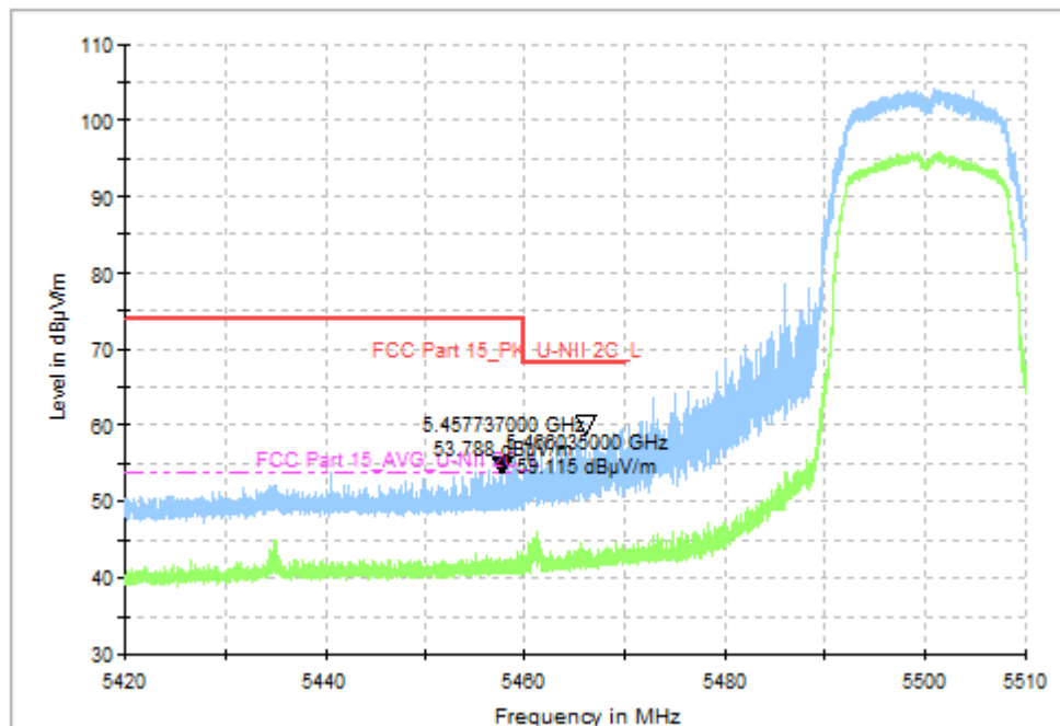
Fig. 51 Band Edges (802.11a, CH100 5500MHz)
