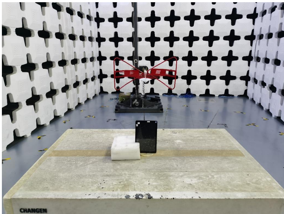
14. Radiated Emissions (Part 15C, 30MHz-1GHz)
