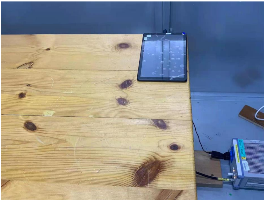
24. Conducted Emission (Part 15C, Bluetooth/Wi-Fi)
