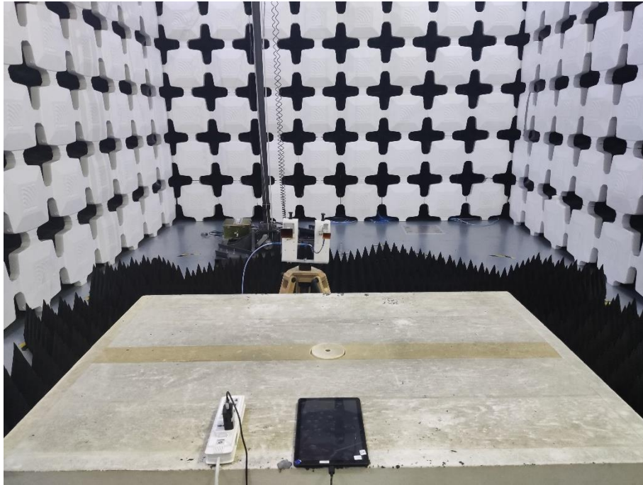
17. Radiated Emissions (Part 15C, 26.5GHz -40GHz)
