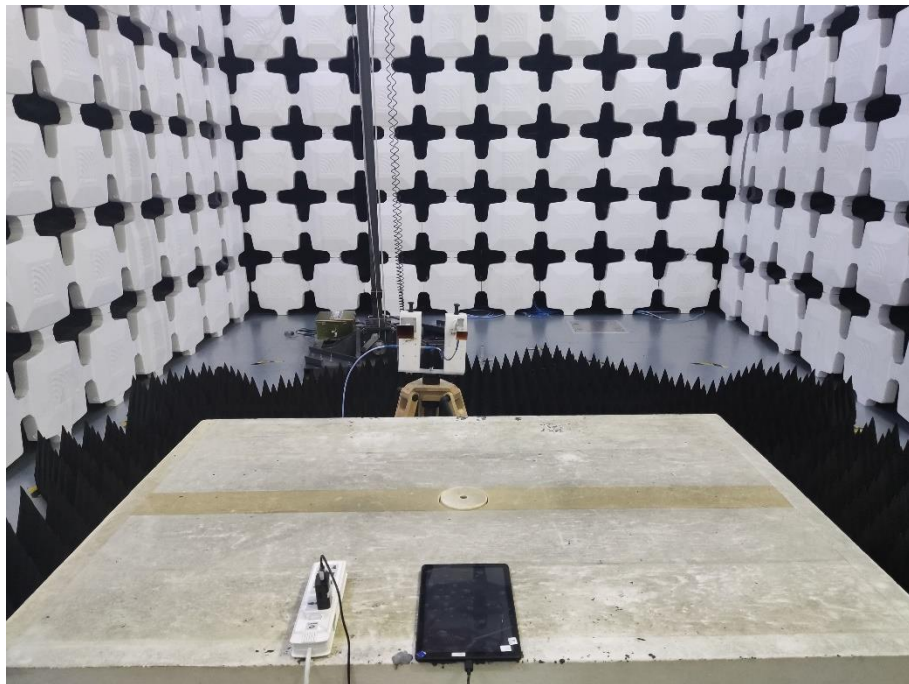
20. Radiated Emissions (Par22/24/27, 26.5GHz -40GHz)
