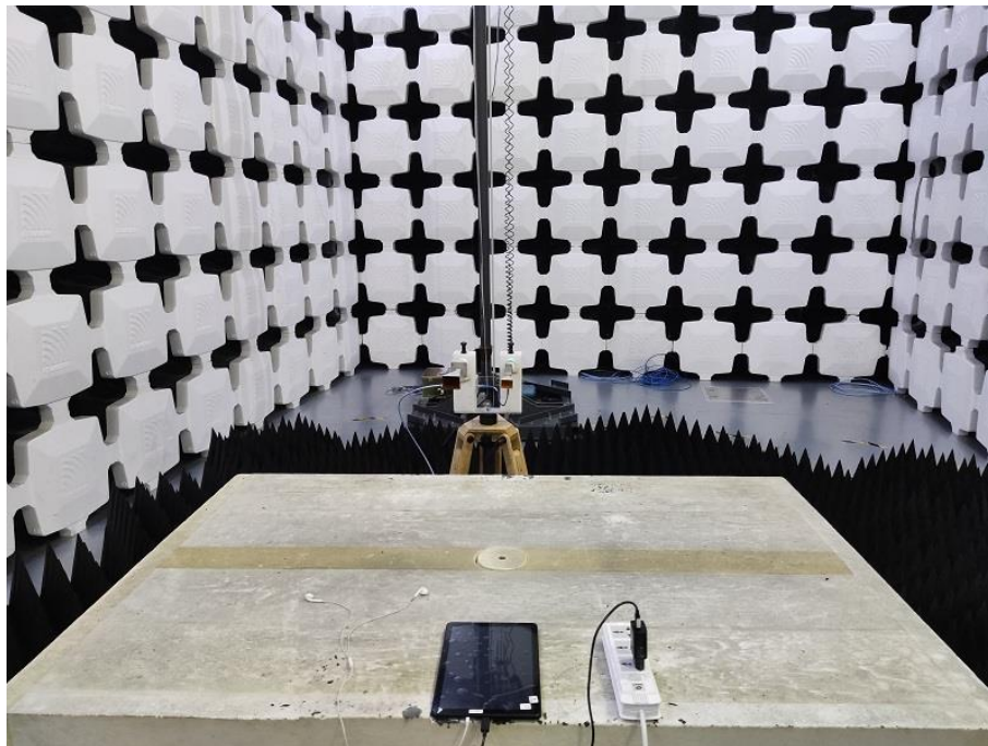
12. Radiated Emissions (Part 15B, FM receive, 26GHz-40GHz)
