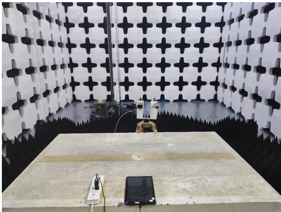
16. Radiated Emissions (Part 15C, 18GHz -26.5GHz)
