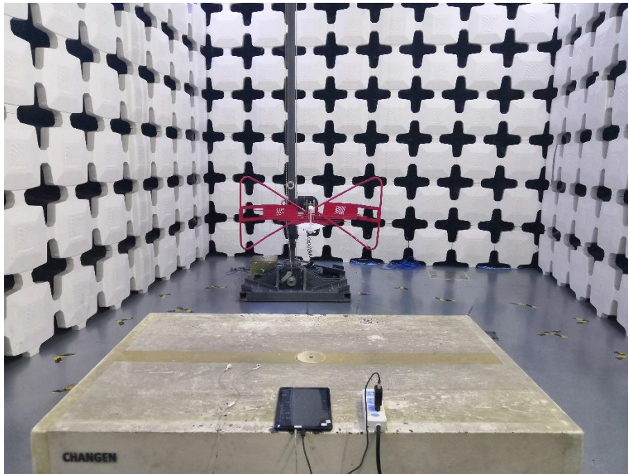
9. Radiated Emissions (Part 15B, FM receive, 30MHz-1GHz)
