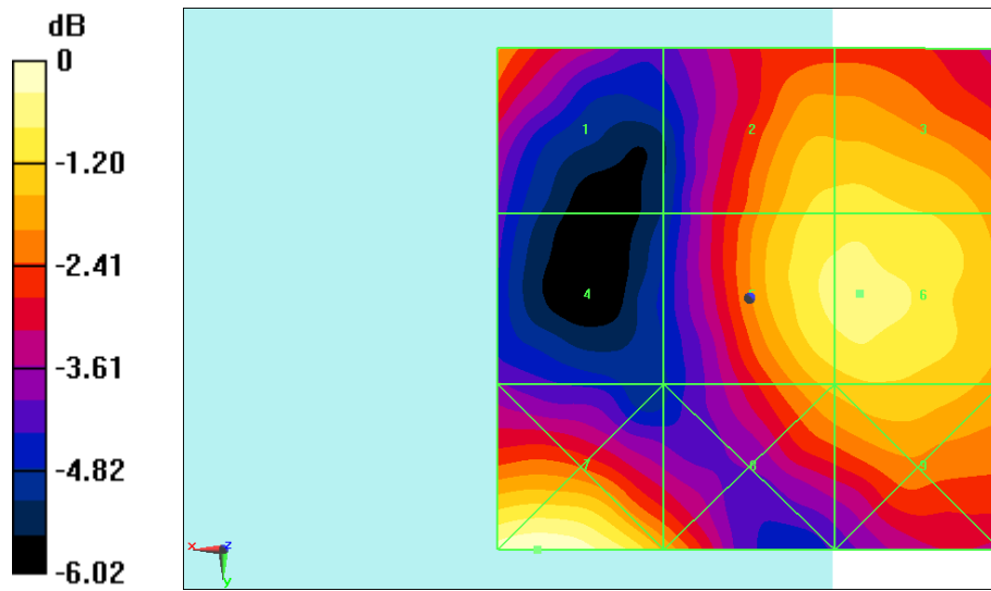
Fig B.3 HAC RF E-Field LTE Band41 QPSK CH40140
