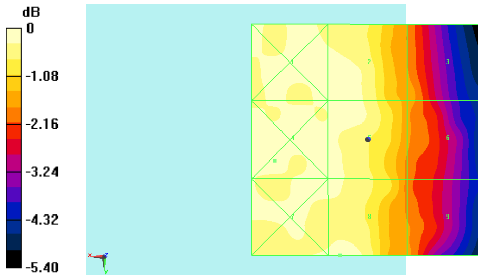
Fig B.2 HAC RF E-Field GSM 1900 Middle
