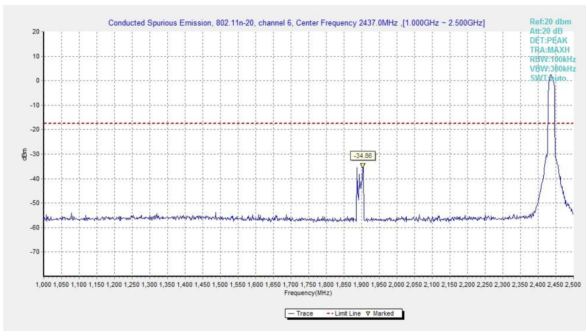
Fig.B.6.1.59 Transmitter Spurious Emission - Conducted (802.11n-HT20, Ch6, 1 GHz-2.5 GHz)
