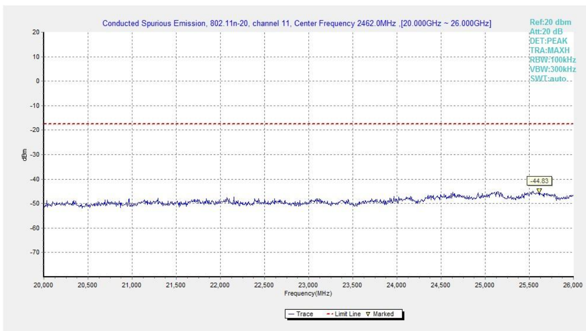
Fig.B.6.1.72 Transmitter Spurious Emission - Conducted (802.11n-HT20, Ch11, 20 GHz-26 GHz)
