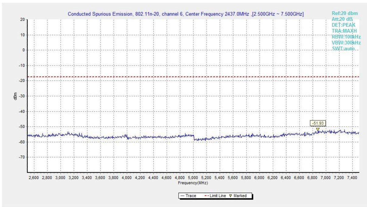
Fig.B.6.1.60 Transmitter Spurious Emission - Conducted (802.11n-HT20, Ch6, 2.5 GHz-7.5 GHz)
