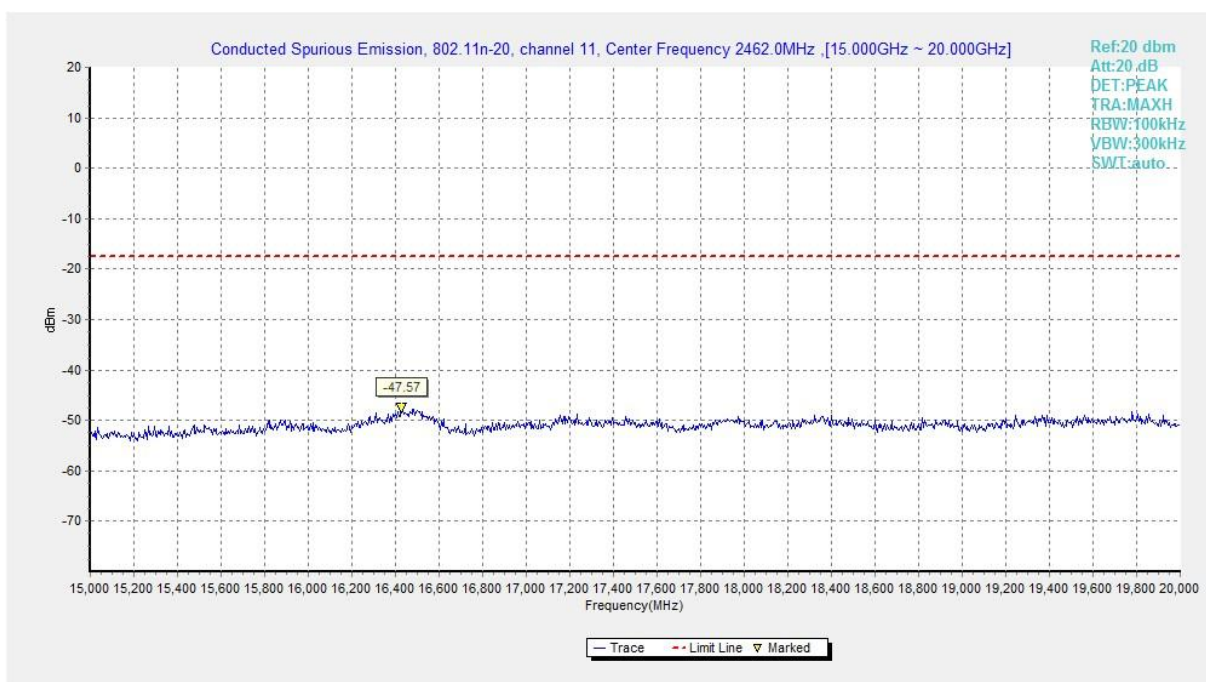
Fig.B.6.1.71 Transmitter Spurious Emission - Conducted (802.11n-HT20, Ch11, 15 GHz-20 GHz)
