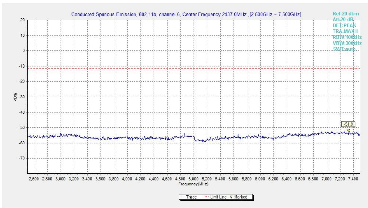
Fig.B.6.1.12 Transmitter Spurious Emission - Conducted (802.11b, Ch6, 2.5 GHz-7.5 GHz)
