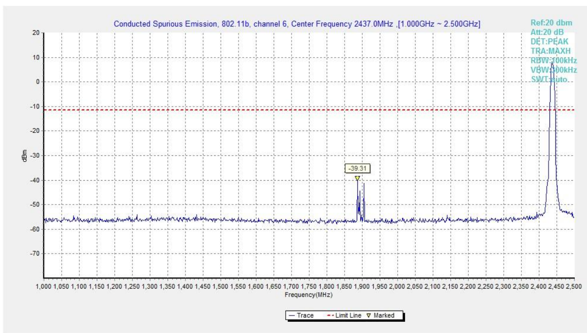
Fig.B.6.1.11 Transmitter Spurious Emission - Conducted (802.11b, Ch6, 1 GHz-2.5 GHz)
