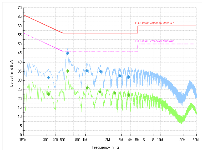
Fig.B.9.6 AC Powerline Conducted Emission with Charger AE7-Idle
