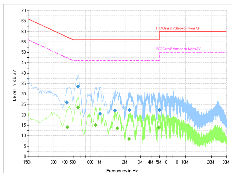
Fig.B.9.2 AC Powerline Conducted Emission with Charger AE5-Idle
