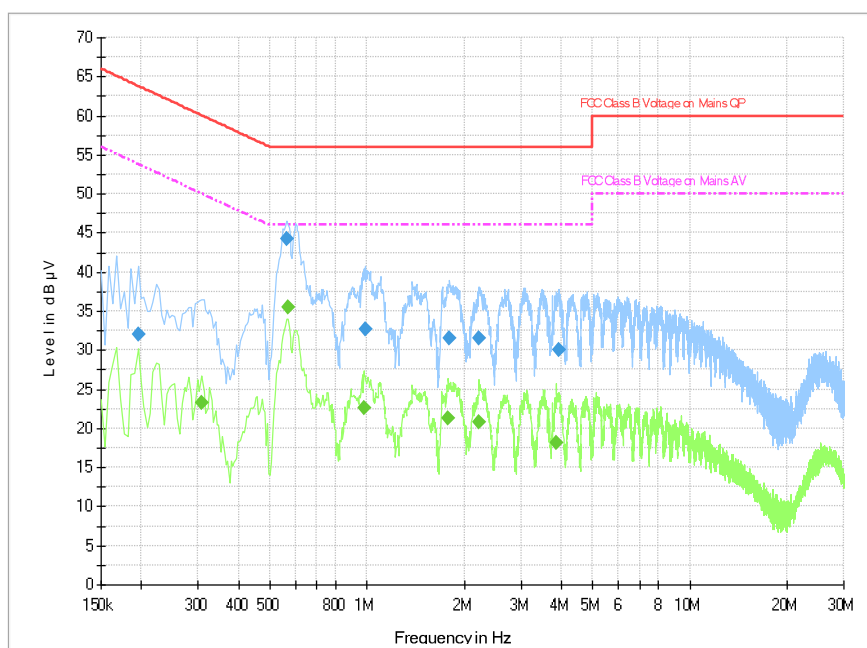
Fig.B.9.5 AC Powerline Conducted Emission with Charger AE7- bluetooth
