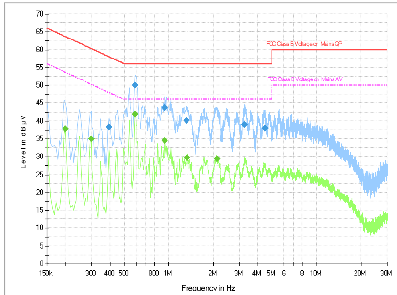
Fig.B.9.8 AC Powerline Conducted Emission with Charger AE8-Idle
