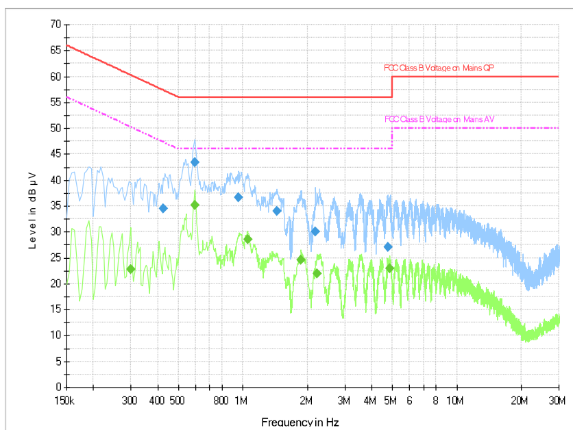
Fig.B.9.3 AC Powerline Conducted Emission with Charger AE6- bluetooth
