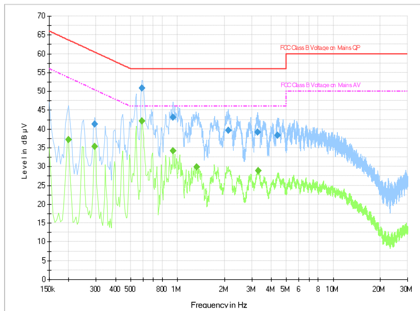
Fig.B.9.7 AC Powerline Conducted Emission with Charger AE8- bluetooth
