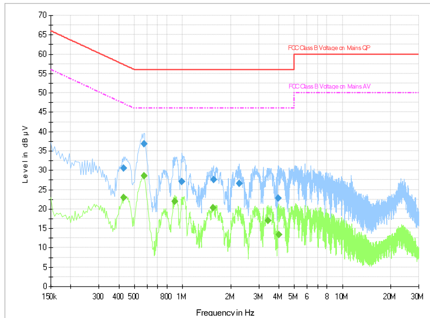
Fig.B.9.1 AC Powerline Conducted Emission with Charger AE5- bluetooth
