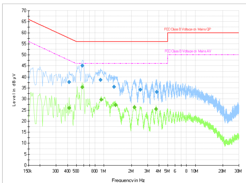
Fig.B.9.4 AC Powerline Conducted Emission with Charger AE6-Idle
