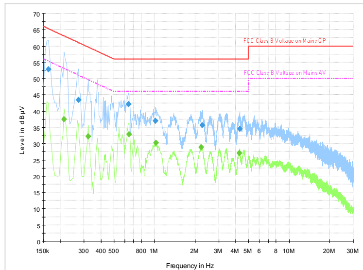
Fig.B.11.1 AC Powerline Conducted Emission- bluetooth
