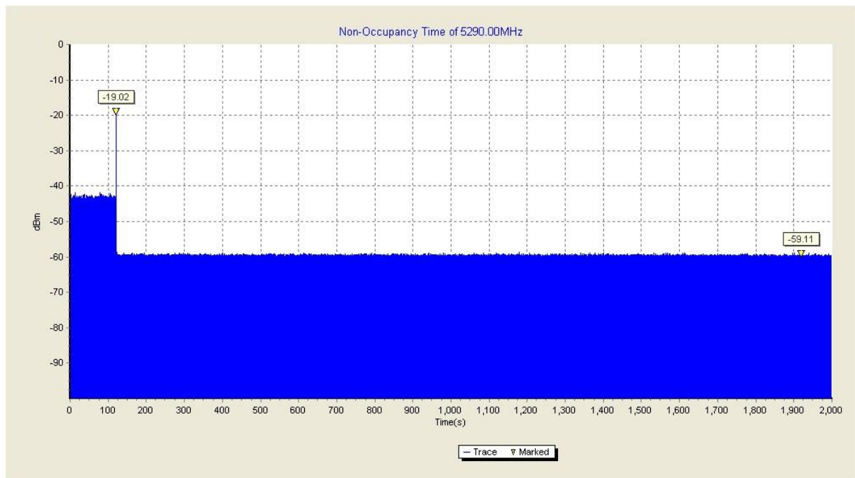
Fig.6 Non-Occupancy Period (HT80 Frequency Band: 5250MHz ~ 5350MHz)
