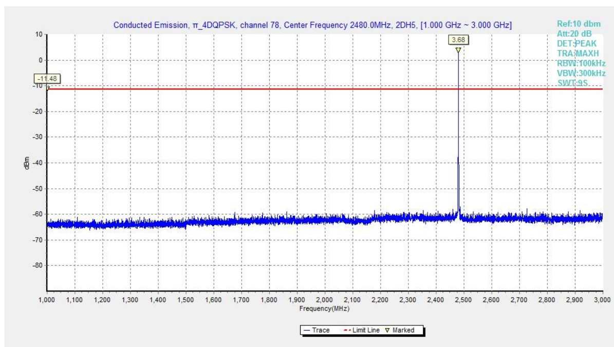
Fig. 29 Conducted Spurious Emission ( \pi/4 DQPSK, Ch78, 1GHz-3 GHz)
