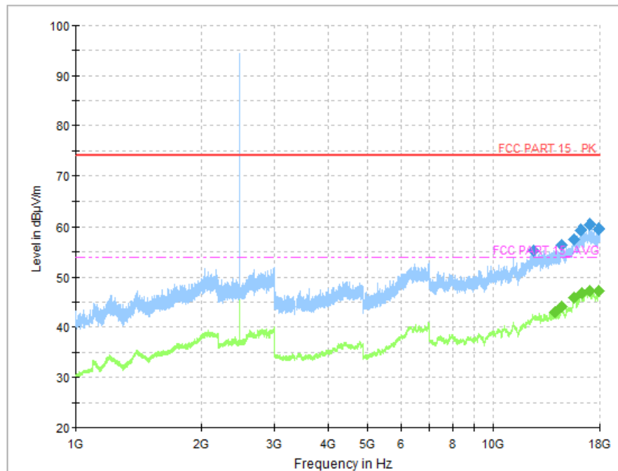
Fig. 44 Radiated Spurious Emission (GFSK, Ch78, 1GHz ~ 18GHz)
