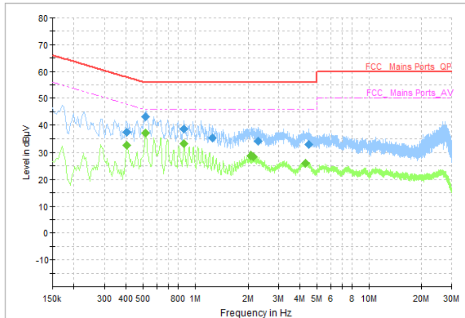
Fig. 48 AC Power line Conducted Emission (Idle)
