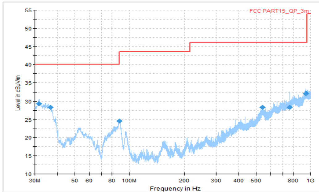
Fiture A.1. Radiated Emission (Set.1, GSM850MHz Receiver, 30MHz to 1GHz)
