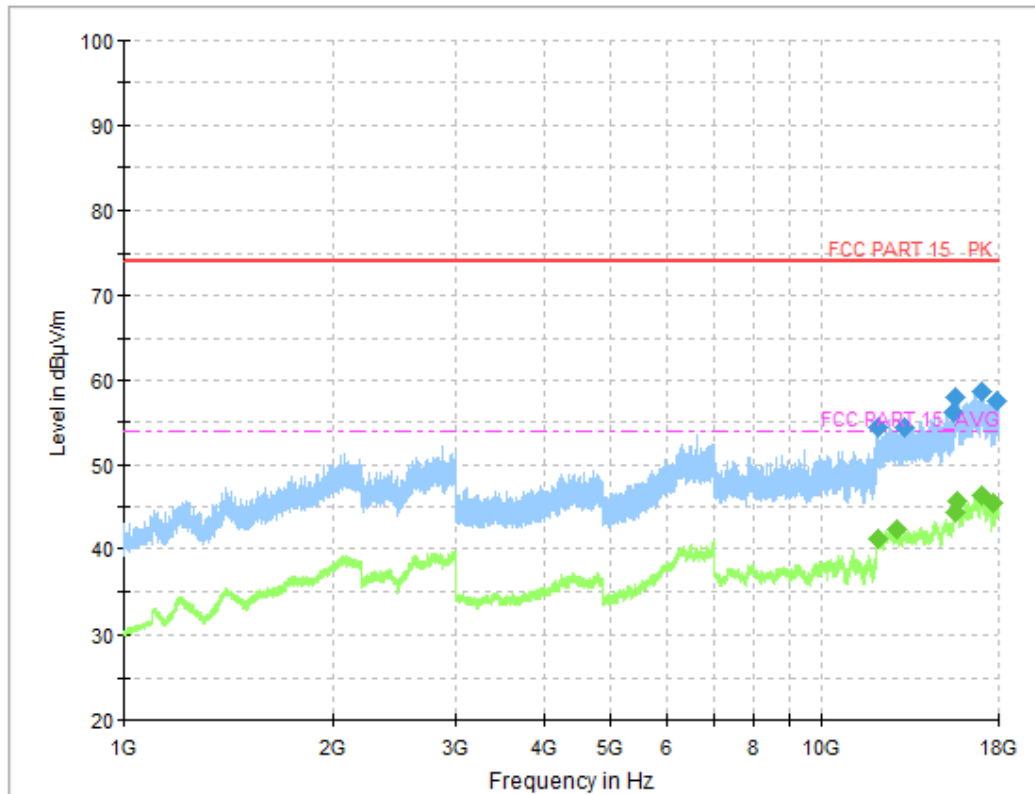
Figure B.2. Radiated Emission (Set.5, Data Transfer Mode: TF Card to PC, 1GHz to 18GHz) Final_Results_PK
