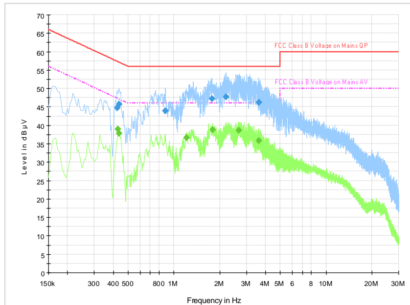
Fig.B.11.5 AC Powerline Conducted Emission- bluetooth Set.3
