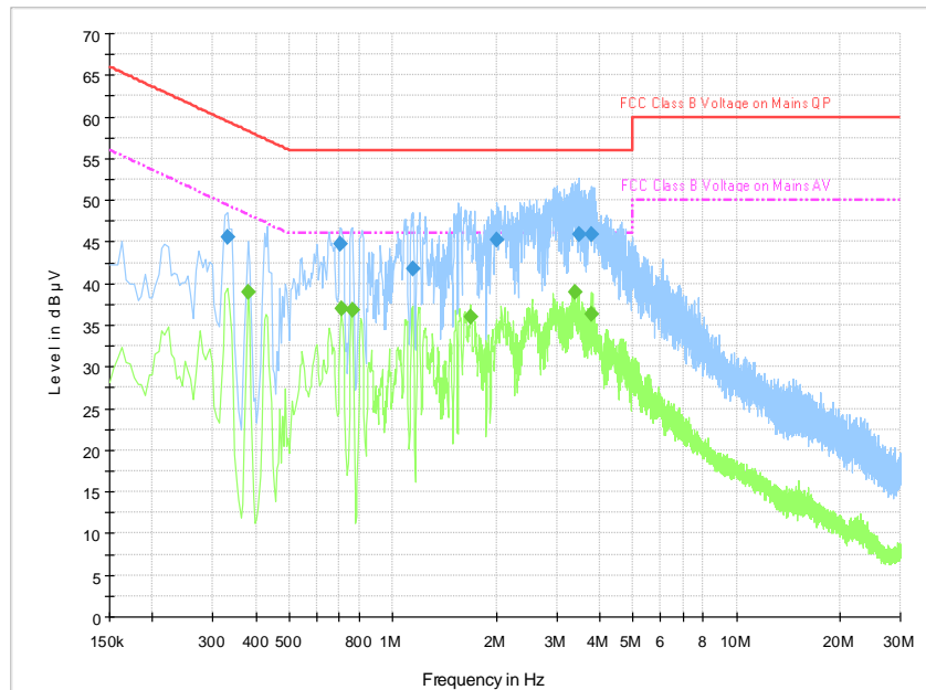
Fig.B.11.7 AC Powerline Conducted Emission- bluetooth Set.4
