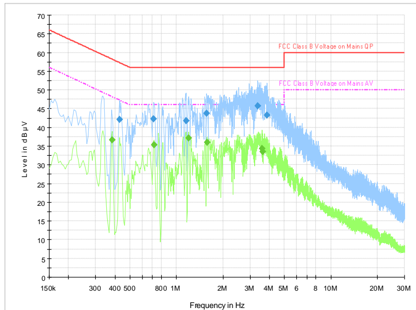
Fig.B.11.8 AC Powerline Conducted Emission-Iidle Set.4
