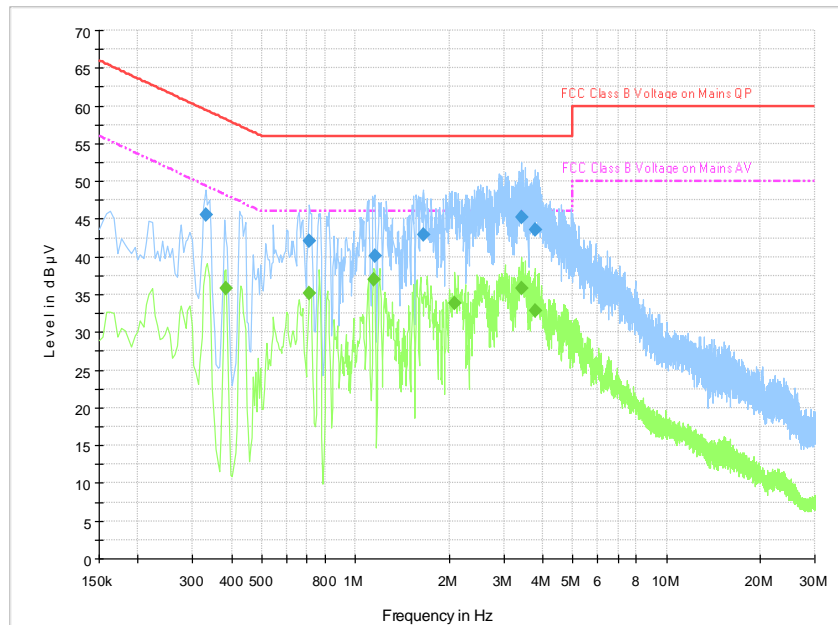
Fig.B.11.3 AC Powerline Conducted Emission- bluetooth Set.2
