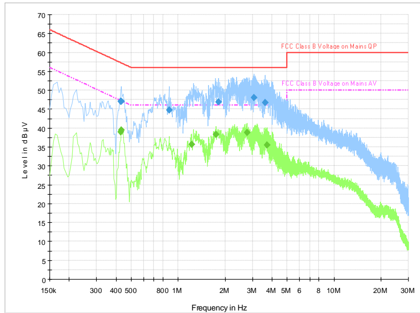
Fig.B.11.1 AC Powerline Conducted Emission- bluetooth Set.1
