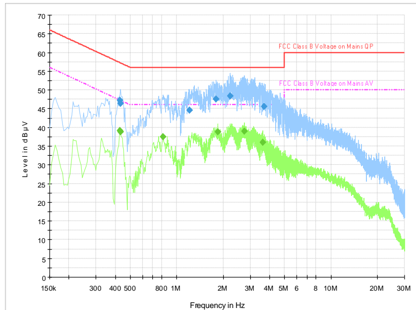
Fig.B.11.6 AC Powerline Conducted Emission-Idle Set.3
