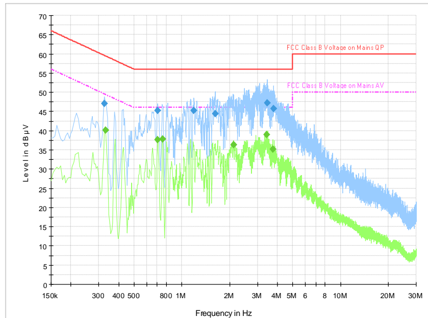
Fig.B.11.4 AC Powerline Conducted Emission-Iidle Set.2
