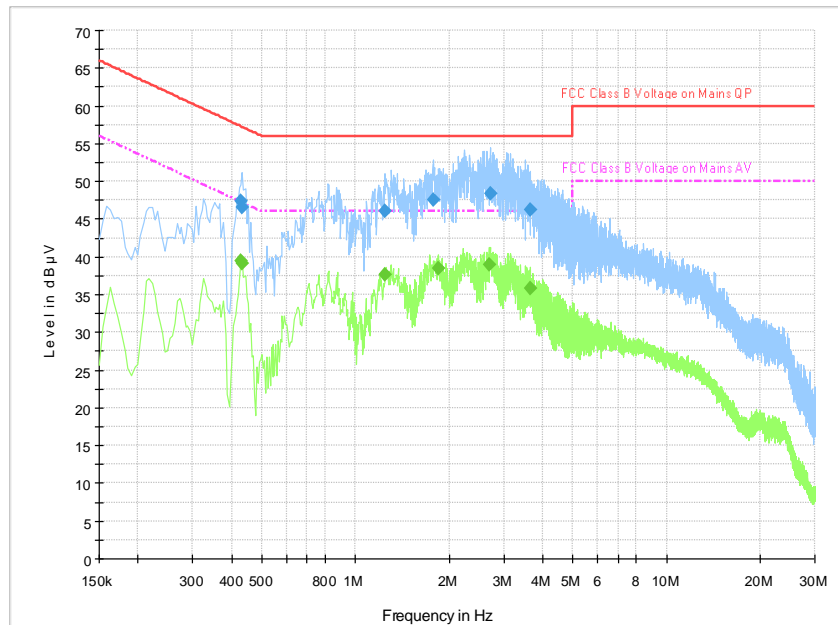
Fig.B.11.2 AC Powerline Conducted Emission-Idle Set.1
