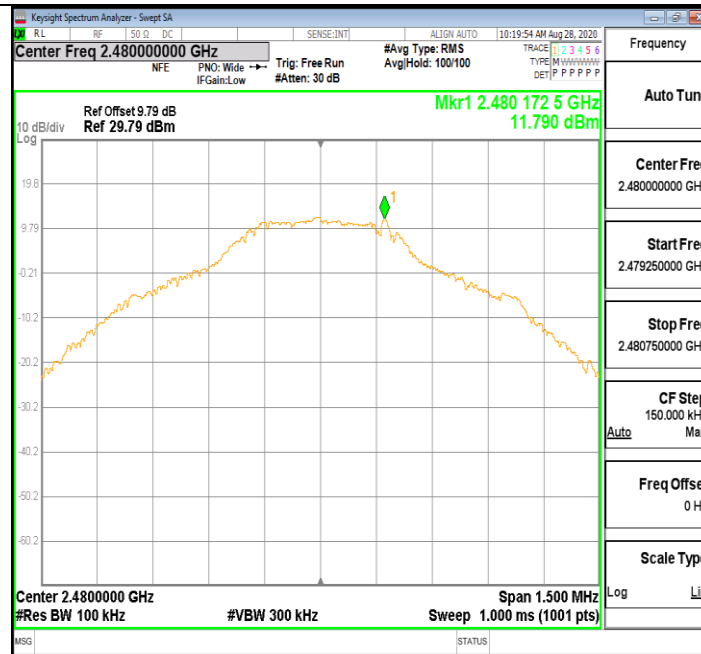
DH5_Ant1_2480_0~Reference
