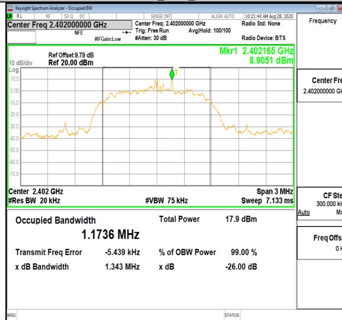
3DH5_Ant1_2402
