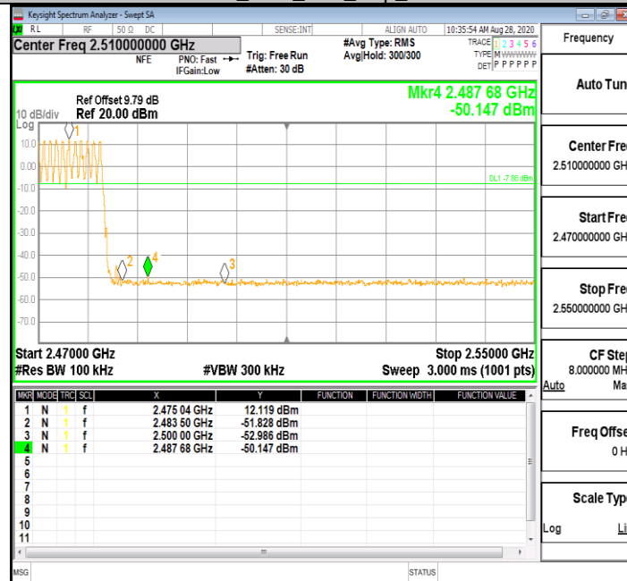
DH5_Ant1_High_Hop_2480
