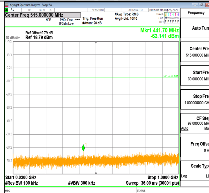
3DH5_Ant1_2441_30~1000
