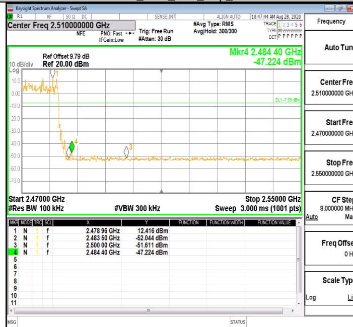
3DH5_Ant1_High_Hop_2480
