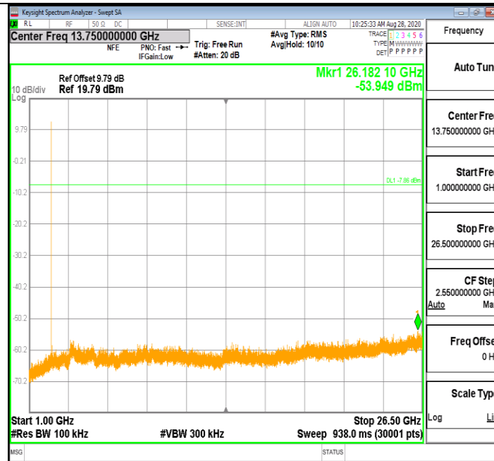
3DH5_Ant1_2441_1000~26500
