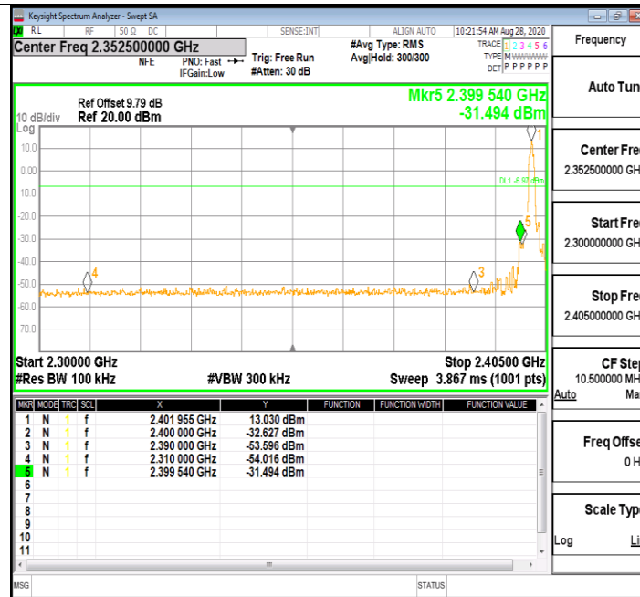
3DH5_Ant1_Low_2402
