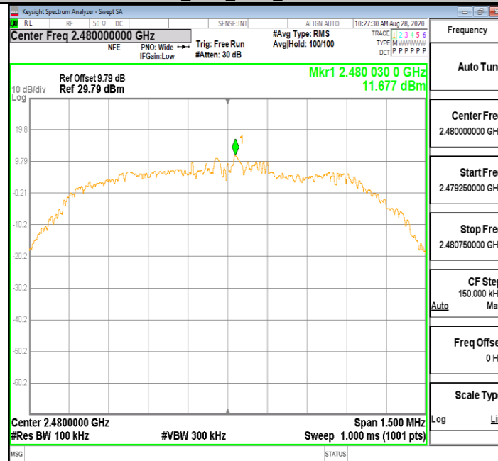
3DH5_Ant1_2480_0~Reference
