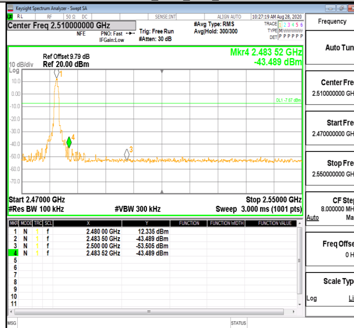
3DH5_Ant1_High_2480
