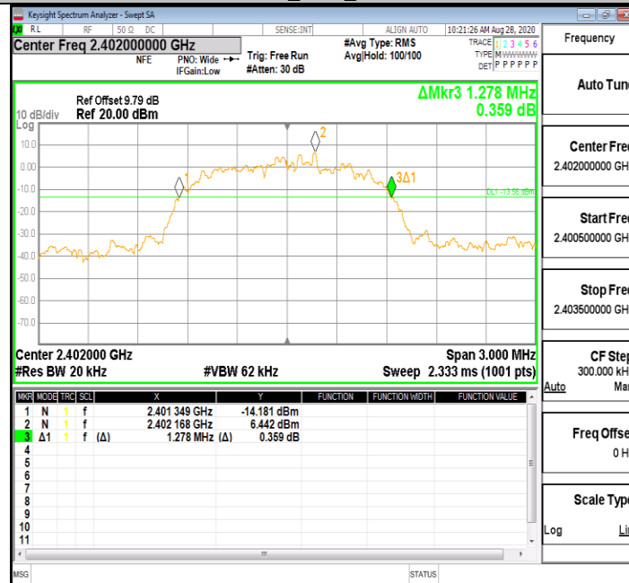
3DH5_Ant1_2402
