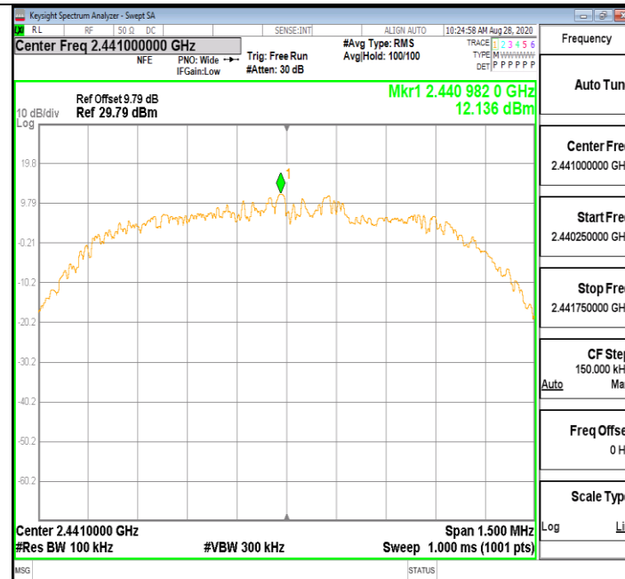
3DH5_Ant1_2441_0~Reference
