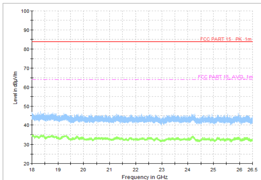
Fig.62 Radiated Spurious Emission (All Channels, 18GHz-26.5GHz)
