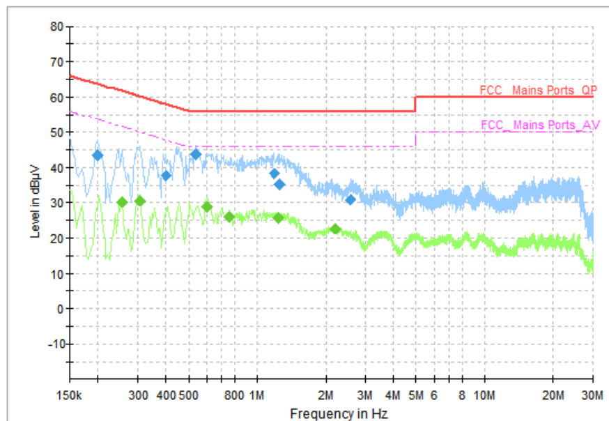
Fig.66 AC Power line Conducted Emission (Idle, AE4, 120V)
