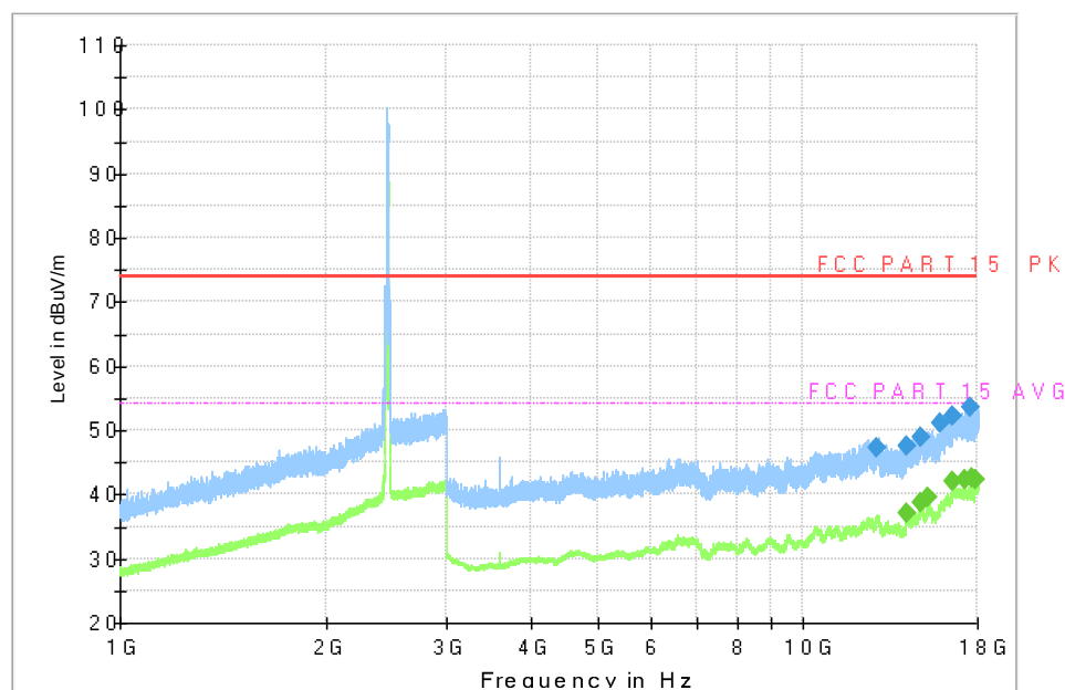
Fig.52 Radiated Spurious Emission (802.11g, CH11, 1GHz-18GHz)
