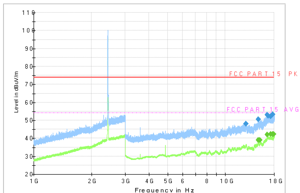
Fig.56 Radiated Spurious Emission (802.11n HT20, CH6, 1GHz-18GHz)
