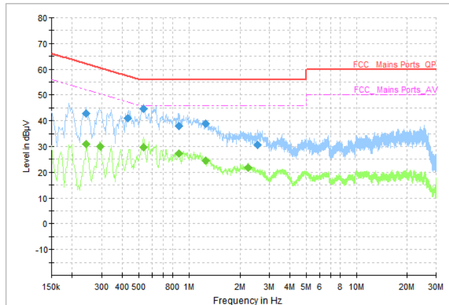
Fig.65 AC Power line Conducted Emission (Traffic, AE4, 120V)
