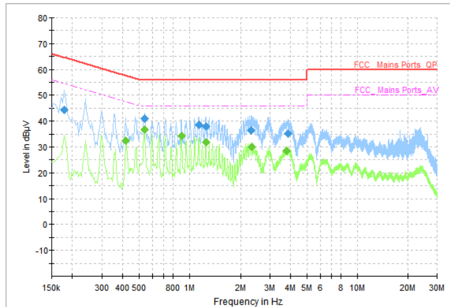
Fig.64 AC Power line Conducted Emission (Idle, AE3, 120V)
