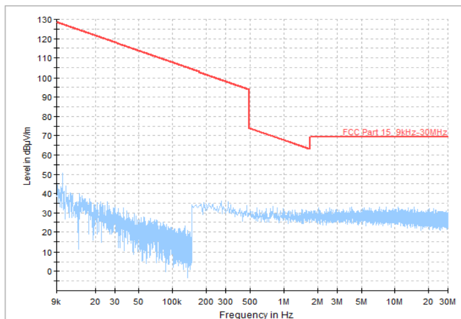
Fig.60 Radiated Spurious Emission (All Channels, 9KHz-30MHz)
