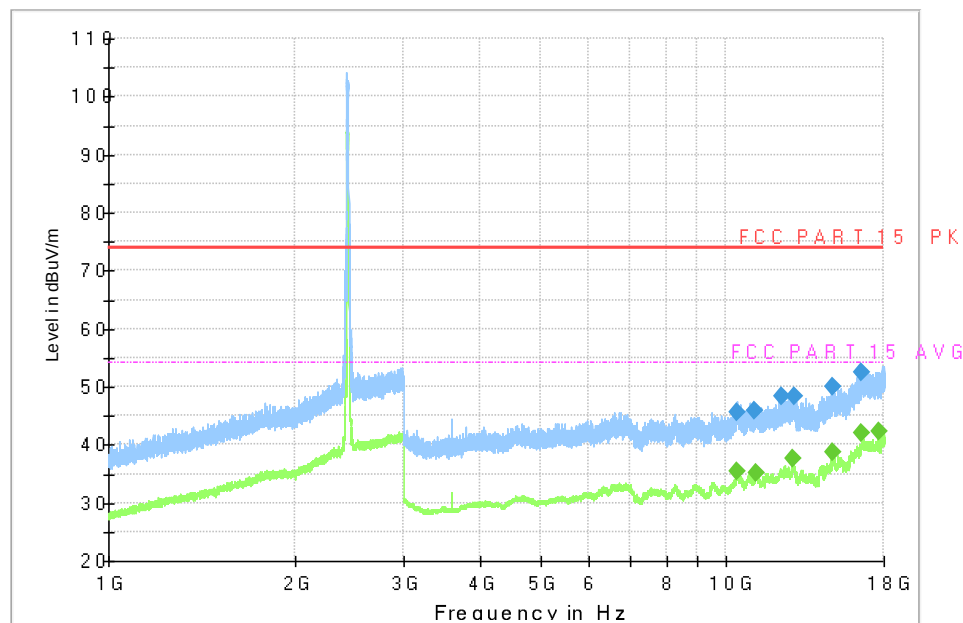
Fig.51 Radiated Spurious Emission (802.11g, CH6, 1GHz-18GHz)
