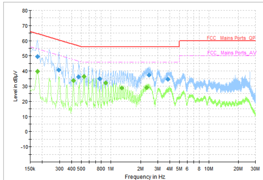
Fig.63 AC Power line Conducted Emission (Traffic, AE3, 120V)
