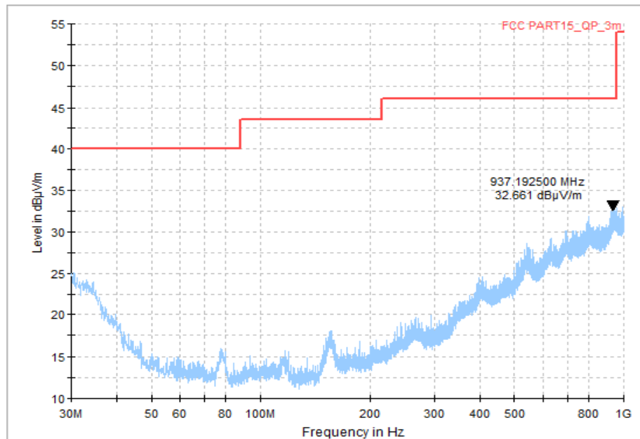
Fig.61 Radiated Spurious Emission (All Channels, 30MHz-1GHz)
