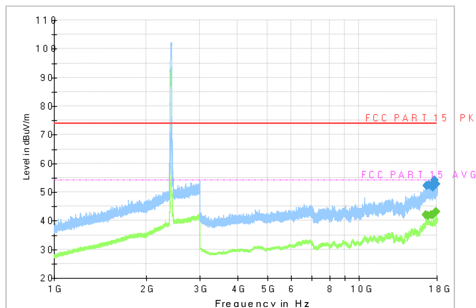
Fig.50 Radiated Spurious Emission (802.11g, CH1, 1GHz-18GHz)
