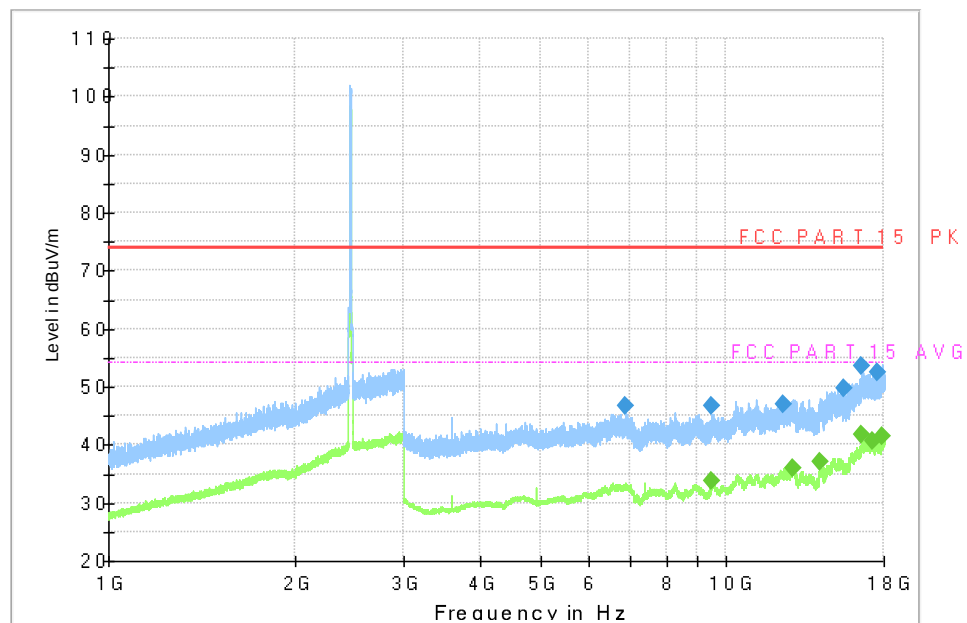
Fig.47 Radiated Spurious Emission (802.11b, CH11, 1GHz-18GHz)
