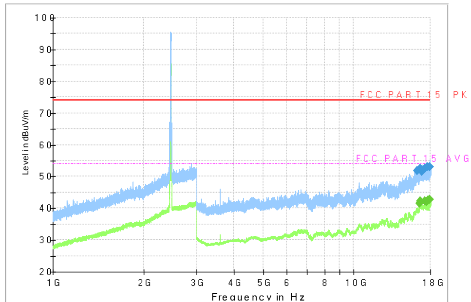
Fig.57 Radiated Spurious Emission (802.11n HT20, CH11, 1GHz-18GHz)
