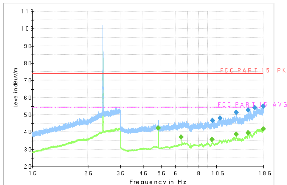
Fig.45 Radiated Spurious Emission (802.11b, CH1, 1GHz-18GHz)
