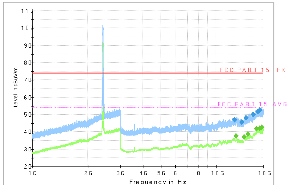
Fig.55 Radiated Spurious Emission (802.11n HT20, CH1, 1GHz-18GHz)
