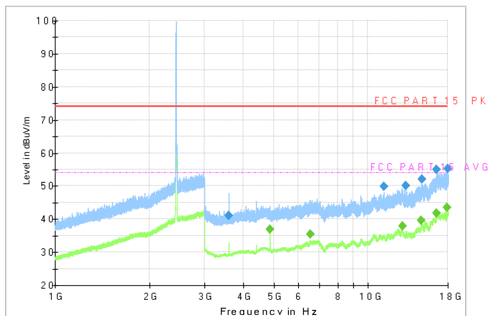
Fig.46 Radiated Spurious Emission (802.11b, CH6, 1GHz-18GHz)
