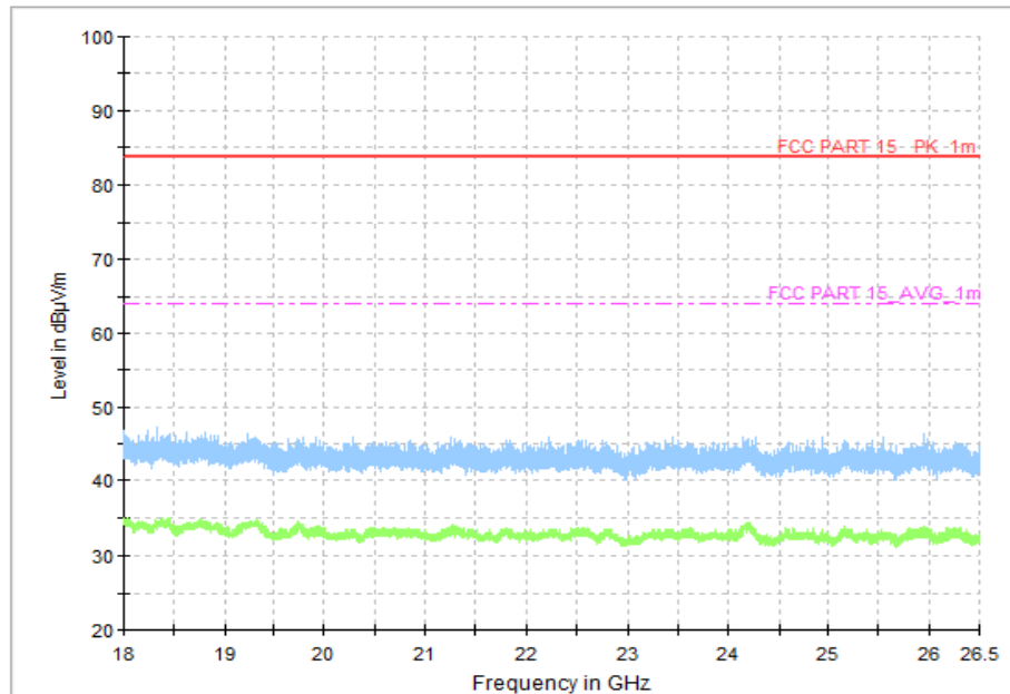
Fig.24 Radiated Spurious Emission (Ch19, 18 GHz - 26.5 GHz), 1M
