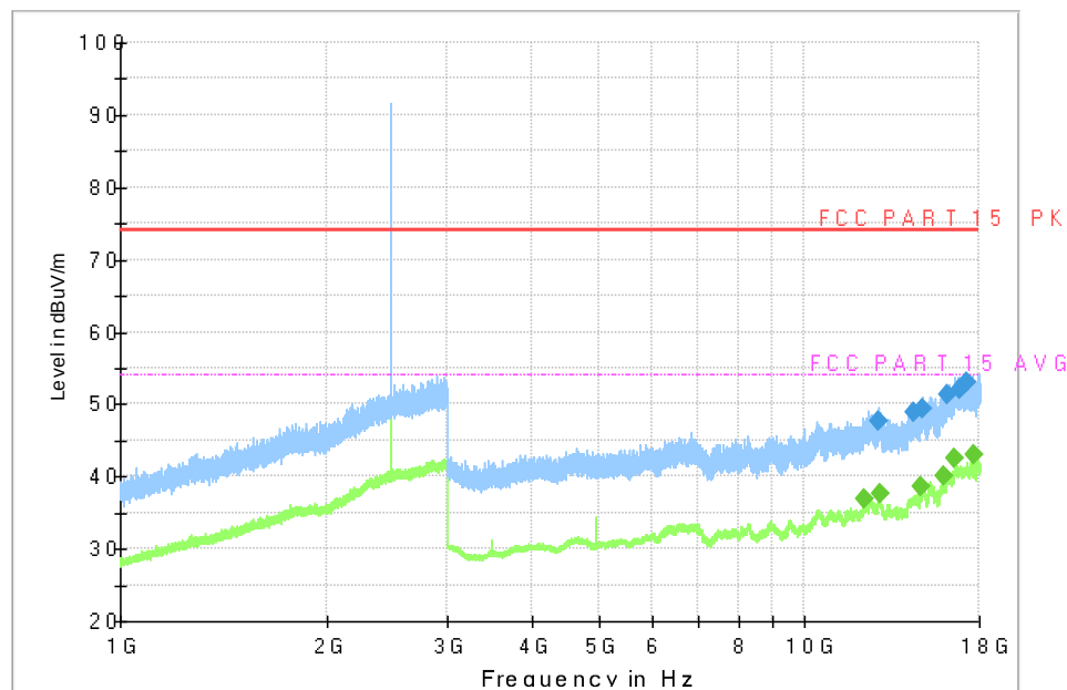
Fig.25 Radiated Spurious Emission (Ch39, 1 GHz - 18 GHz), 1M
