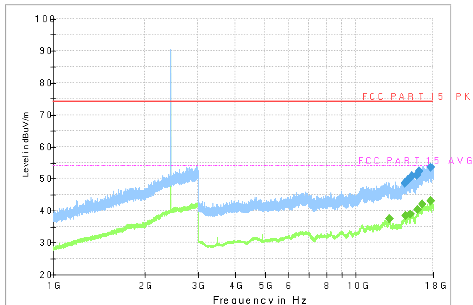
Fig.23 Radiated Spurious Emission (Ch19, 1 GHz - 18 GHz), 1M
