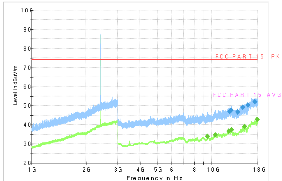
Fig.20 Radiated Spurious Emission (Ch0, 1 GHz - 18 GHz), 1M
