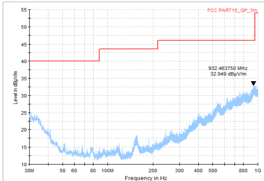
Fig.22 Radiated Spurious Emission (Ch19, 30 MHz - 1 GHz), 1M
