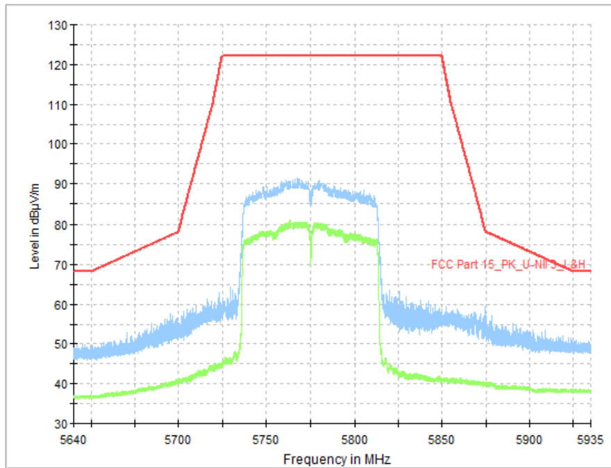
Fig. 41 Band Edges (802.11ac-VHT80, CH155 5775MHz)
