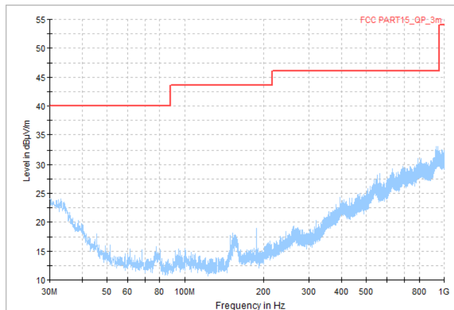
Fig. 60 Transmitter Spurious Emission (All channel, 30MHz~1GHz)
