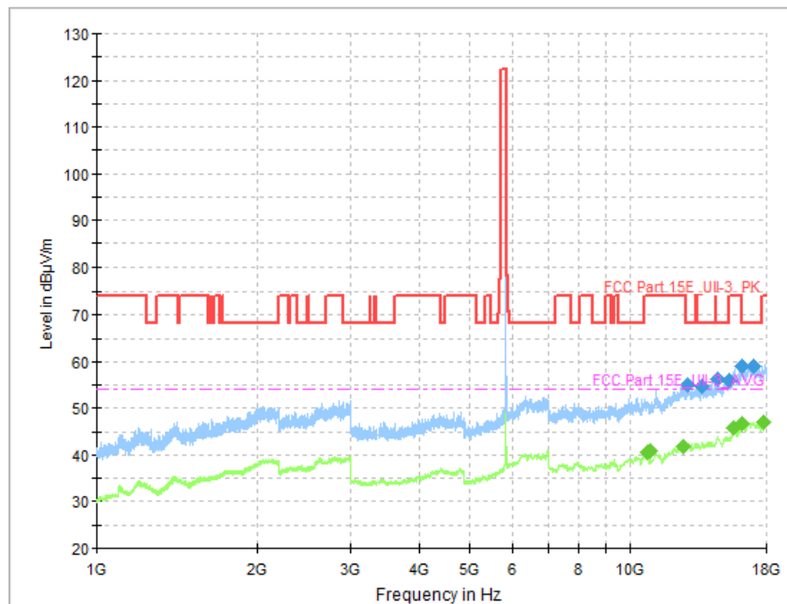
Fig. 50 Transmitter Spurious Emission (802. 11a, CH165 5825MHz)
