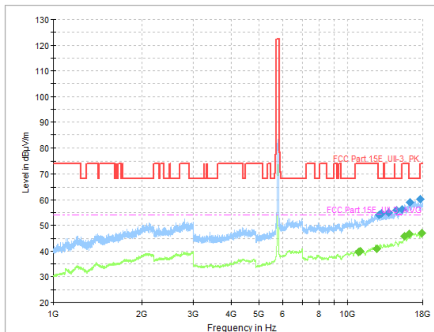
Fig. 59 Transmitter Spurious Emission (802. 11ac-VHT80, CH155 5775MHz)
