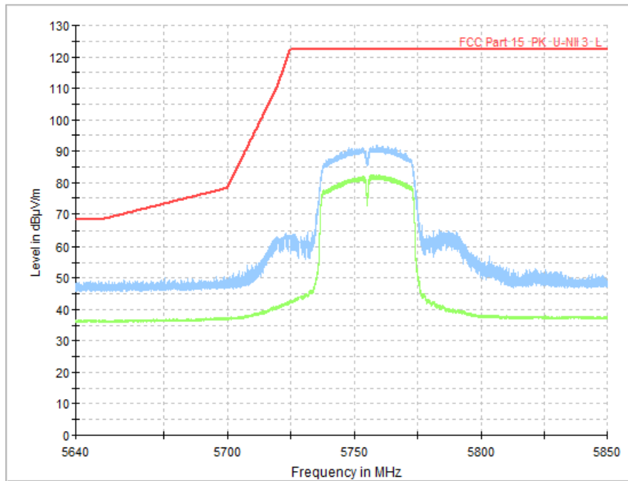
Fig. 37 Band Edges (802.11n-HT40, CH151 5755MHz)
