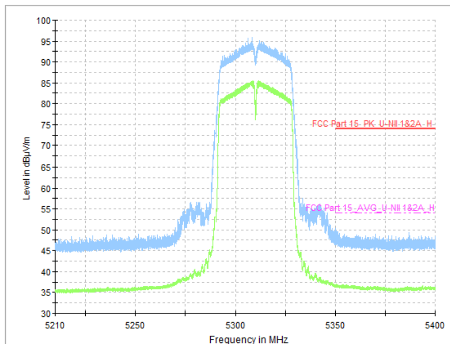
Fig. 36 Band Edges (802.11n-HT40, CH62 5310MHz)
