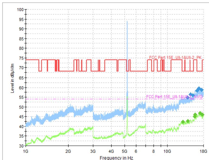
Fig. 51 Transmitter Spurious Emission (802.11n-HT40, CH38 5190MHz)
