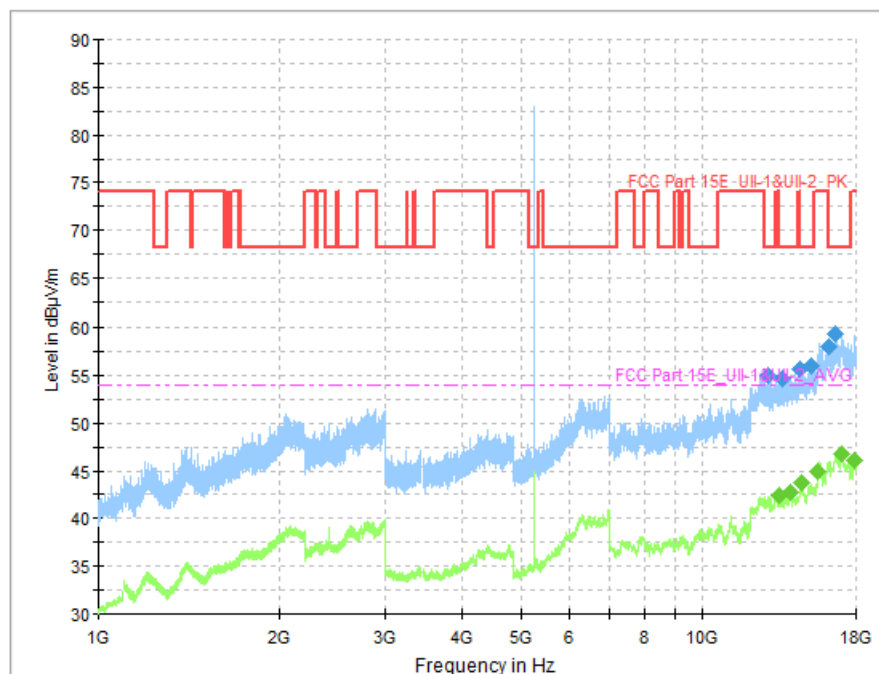
Fig. 45 Transmitter Spurious Emission (802.11a, CH52 5260MHz)
