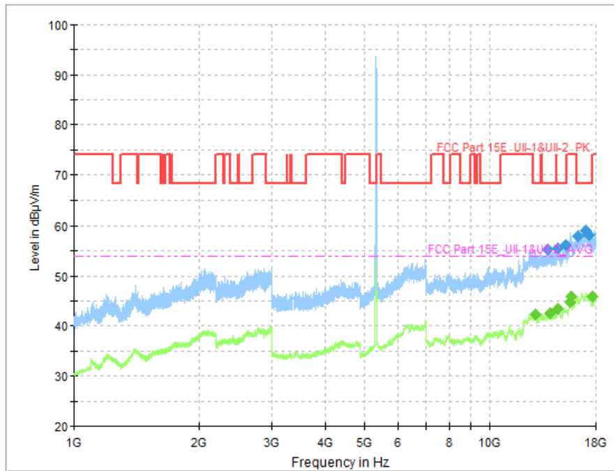
Fig. 54 Transmitter Spurious Emission (802.11n-HT40, CH62 5310MHz)
