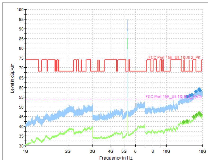
Fig. 53 Transmitter Spurious Emission (802.11n-HT40, CH54 5270MHz)
