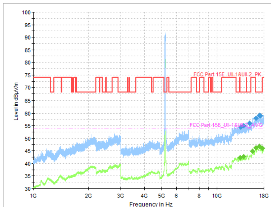
Fig. 57 Transmitter Spurious Emission (802. 11ac-VHT80, CH42 5210MHz)
