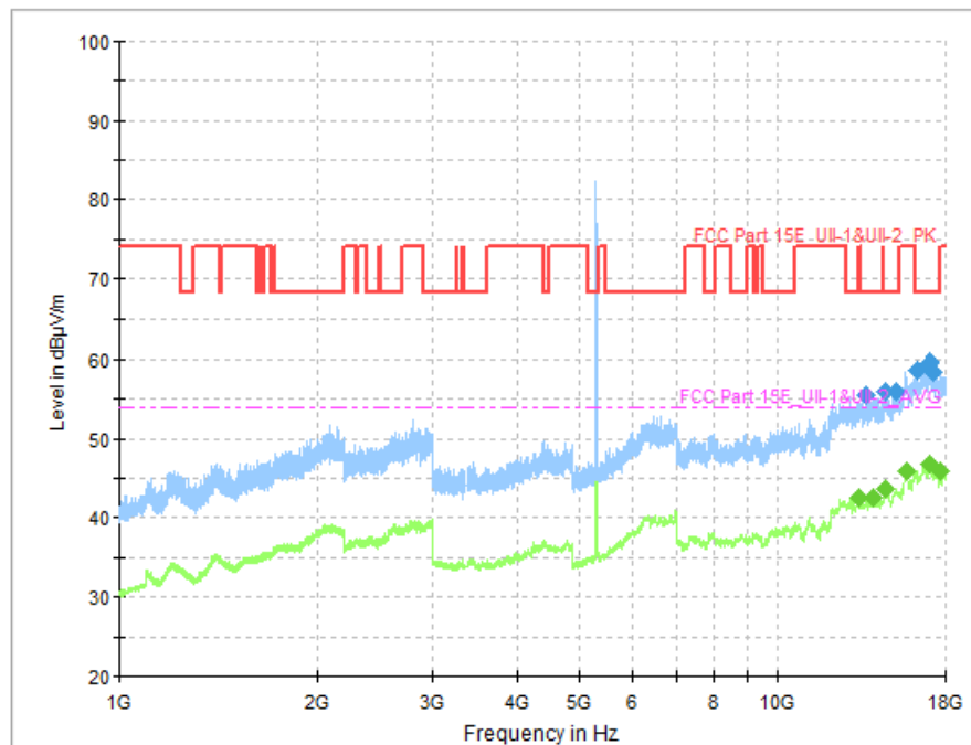
Fig. 46 Transmitter Spurious Emission (802.11a, CH56 5280MHz)
