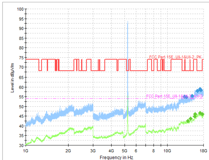
Fig. 52 Transmitter Spurious Emission (802.11n-HT40, CH46 5230MHz)
