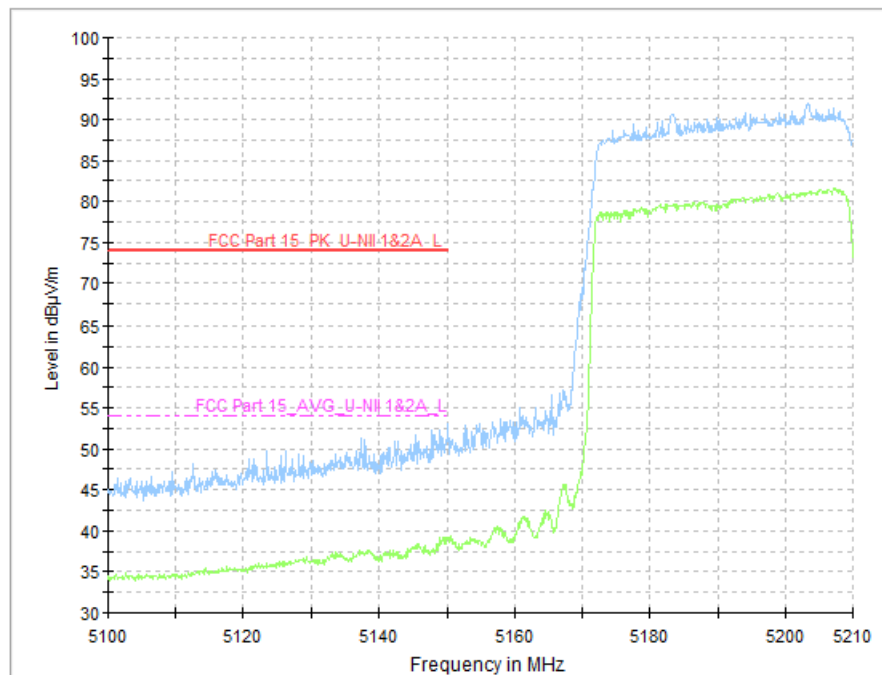
Fig. 39 Band Edges (802.11ac-VHT80, CH42 5210MHz)
