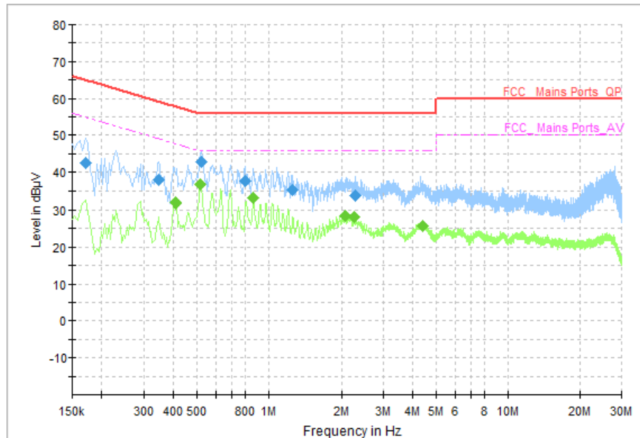
Fig. 64 AC Power line Conducted Emission (Traffic)
