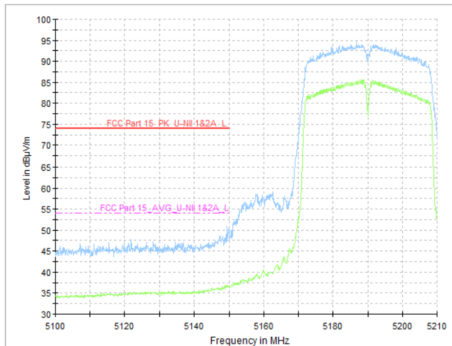
Fig. 35 Band Edges (802.11n-HT40, CH38 5190MHz)
