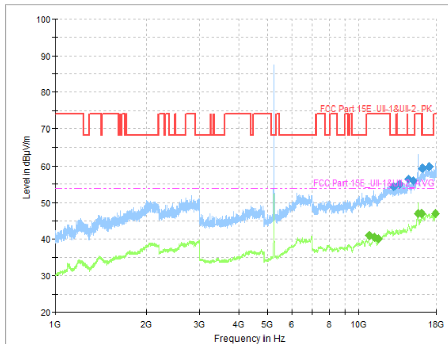
Fig. 44 Transmitter Spurious Emission (802.11a, CH48 5240MHz)
