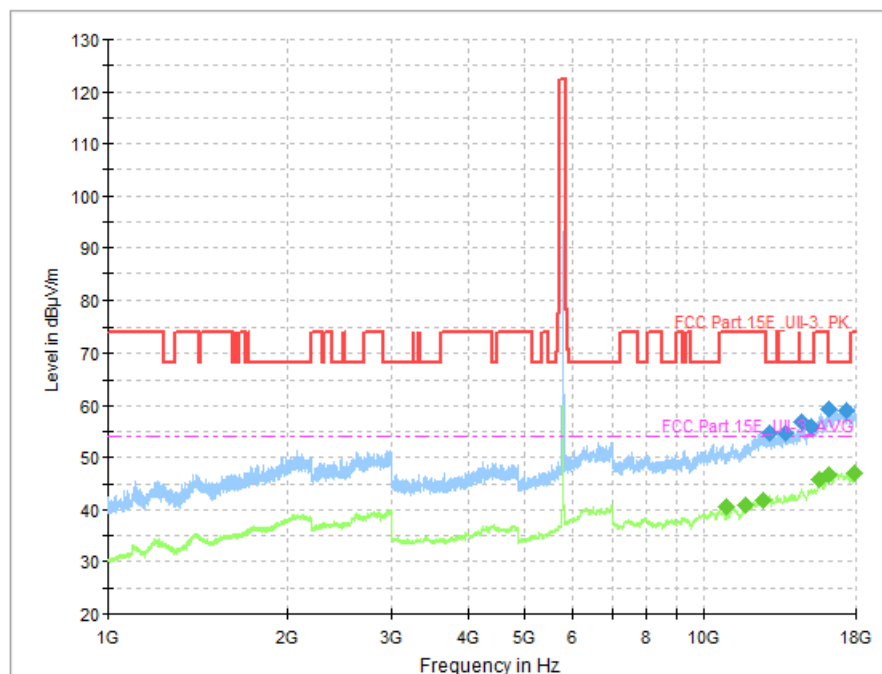
Fig. 49 Transmitter Spurious Emission (802. 11a, CH157 5785MHz)
