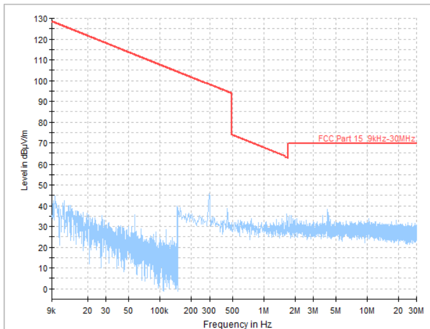
Fig. 63 Radiated Spurious Emission (All Channel, 9 kHz ~30 MHz)
