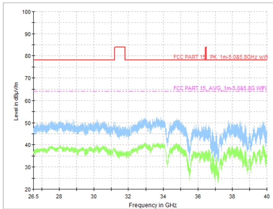
Fig. 62 Transmitter Spurious Emission (All channel, 26.5GHz~40GHz)
