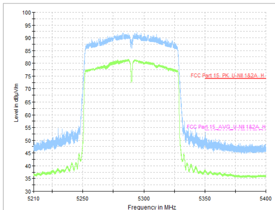
Fig. 40 Band Edges (802.11ac-VHT80, CH58 5290MHz)
