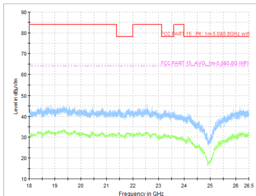
Fig. 61 Transmitter Spurious Emission (All channel, 18GHz~26.5GHz)
