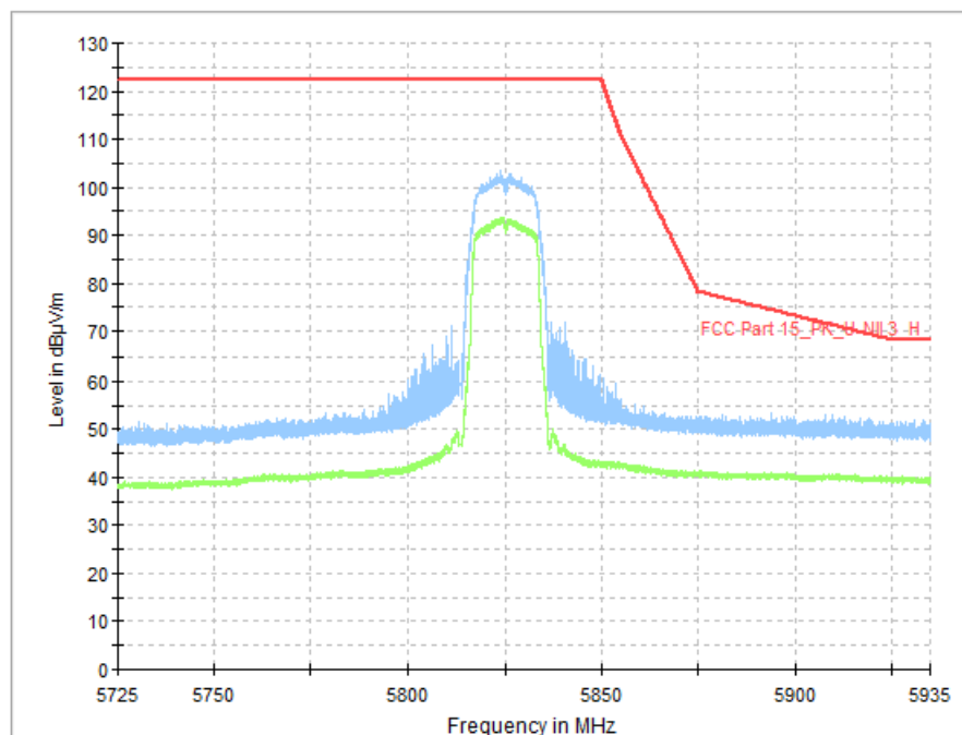
Fig. 34 Band Edges (802.11a, CH165 5825MHz)
