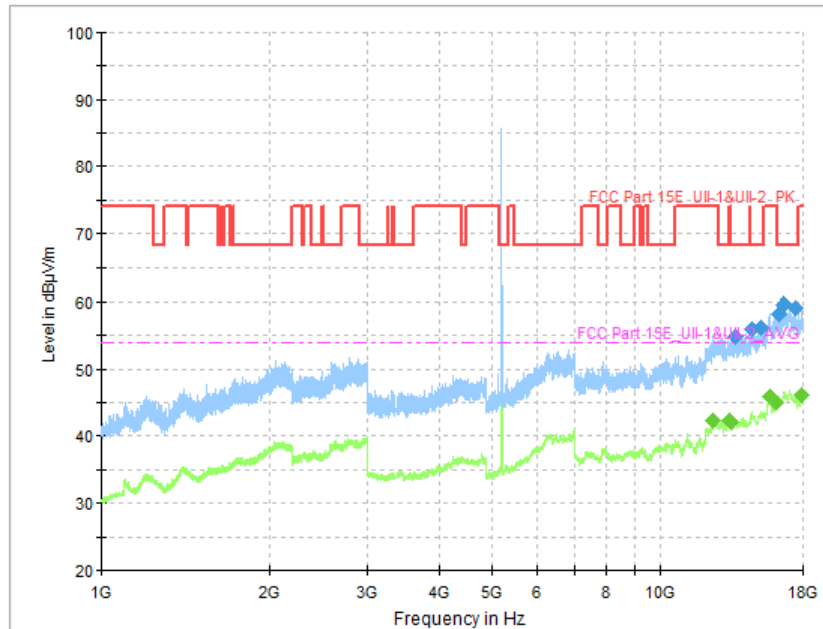
Fig. 42 Transmitter Spurious Emission (802.11a, CH36 5180MHz)
