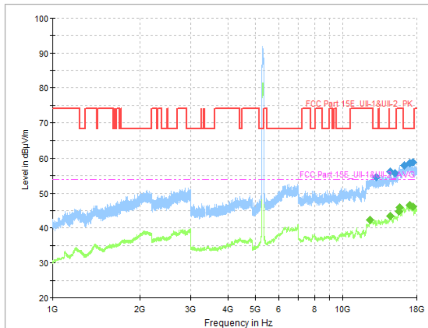
Fig. 58 Transmitter Spurious Emission (802. 11ac-VHT80, CH58 5290MHz)
