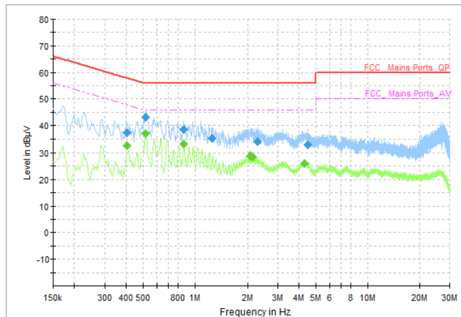
Fig. 65 AC Power line Conducted Emission (Idle)
