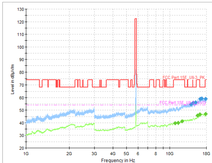
Fig. 56 Transmitter Spurious Emission (802. 11n-HT40, CH159 5795MHz)
