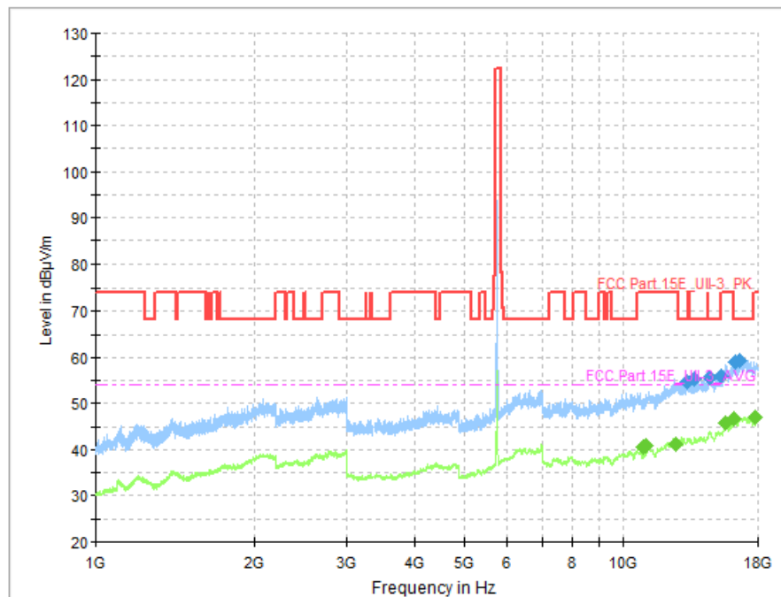
Fig. 48 Transmitter Spurious Emission (802. 11a, CH149 5745MHz)
