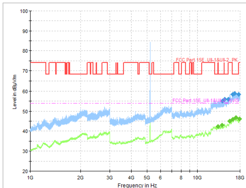
Fig. 43 Transmitter Spurious Emission (802.11a, CH40 5200MHz)
