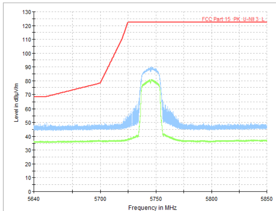
Fig. 33 Band Edges (802.11a, CH149 5745MHz)
