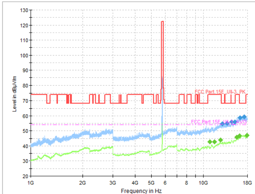
Fig. 55 Transmitter Spurious Emission (802. 11n-HT40, CH151 5755MHz)
