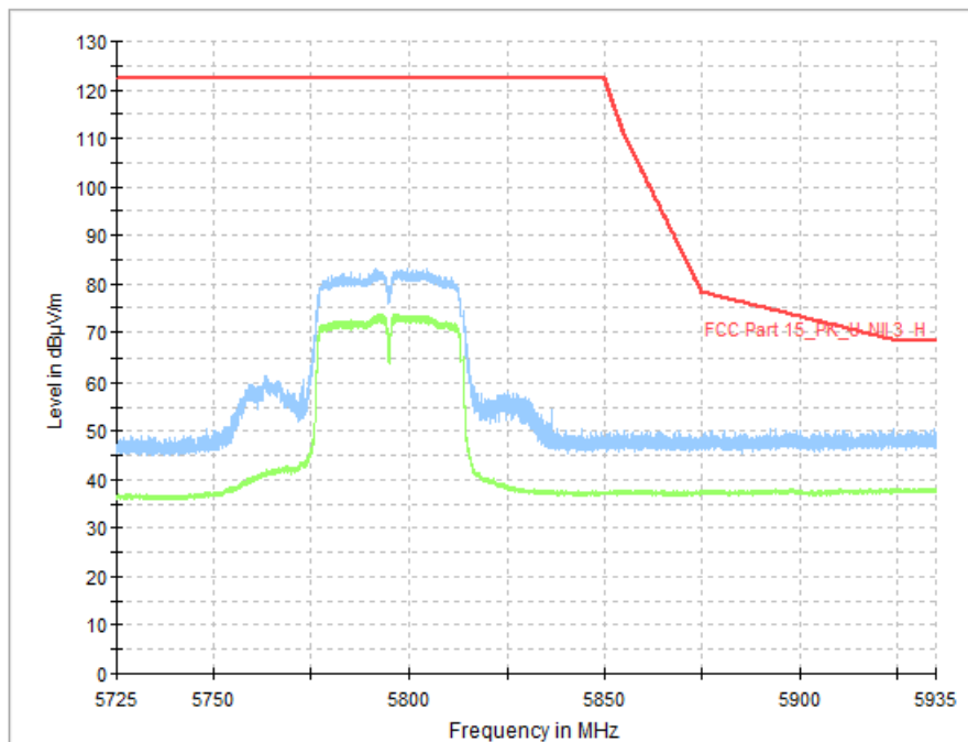
Fig. 38 Band Edges (802.11n-HT40, CH159 5795MHz)
