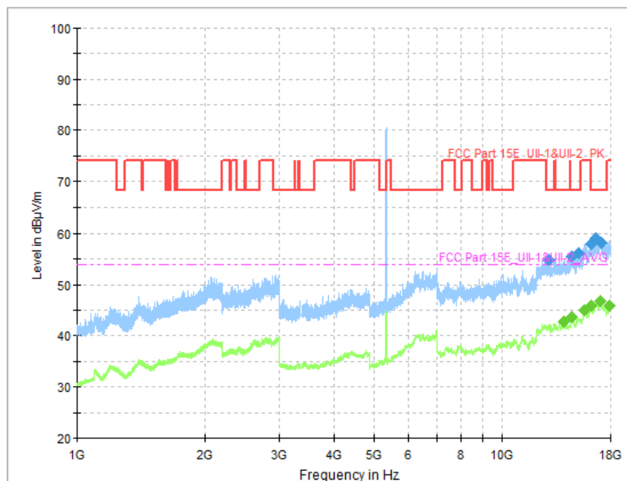
Fig. 47 Transmitter Spurious Emission (802.11a, CH64 5320MHz)
