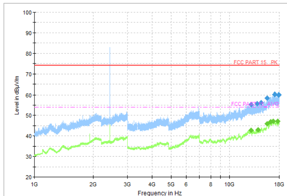
Fig. 43 Radiated Spurious Emission (GFSK, Ch39, 1GHz ~ 18GHz)
