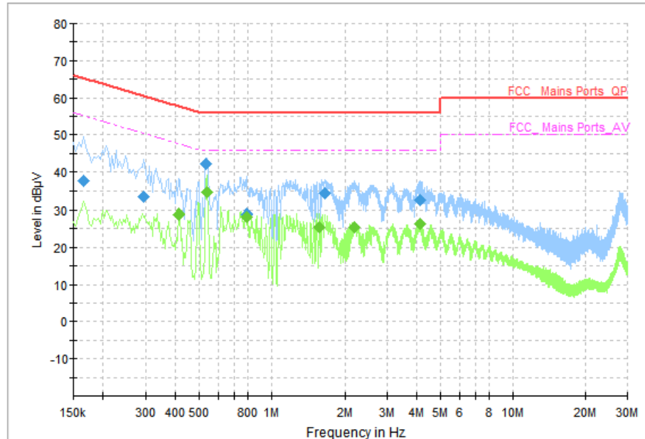
Figure B.10 Conducted Emission(Set.4, FM Mode)
