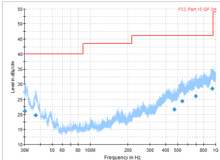
Figure A.25 Radiated Emission (Set.2, Charging and GSM850MHz idle, 30MHz to 1GHz) Final_Result
