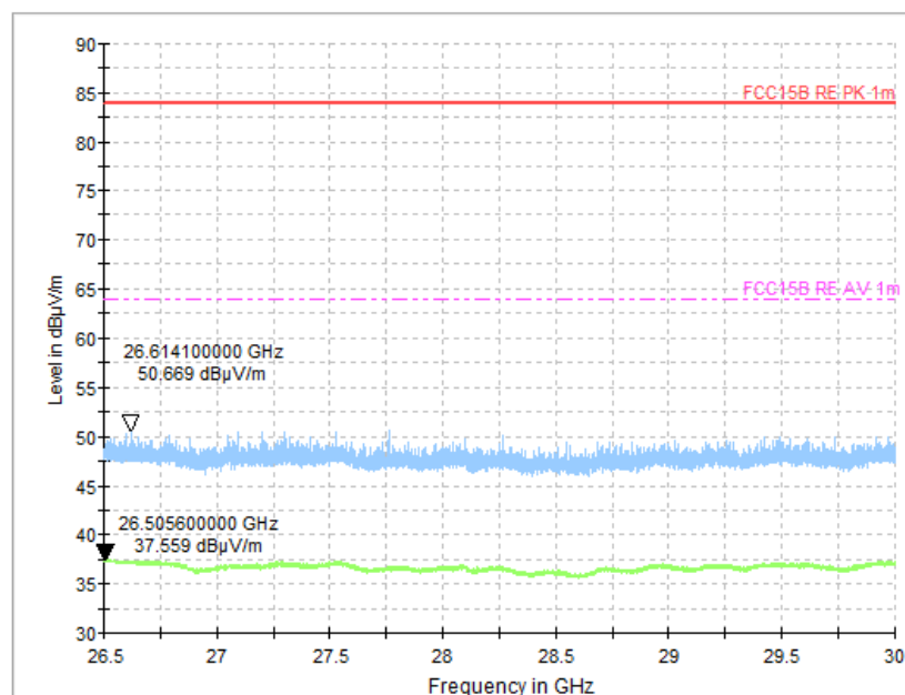
Figure A.28 Radiated Emission (Set.2, Charging and GSM850MHz idle , 26.5GHz to 30GHz)
