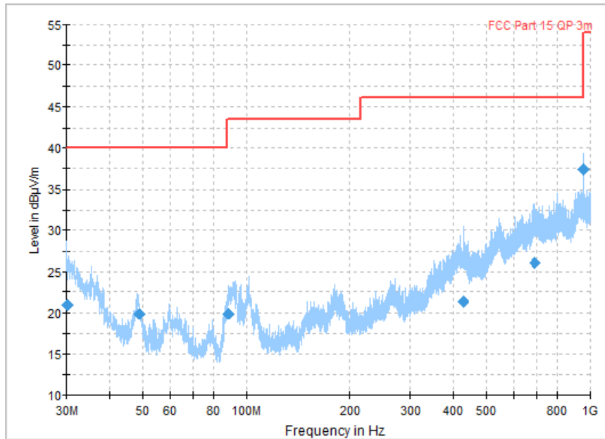
Figure A.21 Radiated Emission (Set.1, Charging and LTE Band 17 idle, 30MHz to 1GHz) Final_Result
