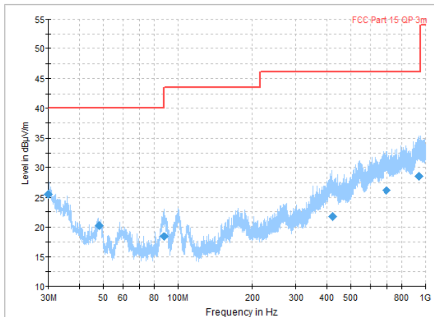
Figure A.33 Radiated Emission (Set.2, Charging and LTE Band 5 idle, 30MHz to 1GHz) Final_Result
