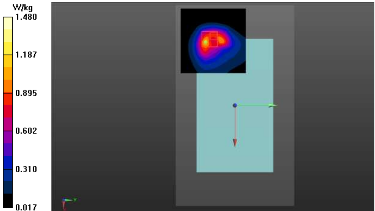
Fig.5 WCDMA Band 5 Body
