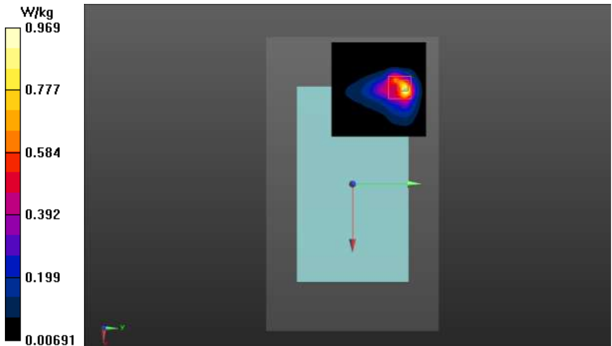
Fig.3 WLAN 2.4G Body
