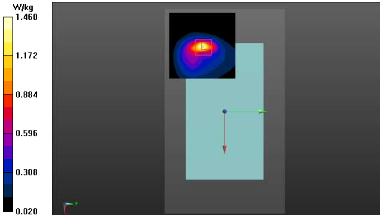
Fig.1 LTE Band 17 Body
