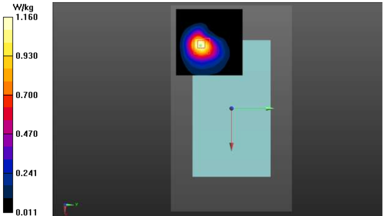
Fig.2 LTE Band 66 Body
