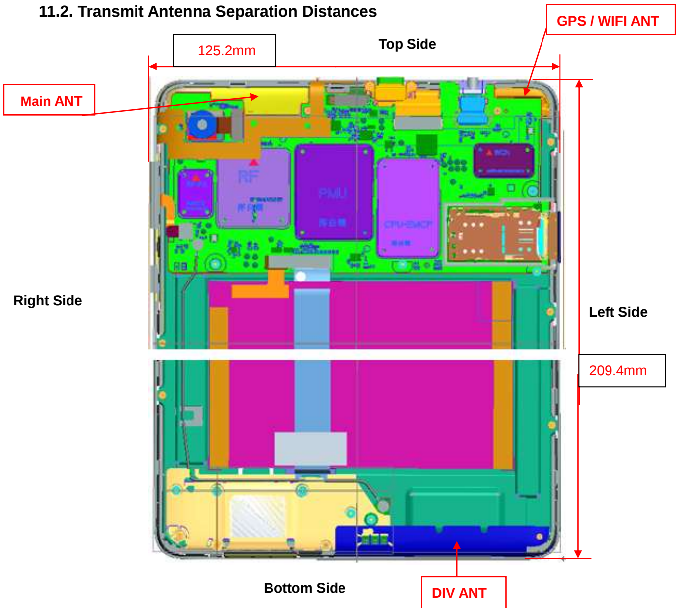
Picture 11.1 Antenna Locations (Back View)
