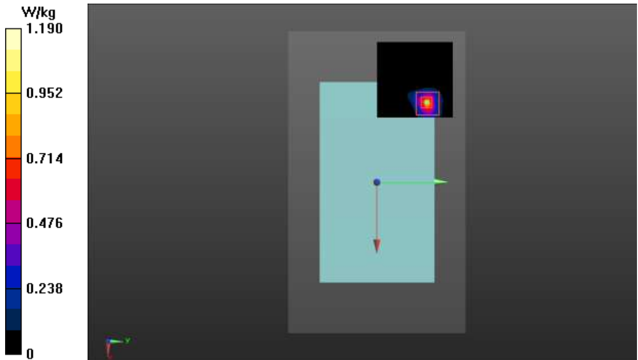
Fig.4 WLAN 5G Body
