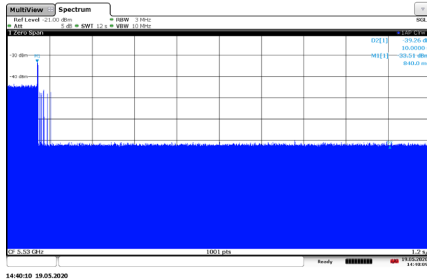
Fig.A.4 Channel move time
