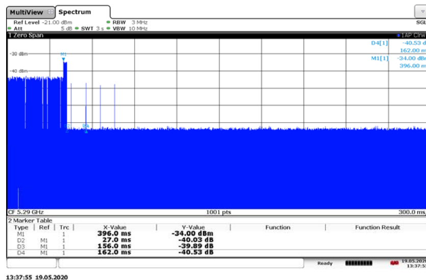
Fig.A.3 channel closing transmission time
