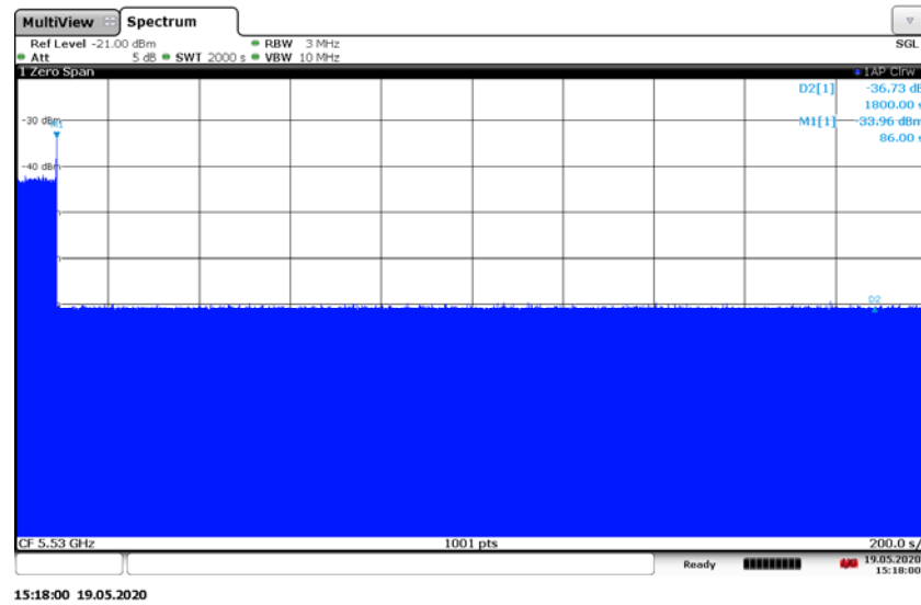
Fig.A.7 Non-Occupancy Period
