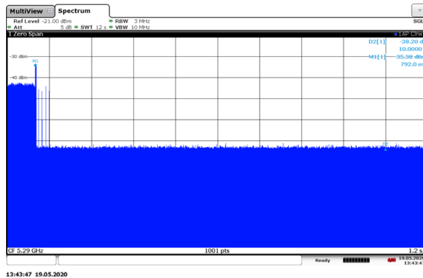
Fig.A.2 Channel move time
