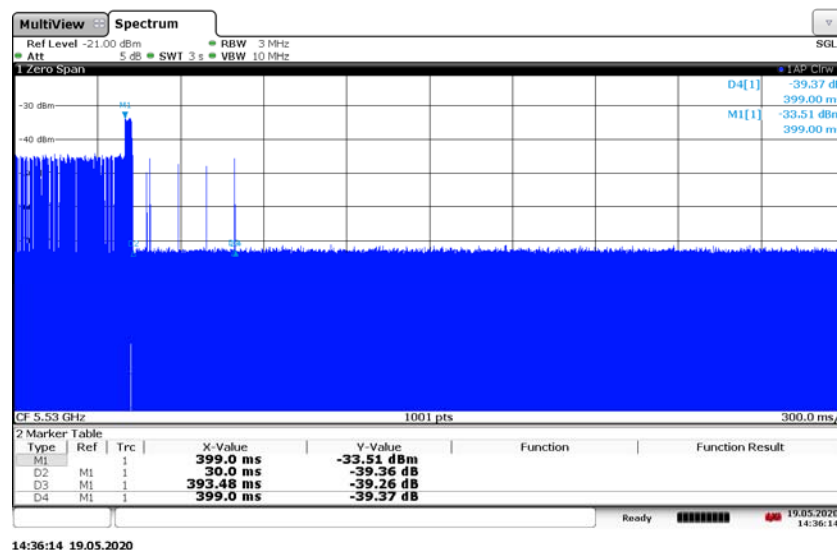
Fig.A.5 channel closing transmission time
