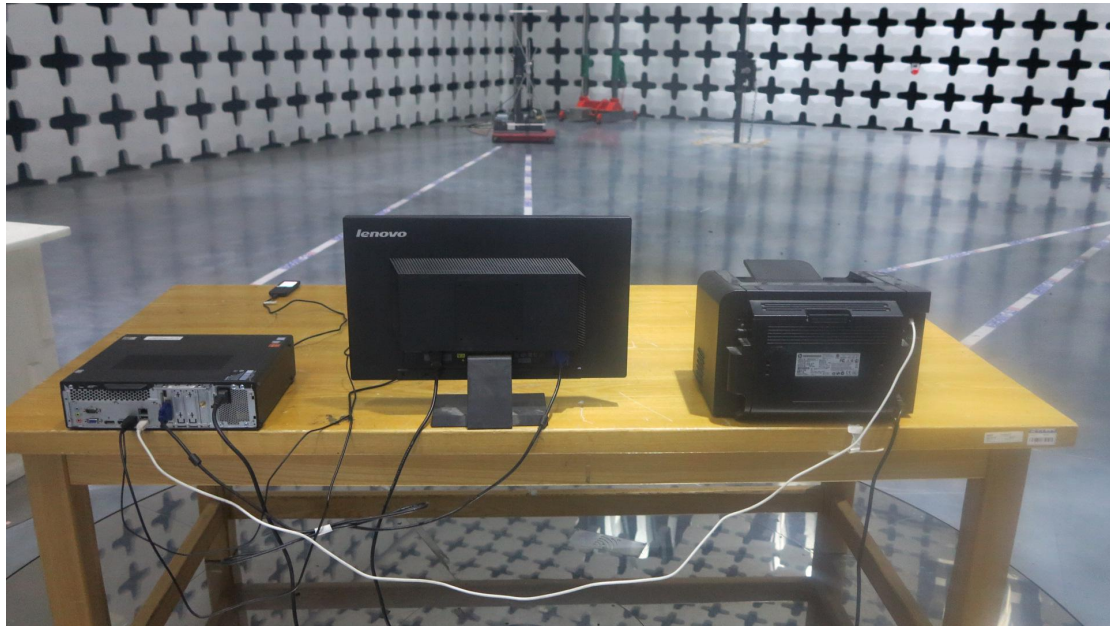
Part15b
