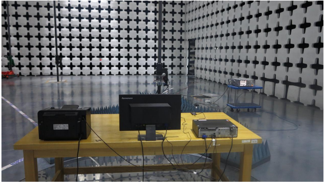
Spurious Emission
