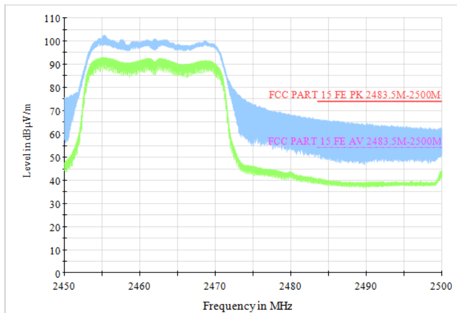
Fig.68 Radiated Restricted Band (802.11n HT20, CH11, 2.45GHz~2.5GHz)
