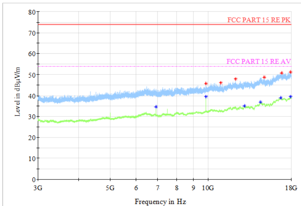
Fig.50 Radiated Spurious Emission (802.11b, CH11, 3GHz-18GHz)
