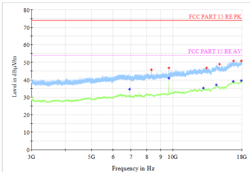
Fig.62 Radiated Spurious Emission (802.11n HT20, CH1, 3GHz-18GHz)
