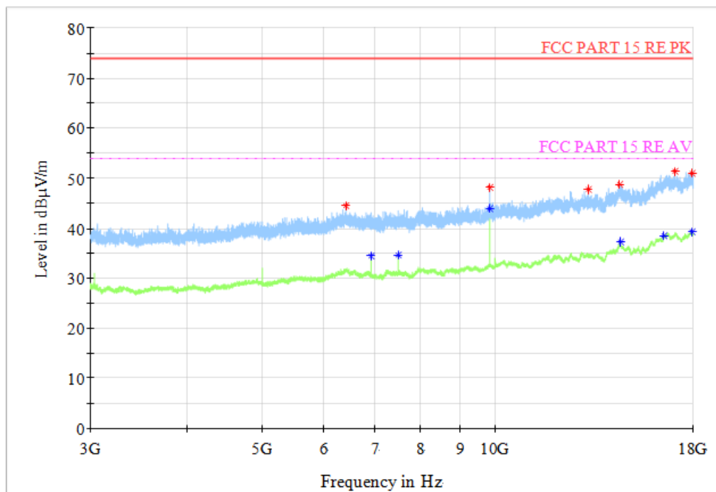
Fig.66 Radiated Spurious Emission (802.11n HT20, CH11, 3GHz-18GHz)
