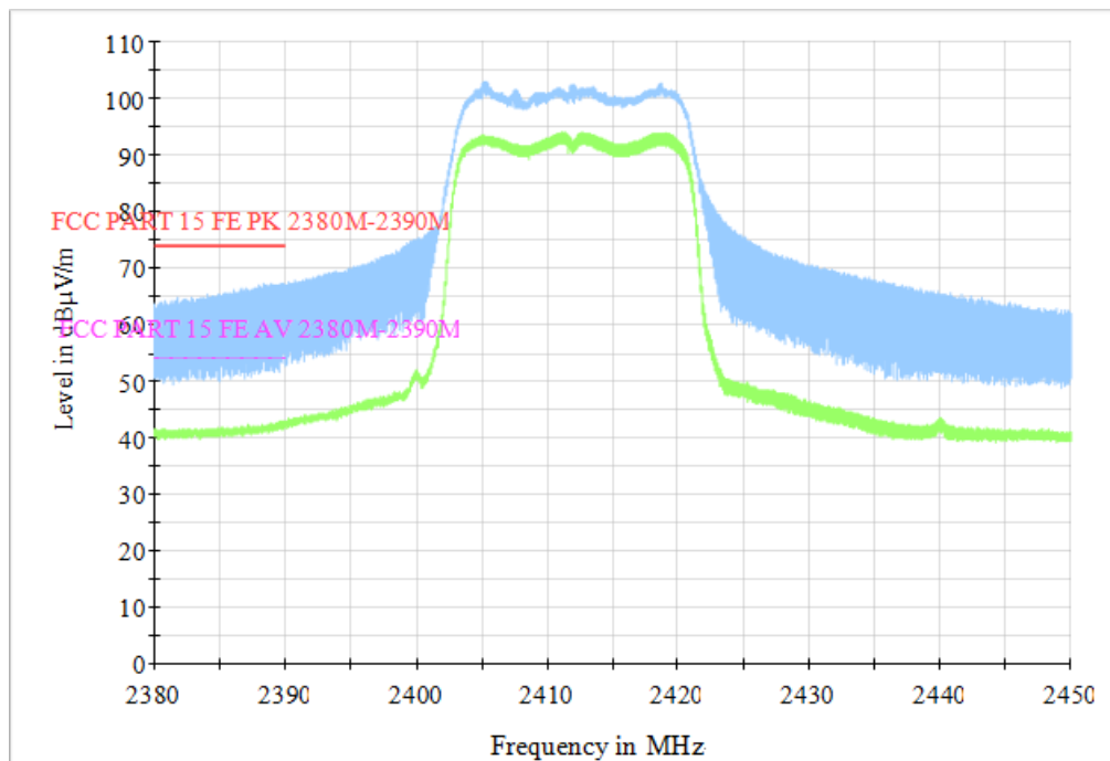
Fig.67 Radiated Restricted Band (802.11n HT20, CH1, 2.38GHz~2.45GHz)
