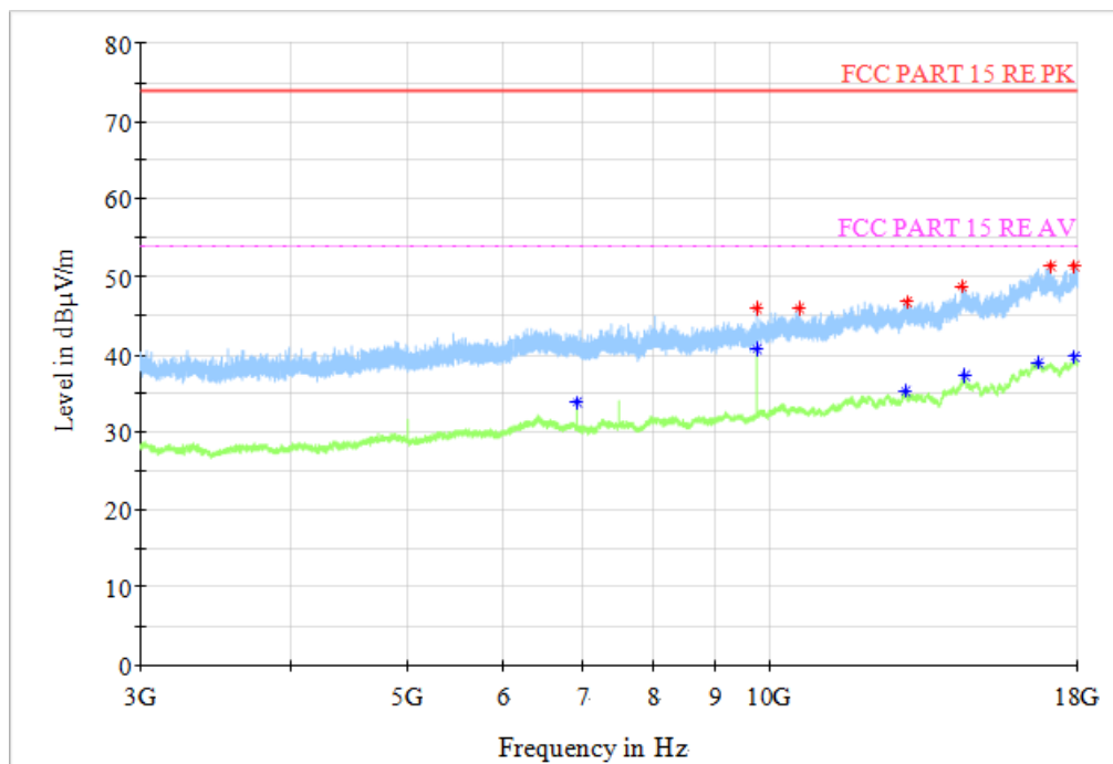
Fig.48 Radiated Spurious Emission (802.11b, CH6, 3GHz-18GHz)
