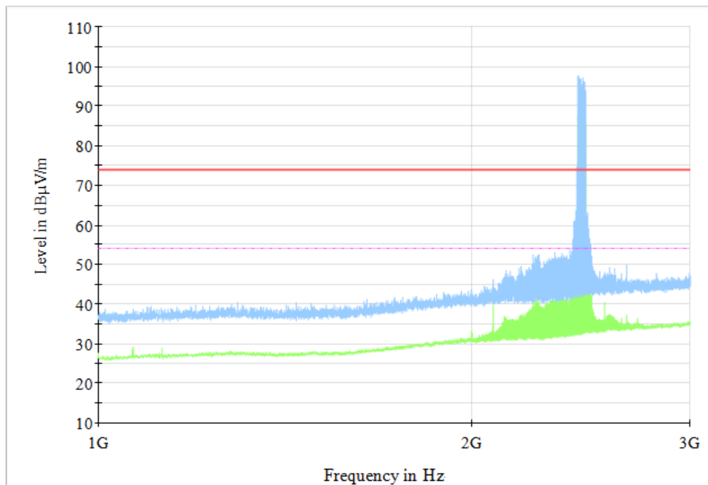
Fig.73 Radiated Spurious Emission (802.11n HT40, CH9, 1GHz-3GHz)
