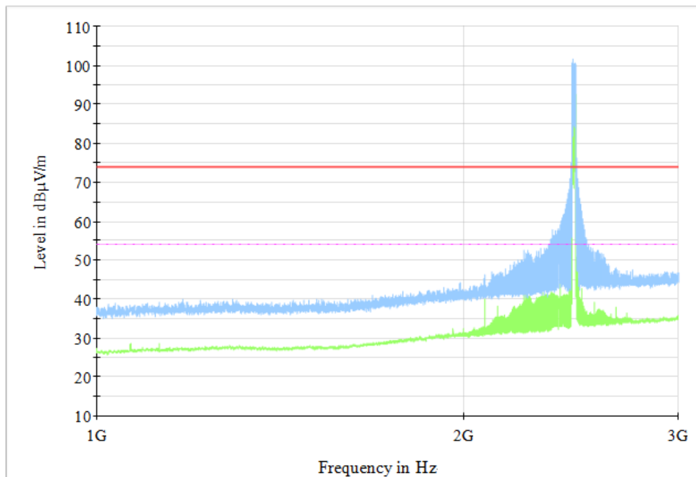
Fig.65 Radiated Spurious Emission (802.11n HT20, CH11, 1GHz-3GHz)
