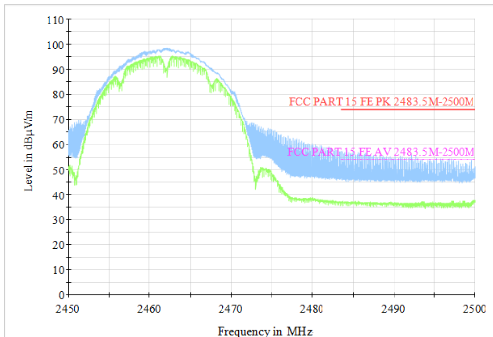
Fig.52 Radiated Restricted Band (802.11b, CH11, 2.45GHz~2.5GHz)
