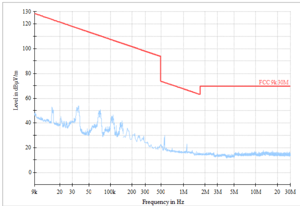
Fig.77 Radiated Spurious Emission (All Channels, 9KHz-30MHz)
