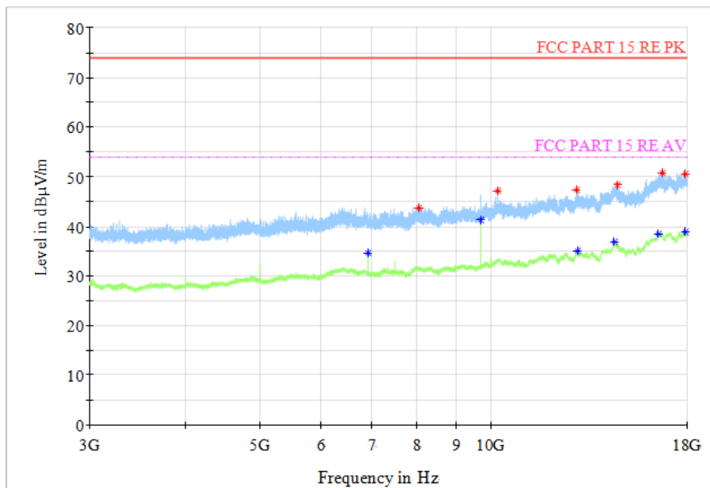
Fig.70 Radiated Spurious Emission (802.11n HT40, CH3, 3GHz-18GHz)
