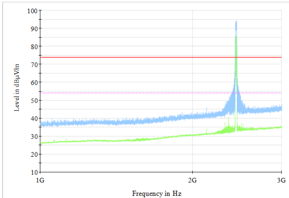
Fig.55 Radiated Spurious Emission (802.11g, CH6, 1GHz-3GHz)
