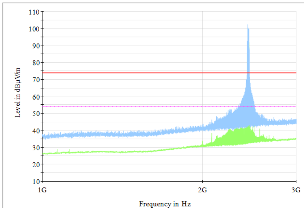
Fig.63 Radiated Spurious Emission (802.11n HT20, CH6, 1GHz-3GHz)
