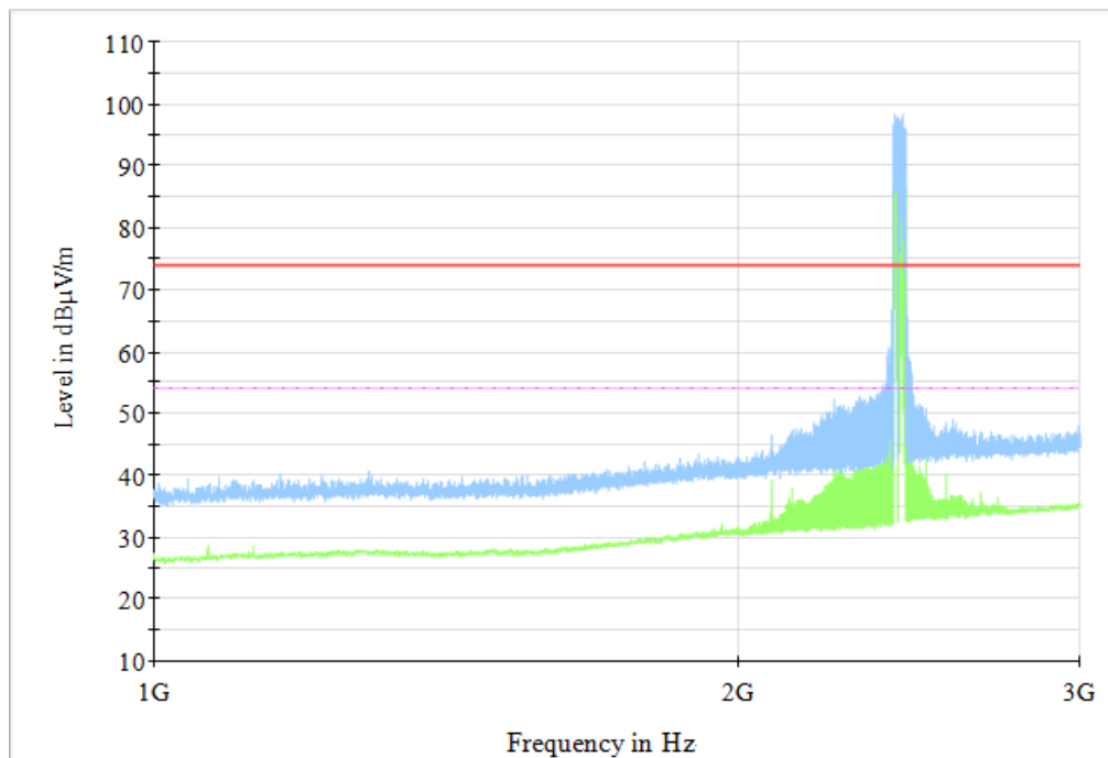
Fig.69 Radiated Spurious Emission (802.11n HT40, CH3, 1GHz-3GHz)
