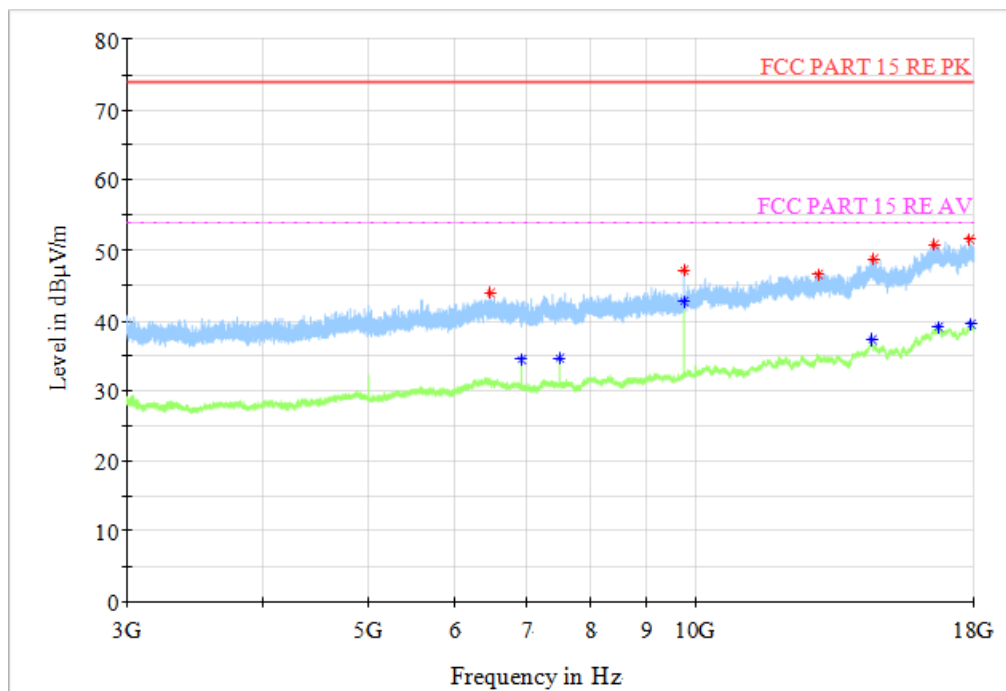
Fig.64 Radiated Spurious Emission (802.11n HT20, CH6, 3GHz-18GHz)
