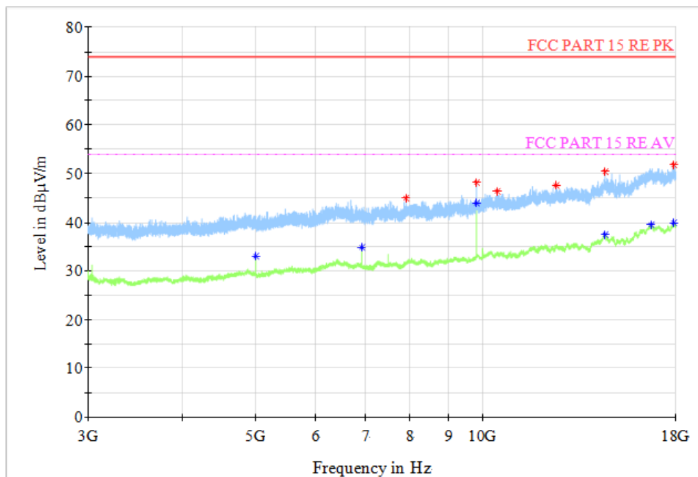
Fig.74 Radiated Spurious Emission (802.11n HT40, CH9, 3GHz-18GHz)
