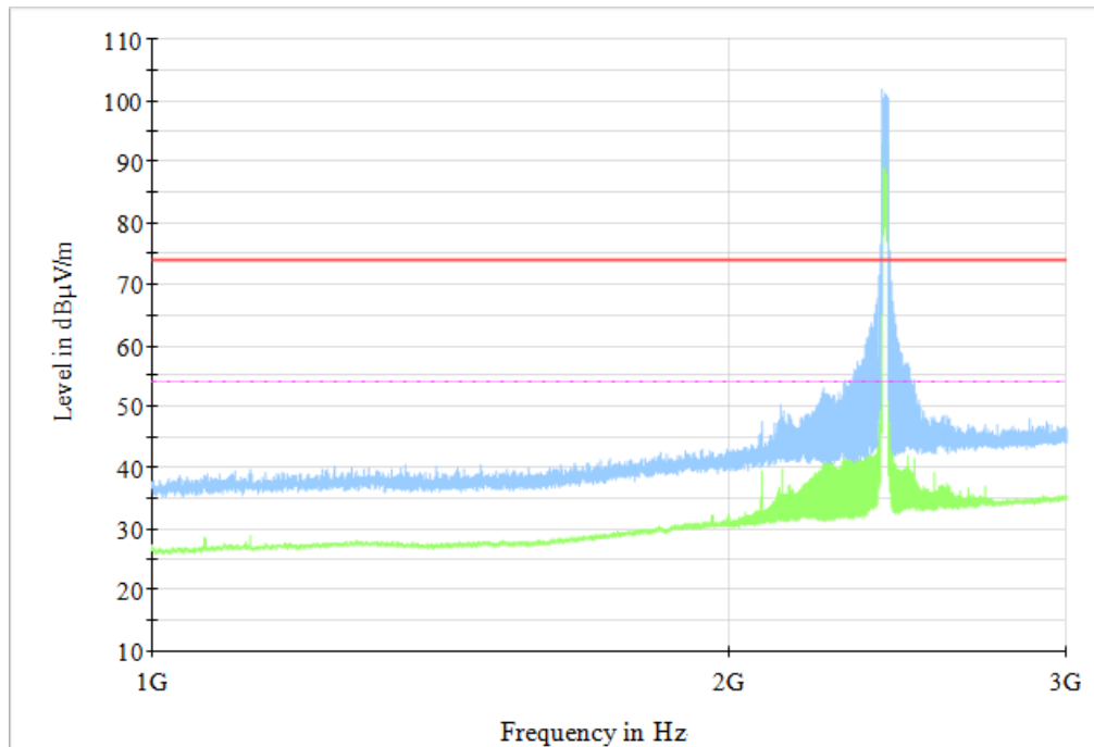
Fig.61 Radiated Spurious Emission (802.11n HT20, CH1, 1GHz-3GHz)
