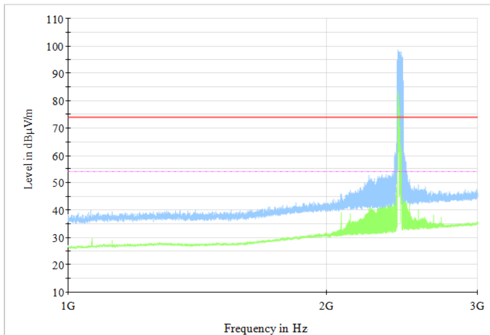
Fig.71 Radiated Spurious Emission (802.11n HT40, CH6, 1GHz-3GHz)
