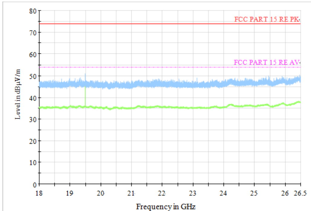
Fig.7.79 Radiated Spurious Emission (All Channels, 18GHz-26.5GHz)
