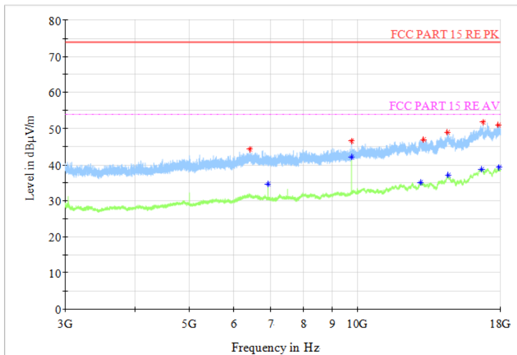
Fig.72 Radiated Spurious Emission (802.11n HT40, CH6, 3GHz-18GHz)
