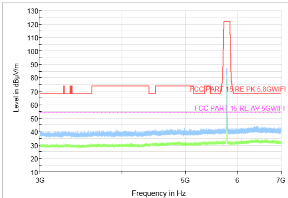
Fig. 79 Transmitter Spurious Emission (802. 11 n-HT20, CH157 5785MHz, 3 GHz-7 GHz), MIMO
