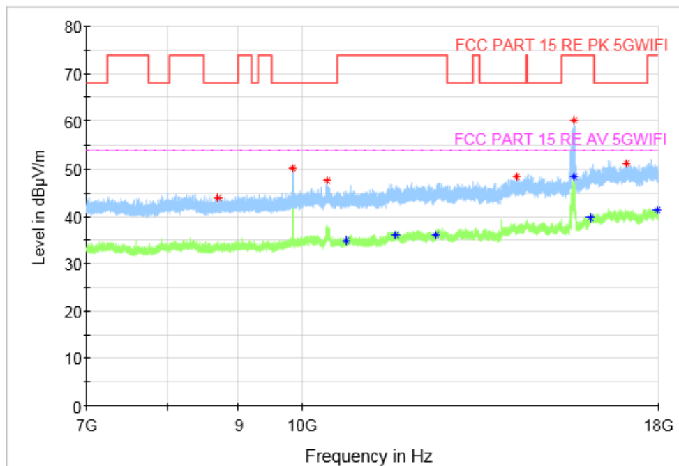
Fig. 59 Transmitter Spurious Emission (802. 11ac-VHT80, CH42 5210MHz, 7 GHz-18 GHz), SISO
