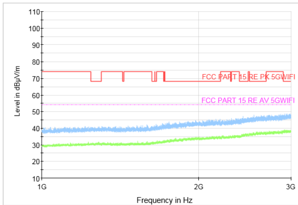
Fig. 57 Transmitter Spurious Emission (802.11ac-VHT80, CH42 5210MHz, 1 GHz-3 GHz), SISO
