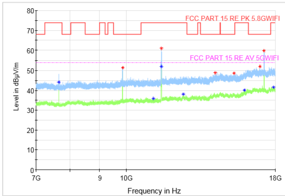
Fig. 77 Transmitter Spurious Emission (802. 11 n-HT20, CH149 5745MHz, 7 GHz-18 GHz), MIMO
