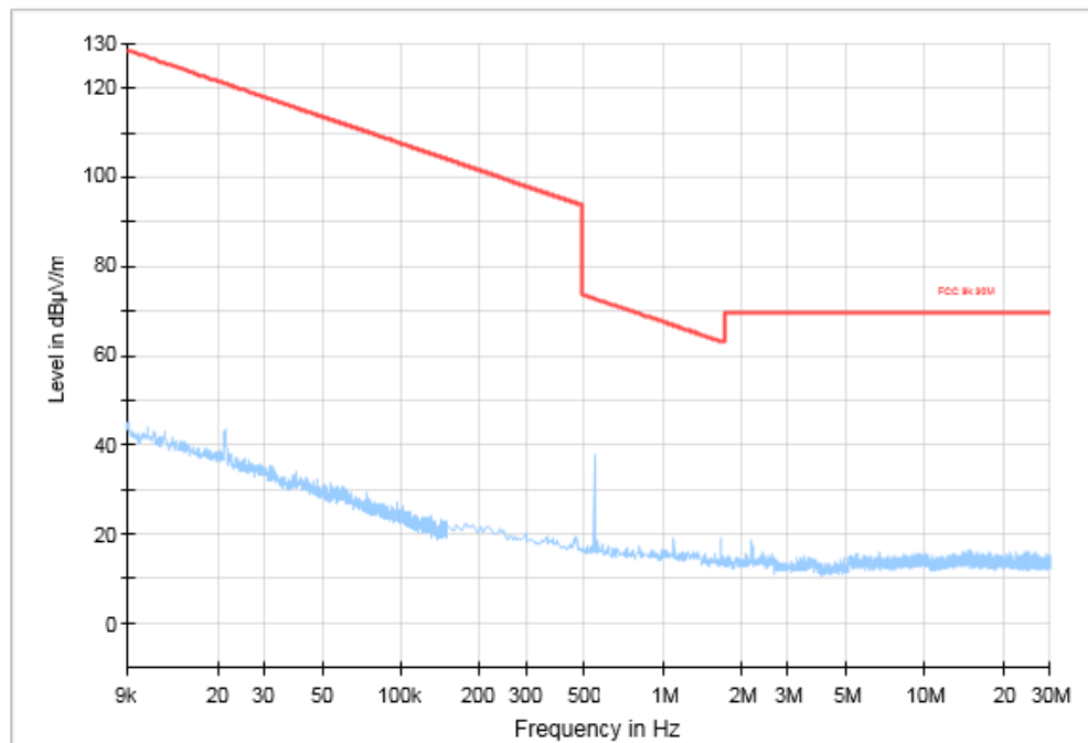
Fig. 112 Radiated Spurious Emission (All Channel, 9 kHz ~30 MHz),MIMO
