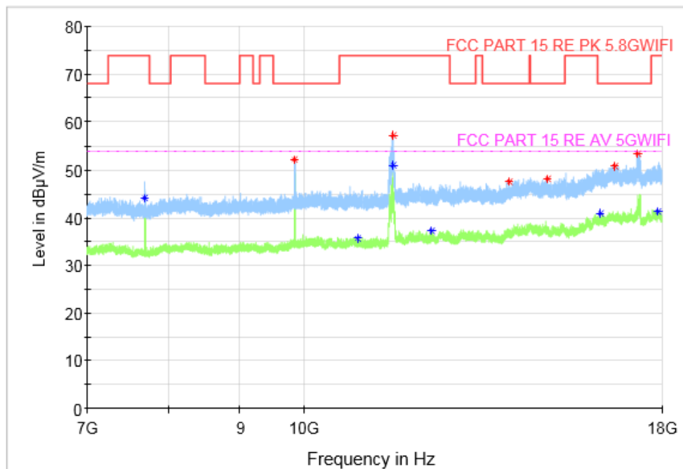
Fig. 101 Transmitter Spurious Emission (802.11ac-VHT80, CH155 5775MHz, 7 GHz-18 GHz), MIMO
