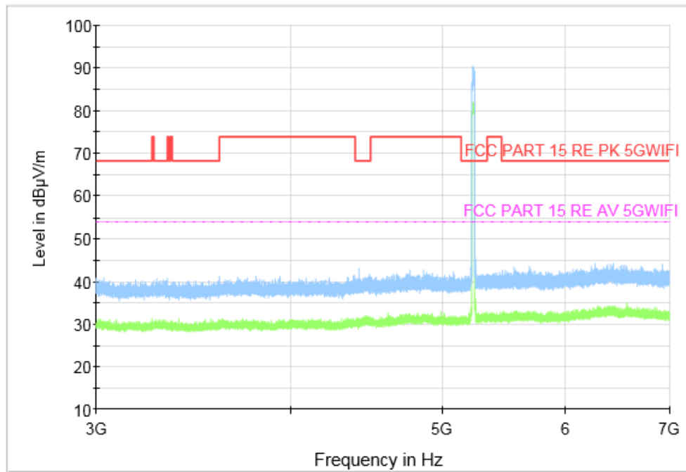
Fig. 73 Transmitter Spurious Emission (802.11 n-HT20, CH48 5240MHz, 3 GHz-7 GHz), MIMO
