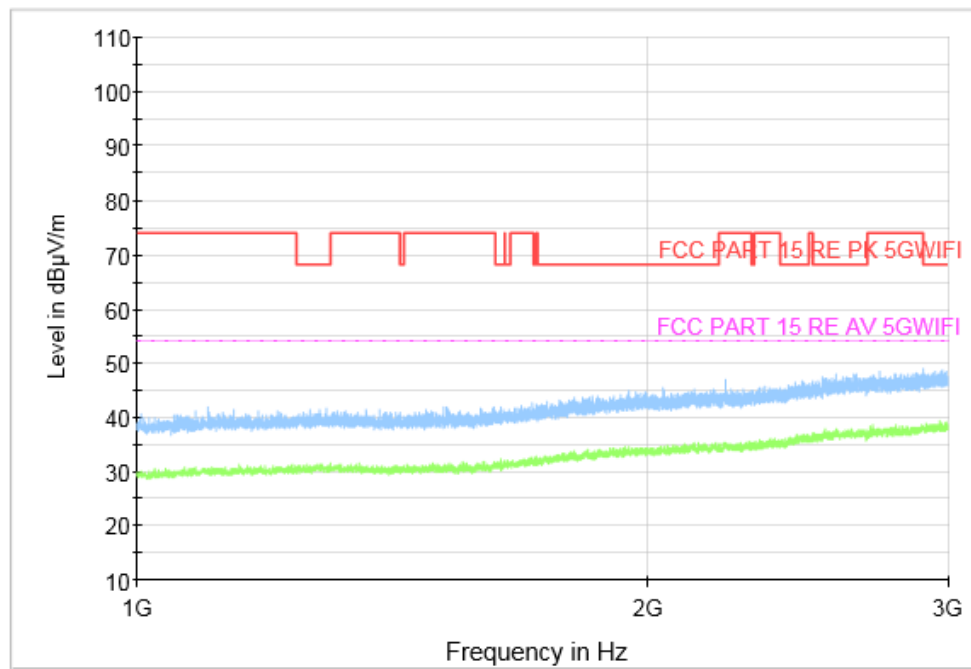
Fig. 87 Transmitter Spurious Emission (802.11n-HT40, CH46 5230MHz, 1 GHz-3 GHz), MIMO
