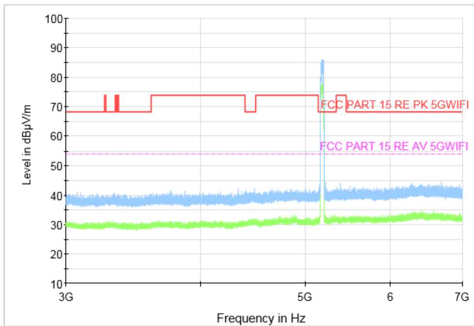
Fig. 85 Transmitter Spurious Emission (802.11n-HT40, CH38 5190MHz, 3 GHz-7 GHz), MIMO
