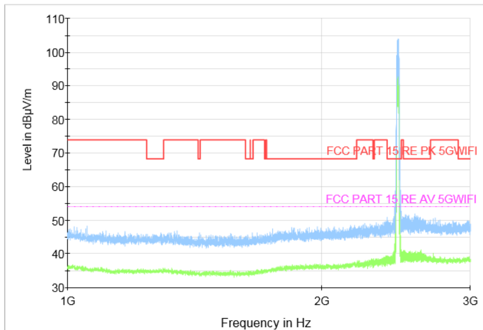
Fig. 106 Transmitter Spurious Emission (Co-located, 1 GHz-3 GHz)
