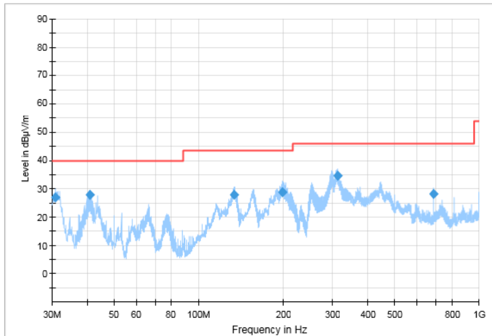
Fig. 63 Transmitter Spurious Emission (All channel, 30MHz~1GHz), SISO
