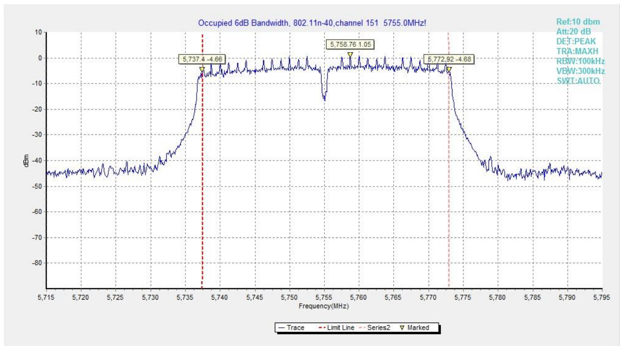
Fig. 10 Occupied 6dB Bandwidth (802.11n-HT40, 5755MHz)
