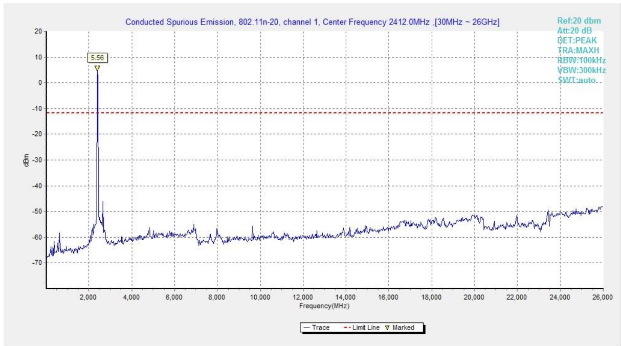
Fig.45 Conducted Spurious Emission (802.11n HT20, CH1), MIMO
