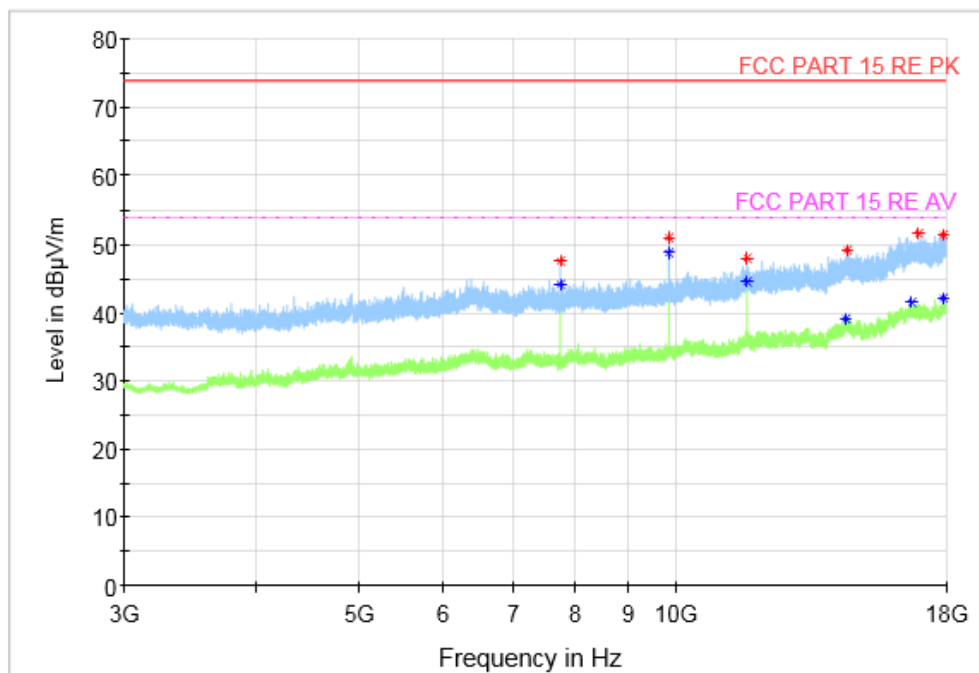
Fig.72 Radiated Spurious Emission (802.11n HT20, CH11, 3 GHz-18 GHz), SISO
