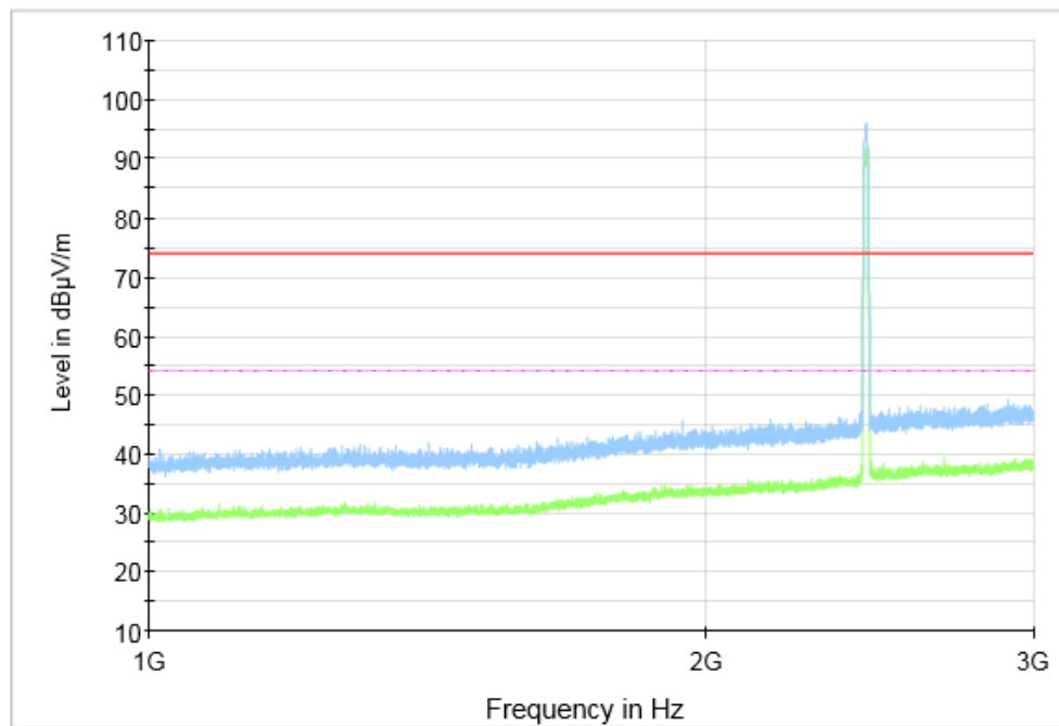
Fig.53 Radiated Spurious Emission (802.11b, CH6, 1 GHz-3GHz), SISO
