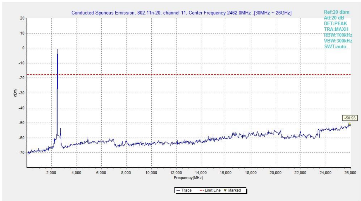
Fig.41 Conducted Spurious Emission (802.11n HT20, CH11), SISO
