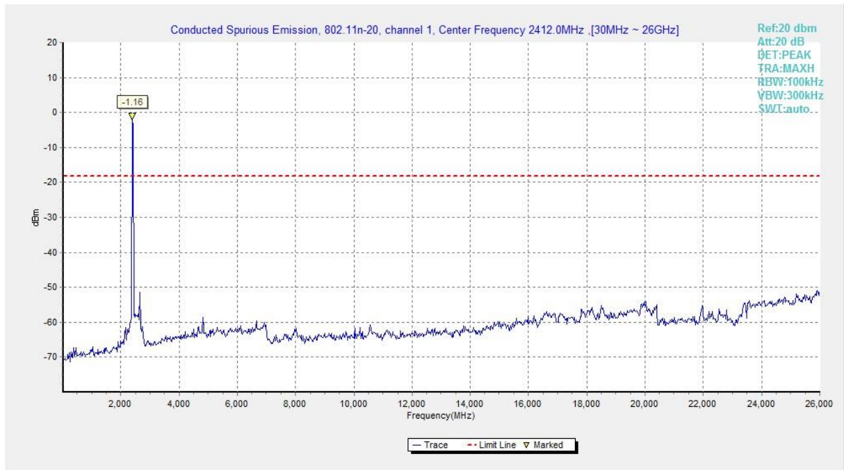
Fig.39 Conducted Spurious Emission (802.11n HT20, CH1), SISO
