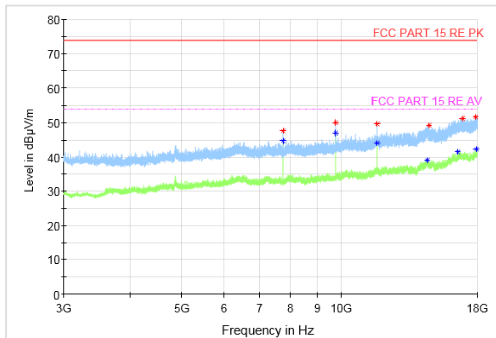
Fig.78 Radiated Spurious Emission (802.11n HT40, CH6, 3 GHz-18 GHz), SISO
