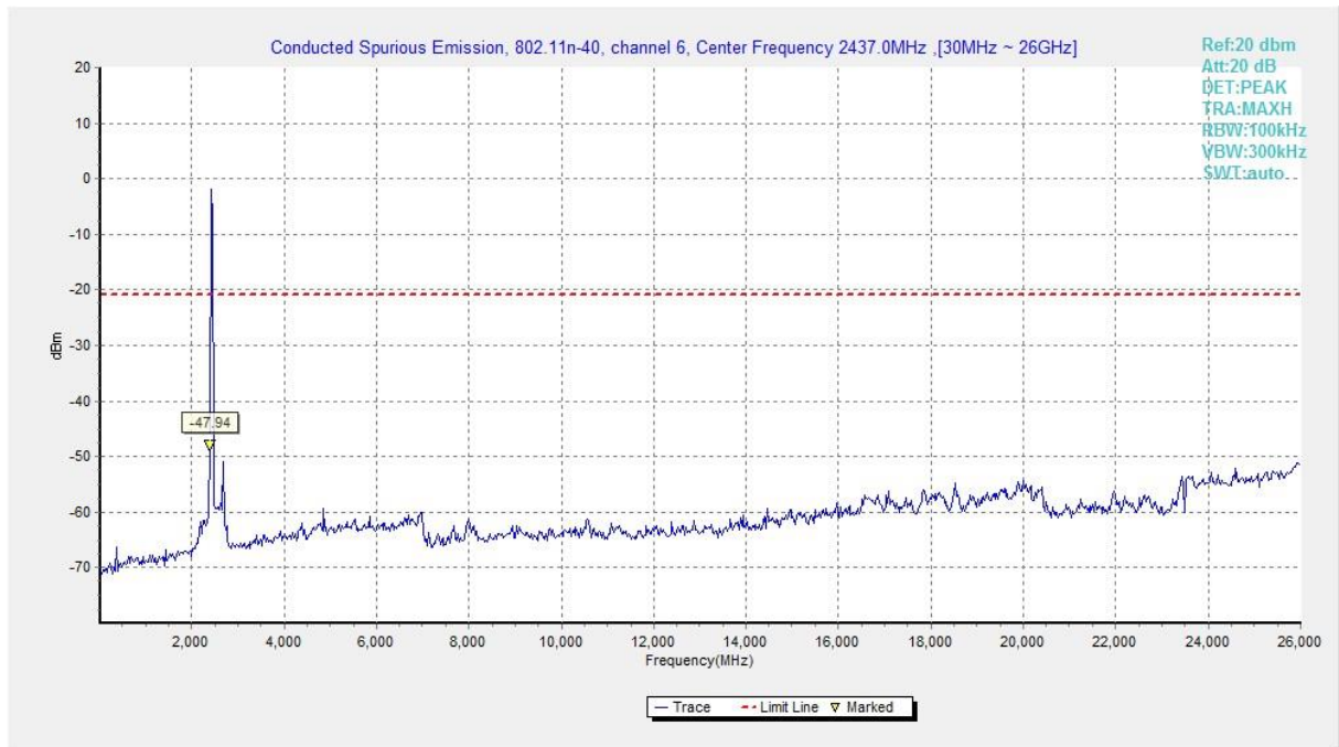
Fig.43 Conducted Spurious Emission (802.11n HT40, CH6), SISO
