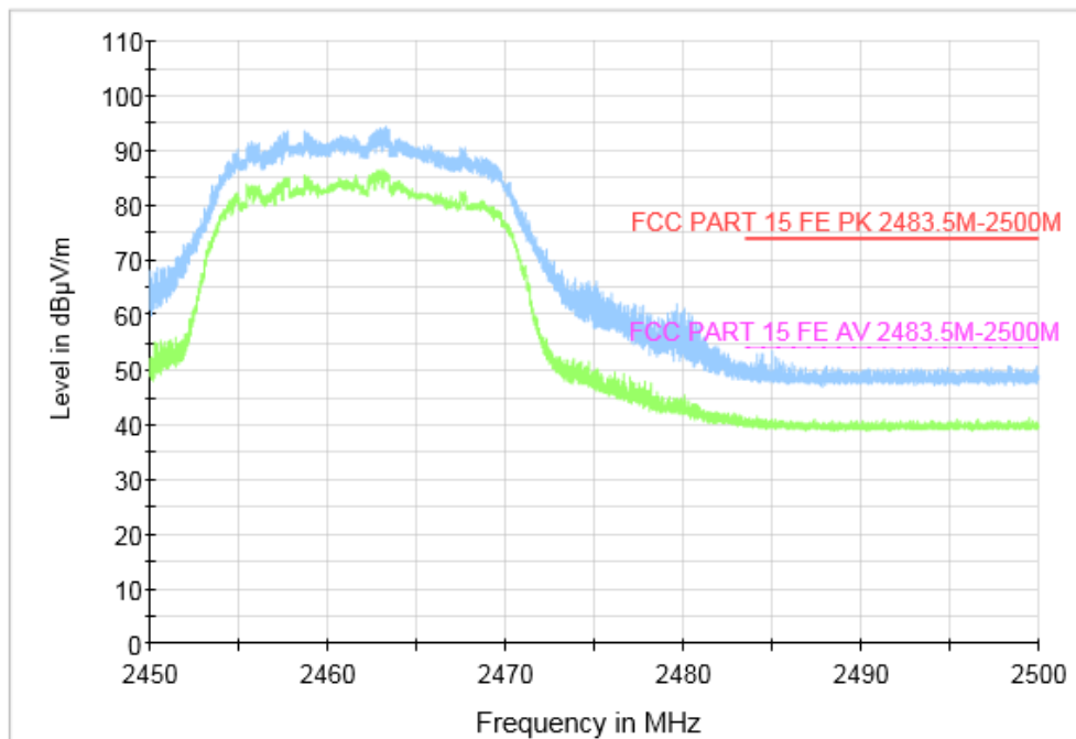
Fig.66 Radiated Restricted Band (802.11g, CH11, 2.45GHz~2.5GHz), SISO
