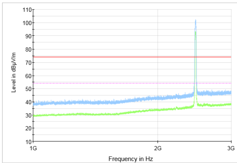
Fig.90 Radiated Spurious Emission (802.11n HT20, CH11, 1 GHz-3 GHz), MIMO
