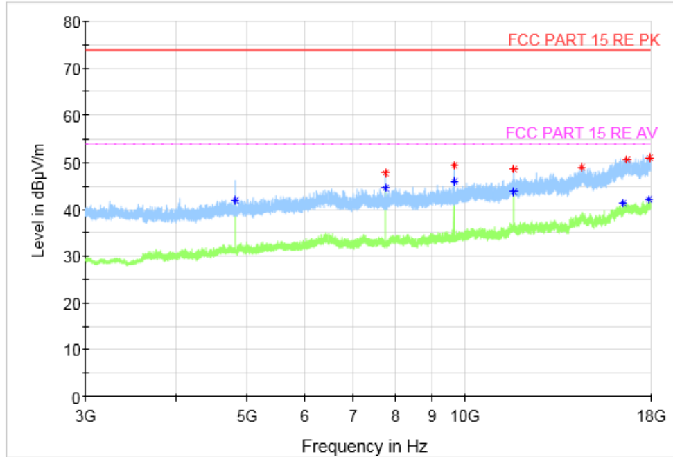
Fig.52 Radiated Spurious Emission (802.11b, CH1, 3 GHz-18GHz), SISO
