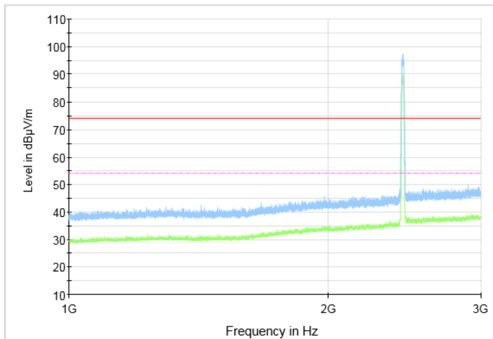
Fig.61 Radiated Spurious Emission (802.11g, CH6, 1 GHz-3 GHz), SISO
