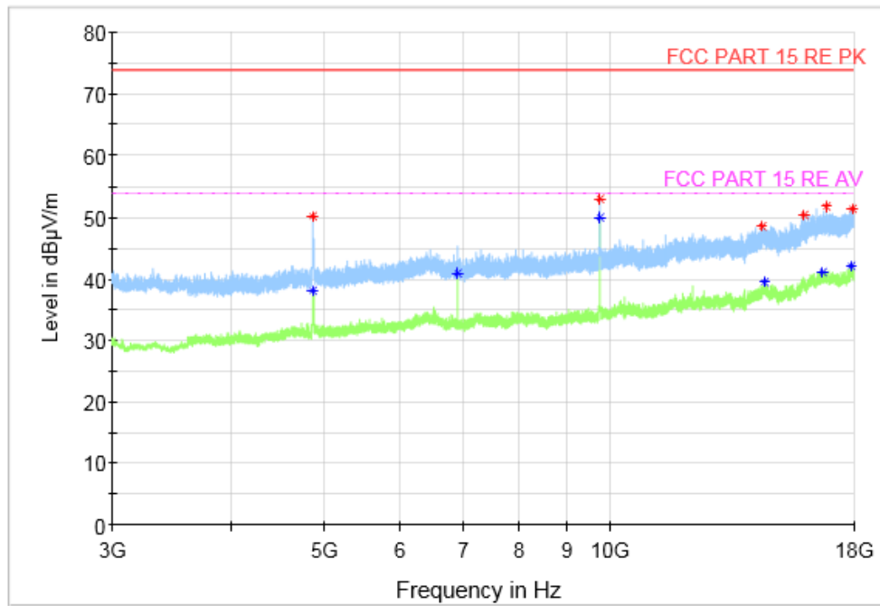
Fig.89 Radiated Spurious Emission (802.11n HT20, CH6, 3 GHz-18 GHz), MIMO
