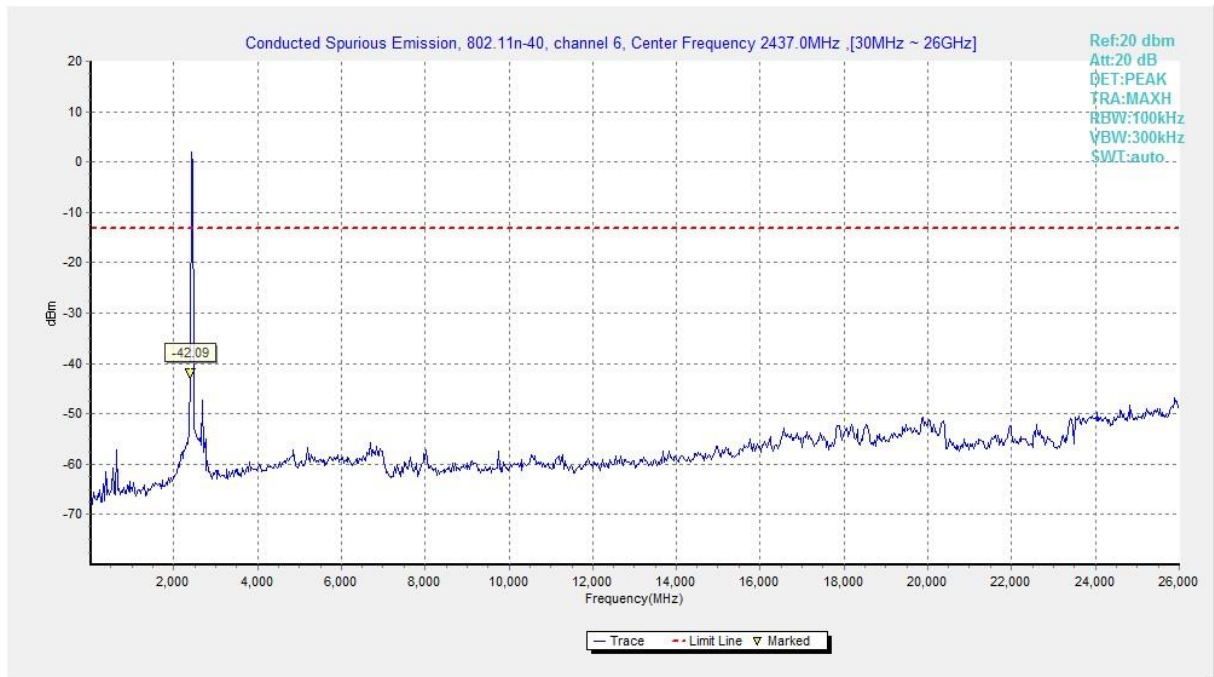
Fig.49 Conducted Spurious Emission (802.11n HT40, CH6), MIMO
