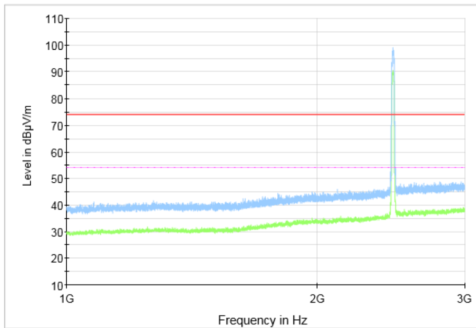
Fig.63 Radiated Spurious Emission (802.11g, CH11, 1 GHz-3 GHz), SISO
