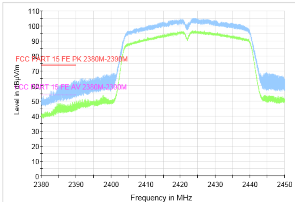
Fig.81 Radiated Restricted Band (802.11n HT40, CH3, 2.38GHz~2.45GHz), SISO
