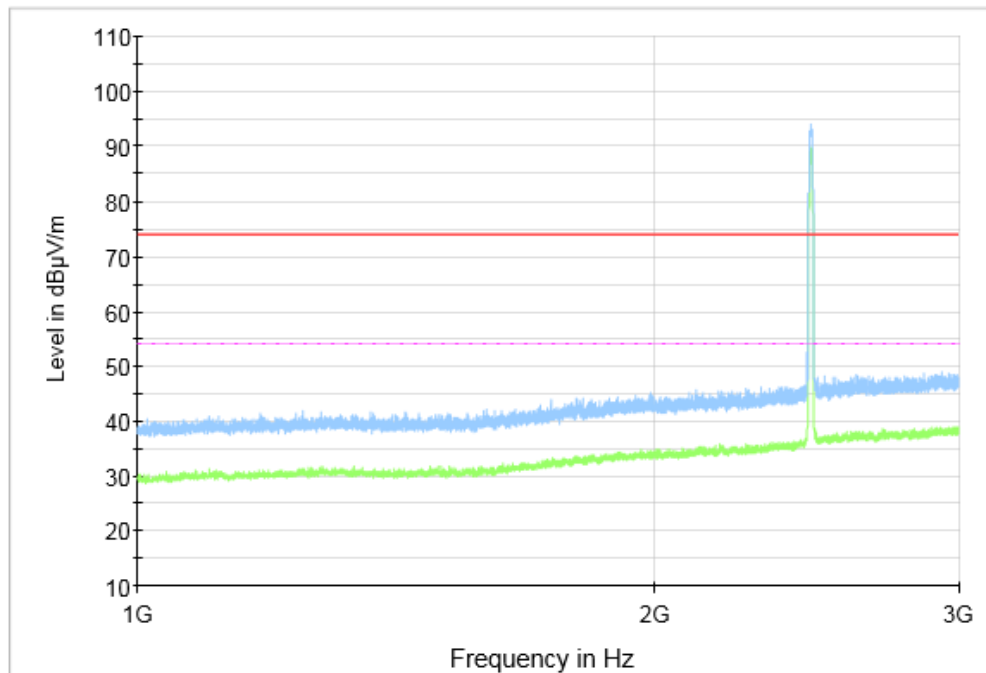
Fig.55 Radiated Spurious Emission (802.11b, CH11, 1 GHz-3GHz), SISO
