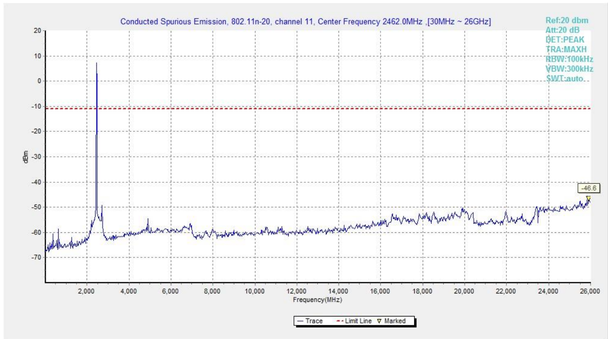
Fig.47 Conducted Spurious Emission (802.11n HT20, CH11), MIMO
