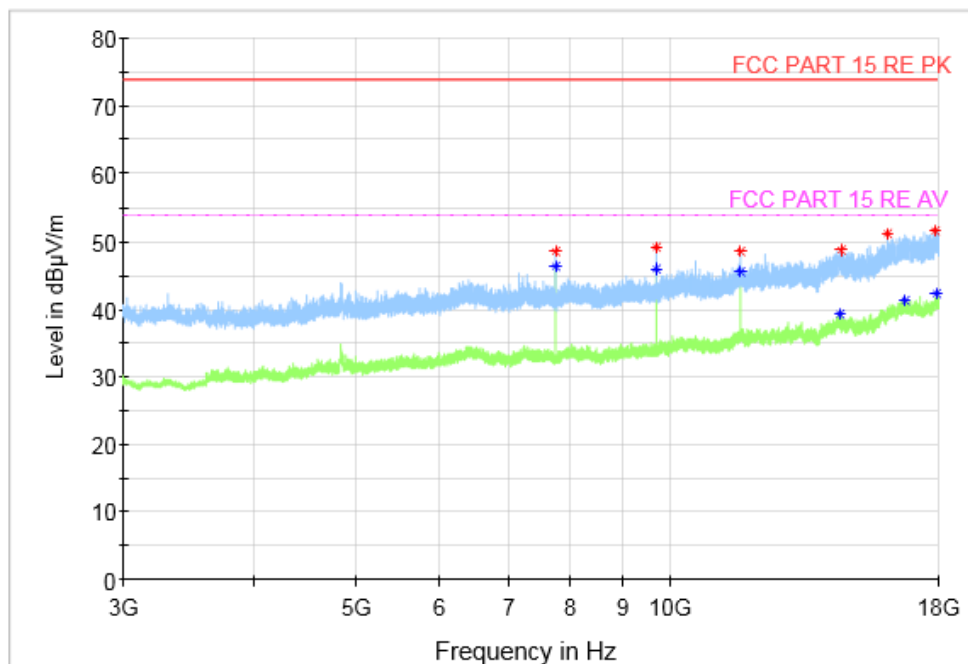
Fig.76 Radiated Spurious Emission (802.11n HT40, CH3, 3 GHz-18 GHz), SISO
