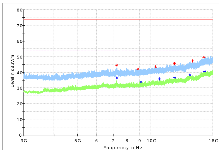
Fig.51 Radiated Spurious Emission (802.11n HT20, CH1, 3 GHz-18 GHz)
