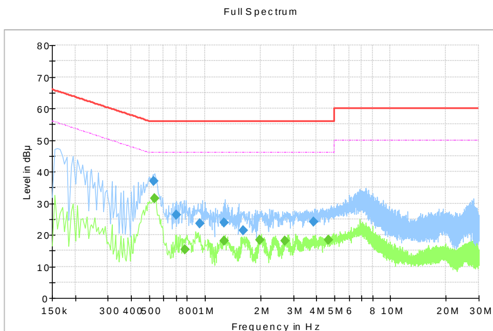
Fig.62 AC Power line Conducted Emission (Idle)
