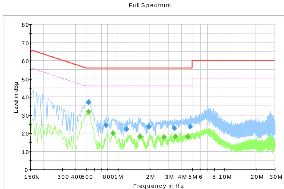
Fig.61 AC Power line Conducted Emission (Traffic)
