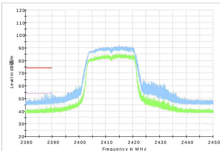
Fig.56 Radiated Restricted Band (802.11n HT20, CH1, 2.38GHz~2.45GHz)
