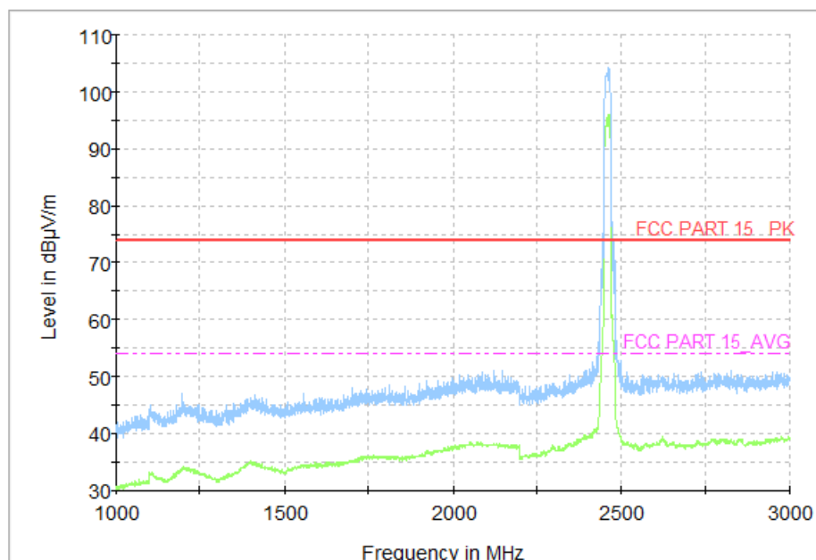
Fig.54 Radiated Spurious Emission (802.11n HT20, CH11, 1 GHz-3 GHz)
