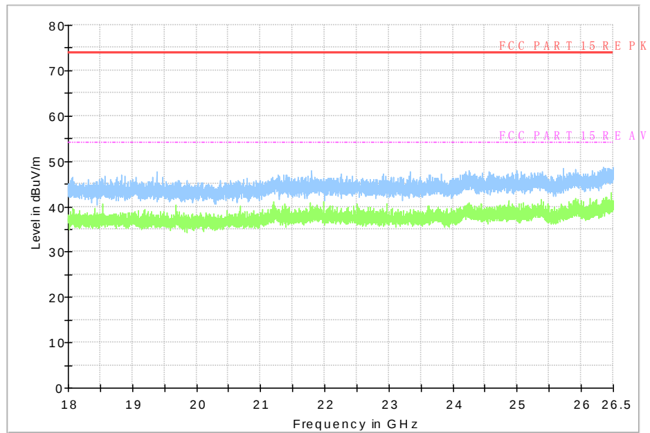
Fig.60 Radiated Spurious Emission (All Channels, 18 GHz-26.5 GHz)
