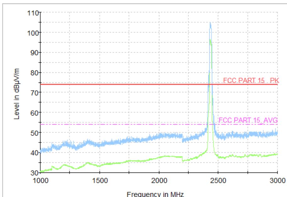
Fig.52 Radiated Spurious Emission (802.11n HT20, CH6, 1 GHz-3 GHz)
