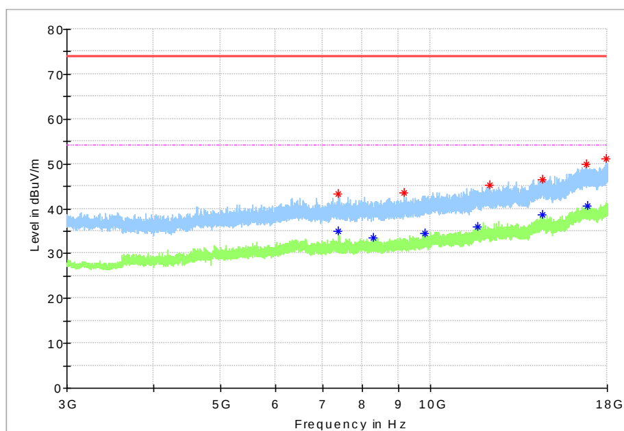
Fig.55 Radiated Spurious Emission (802.11n HT20, CH11, 3 GHz-18 GHz)
