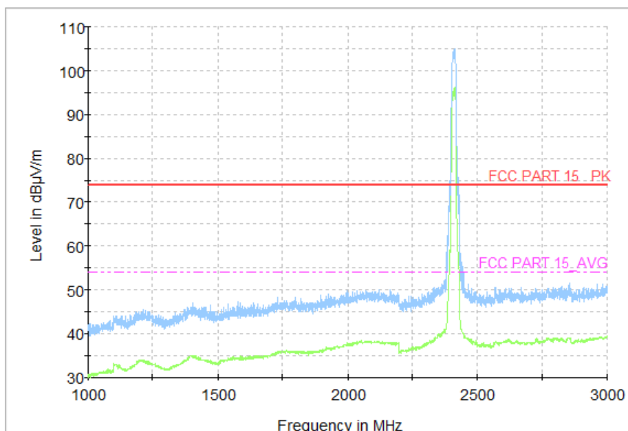
Fig.50 Radiated Spurious Emission (802.11n HT20, CH1, 1 GHz-3 GHz)
