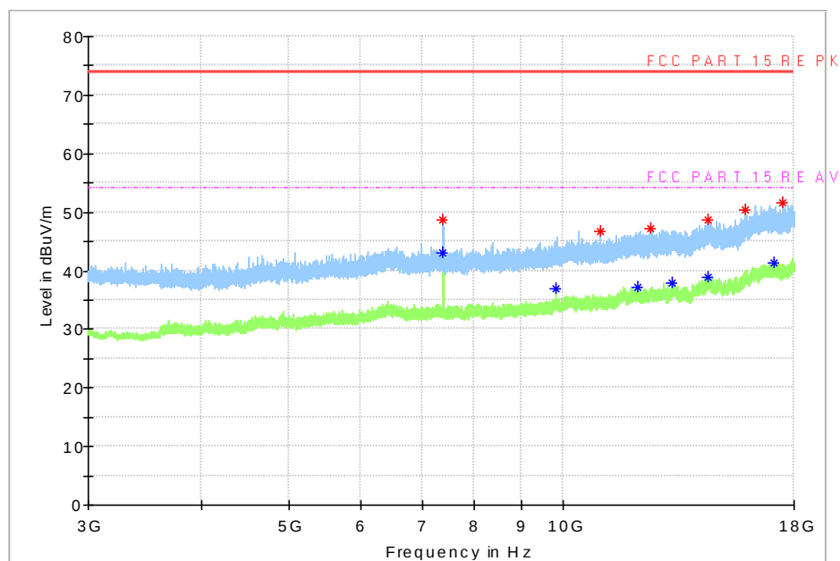
Fig.39 Radiated Spurious Emission (802.11b, CH11, 3 GHz-18GHz)
