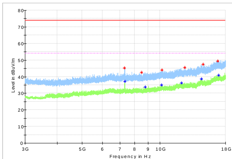
Fig.53 Radiated Spurious Emission (802.11n HT20, CH6, 3 GHz-18 GHz)
