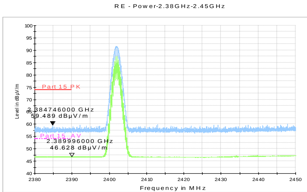
Fig.60. Radiated emission (Power): π/4 DQPSK, low channel
