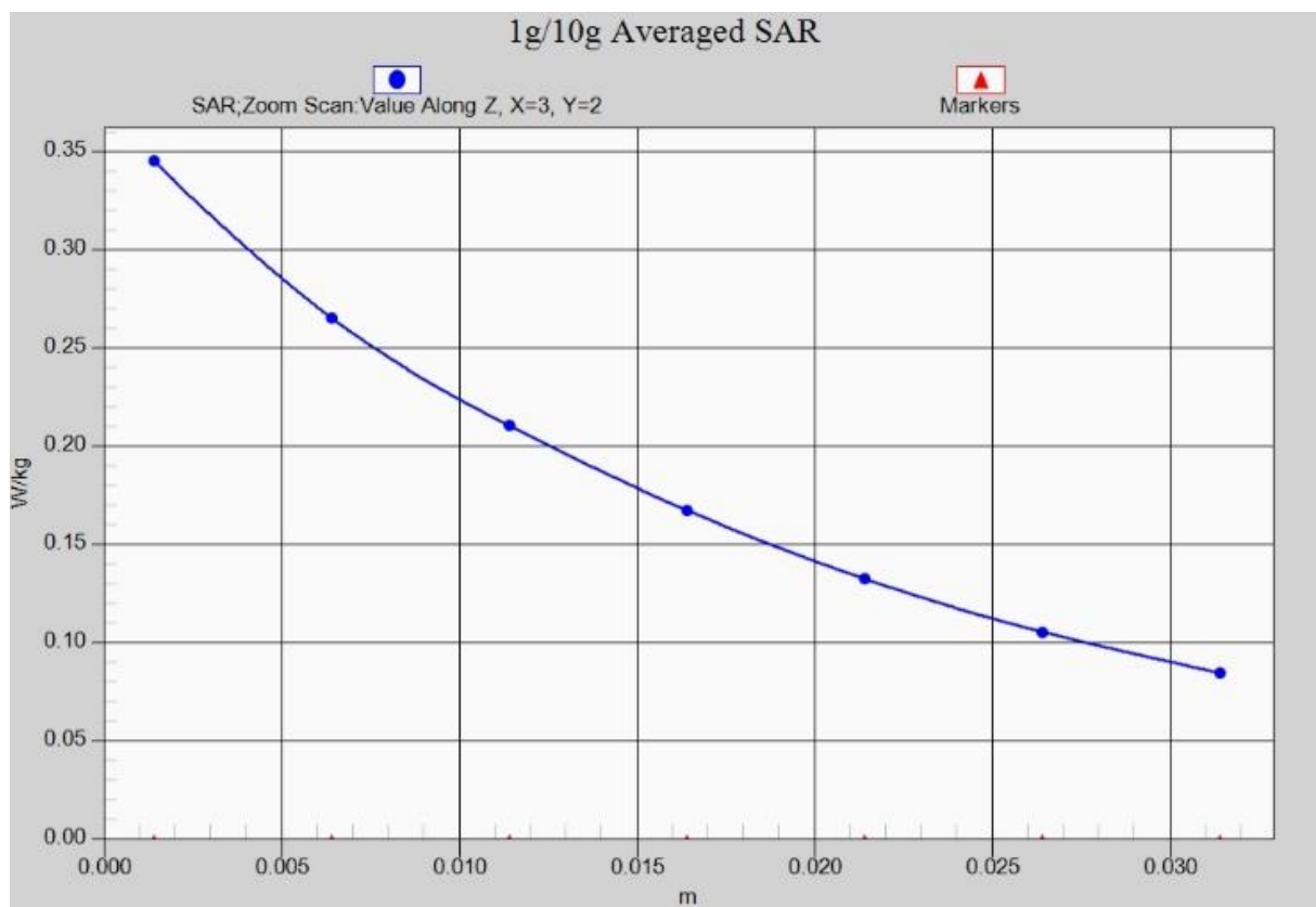
Fig.1- 6 Z-Scan at power reference point (W850)
