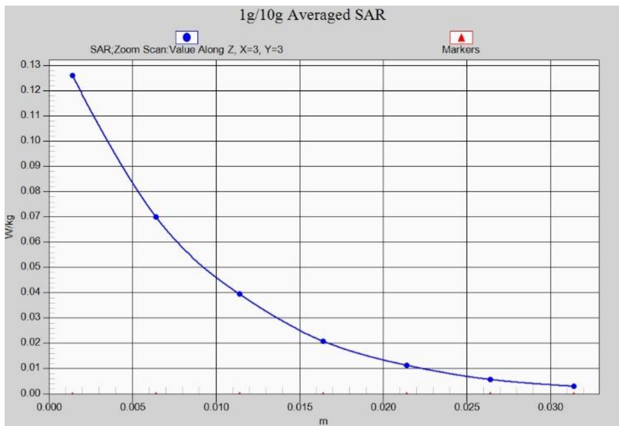
Fig.1- 8 Z-Scan at power reference point (WLAN)
