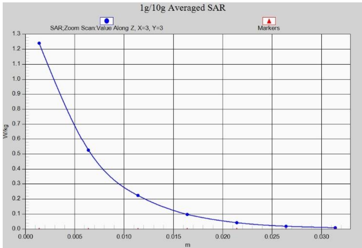
Fig.1- 7 Z-Scan at power reference point (WLAN)
