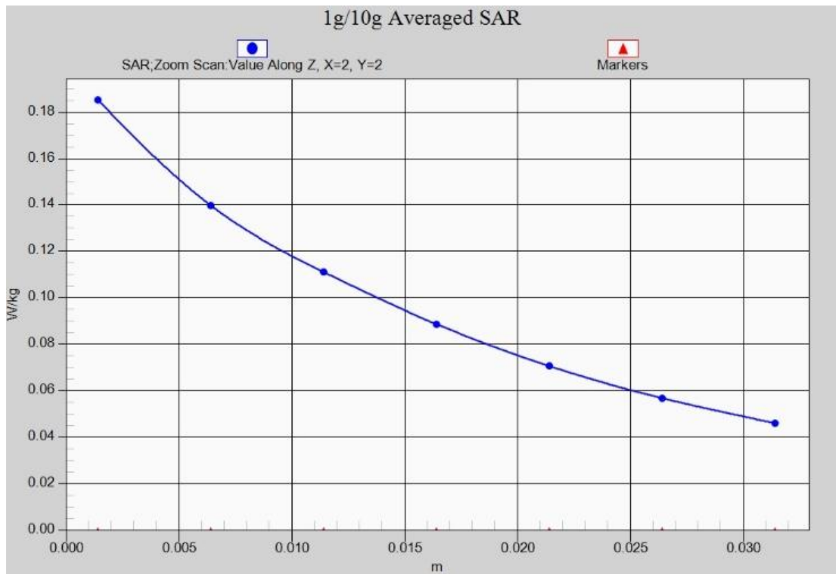
Fig.1- 5 Z-Scan at power reference point (W850)
