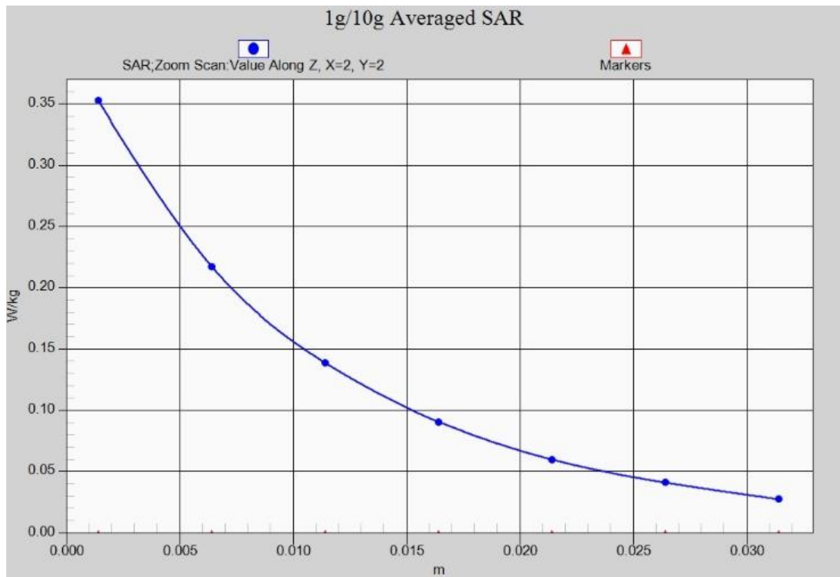
Fig.1- 9 Z-Scan at power reference point (W1900)
