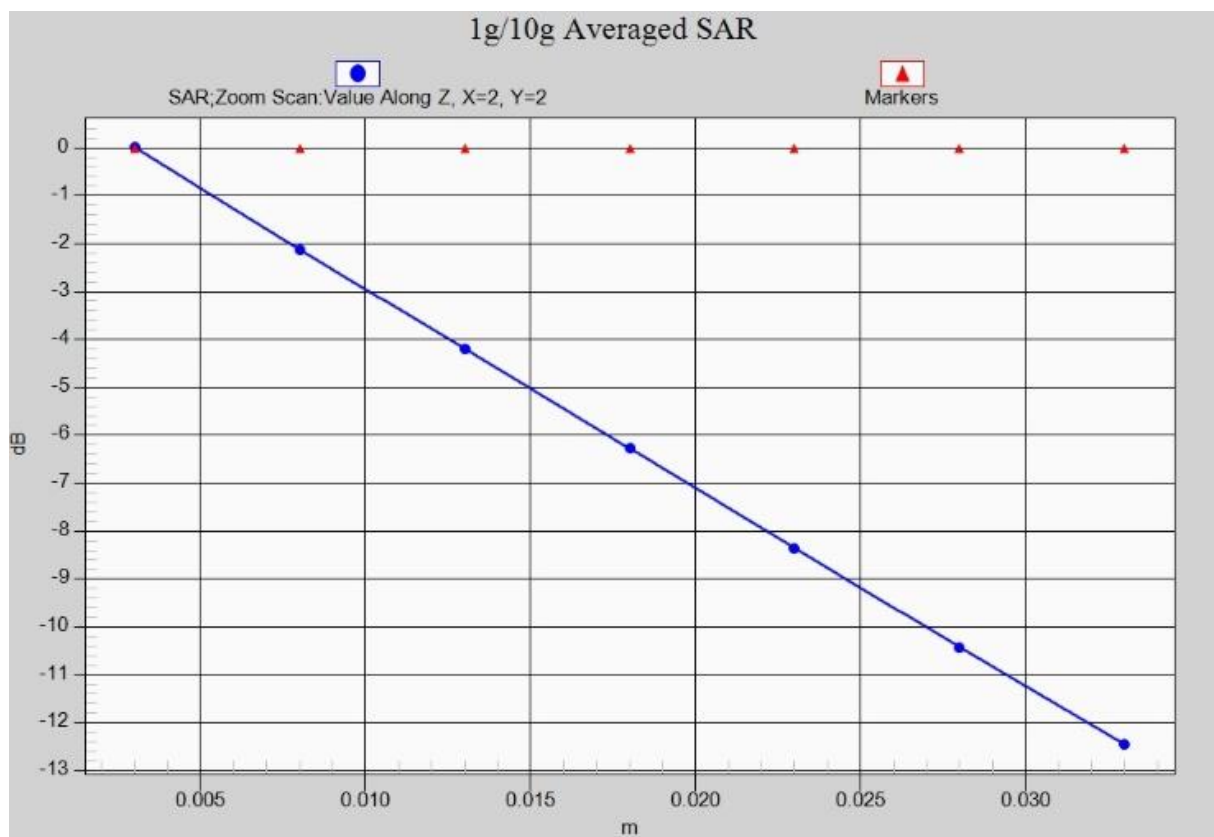
Fig.1- 10 Z-Scan at power reference point (W1900)
