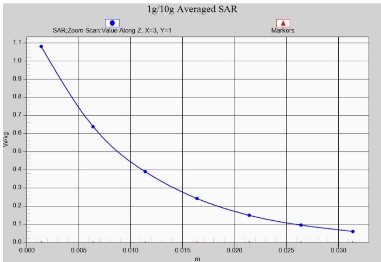
Fig.1- 6 Z-Scan at power reference point (W1700)
