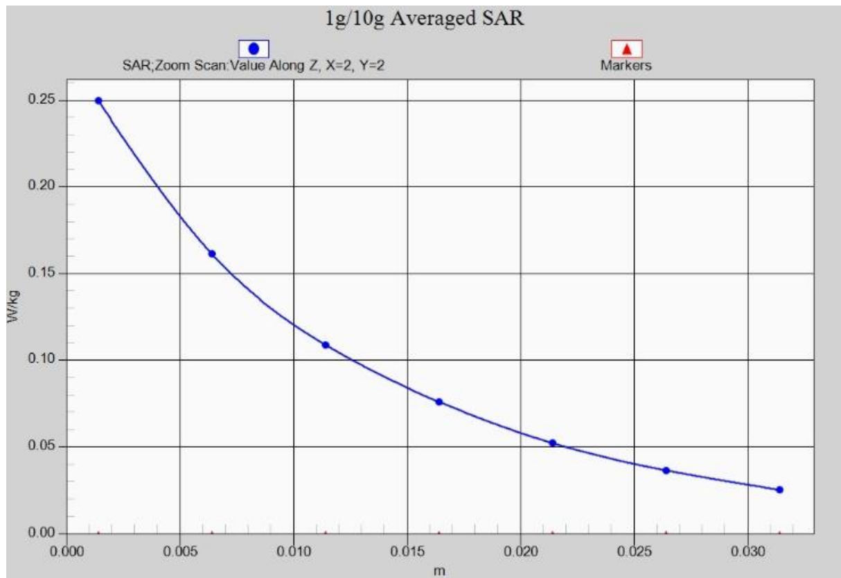
Fig. 1- 5 Z-Scan at power reference point (W1700)
