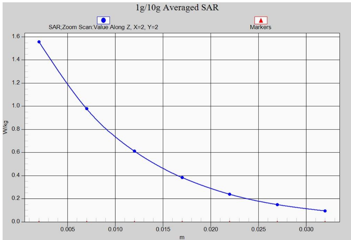
Fig.1- 4 Z-Scan at power reference point (PCS1900)
