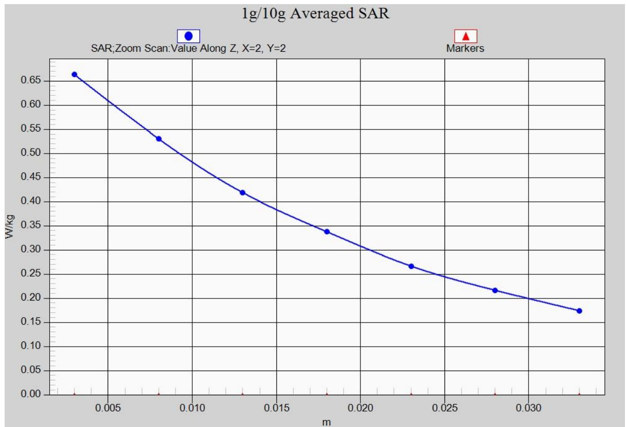
Fig.1- 2 Z-Scan at power reference point (GSM850)
