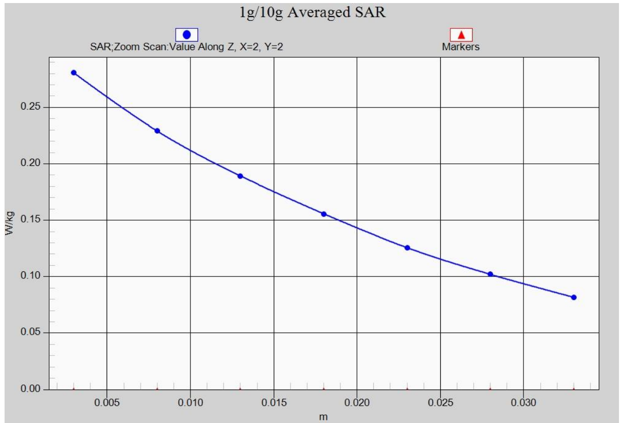
Fig.1- 1 Z-Scan at power reference point (GSM850)
