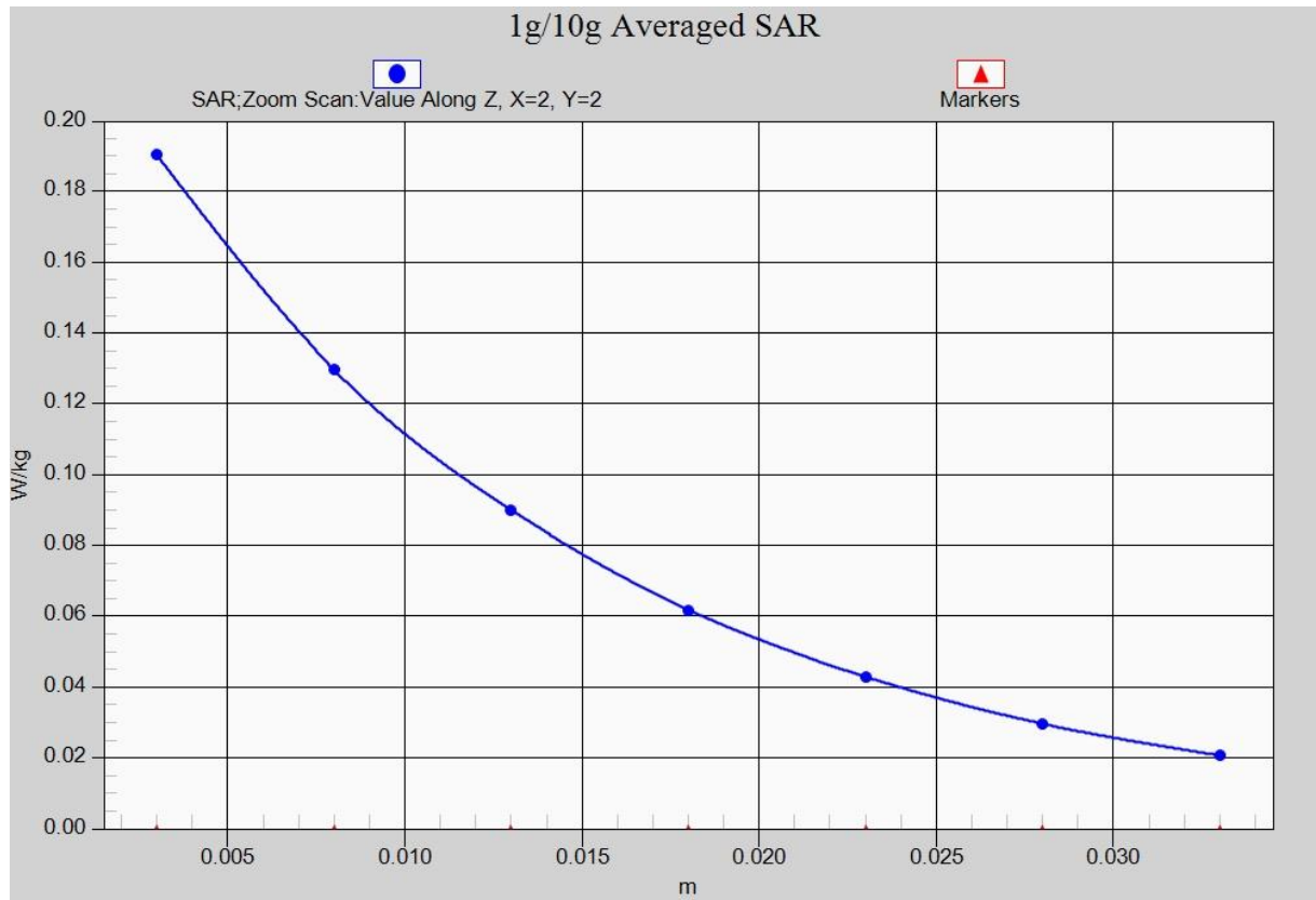
Fig.1- 3 Z-Scan at power reference point (PCS1900)
