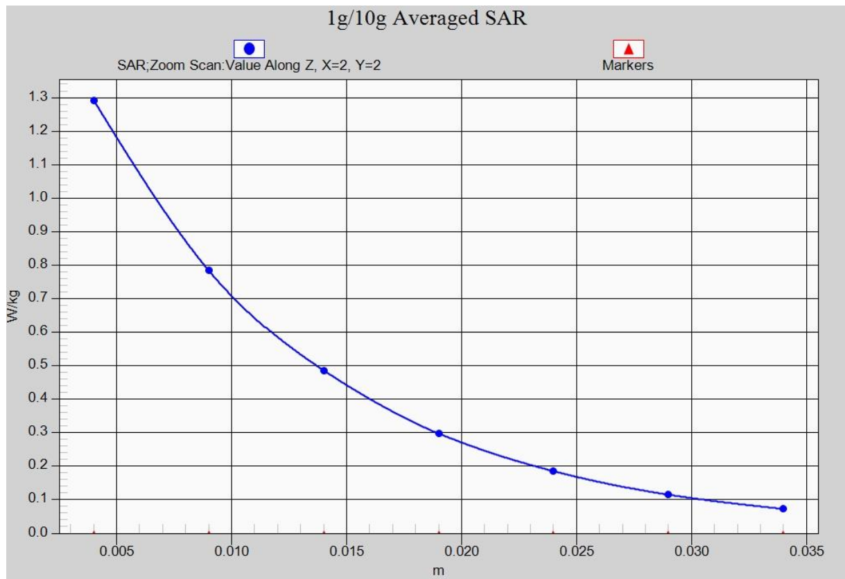
Fig. 24-1 Z-Scan at power reference point (WCDMA1700)
