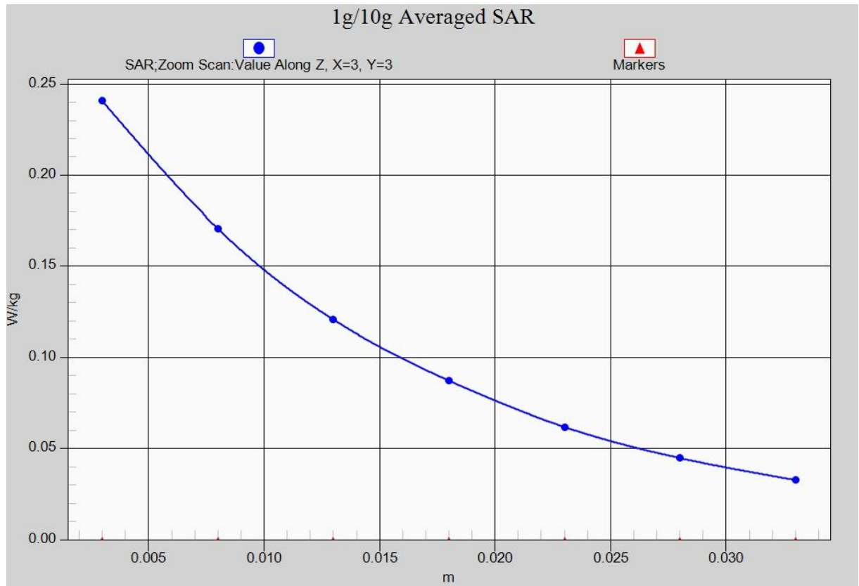
Fig. 23-1 Z-Scan at power reference point (WCDMA1700)
