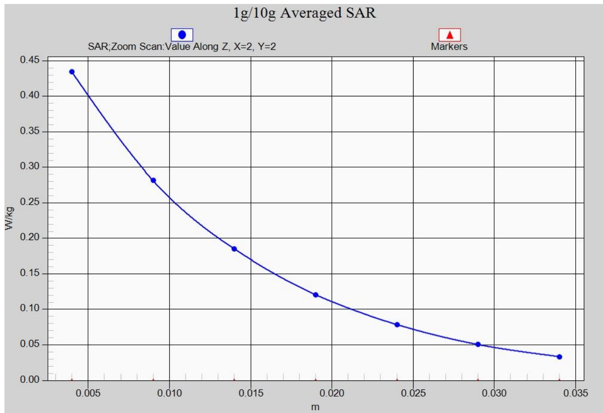
Fig. 25-1 Z-Scan at power reference point (WCDMA1700)
