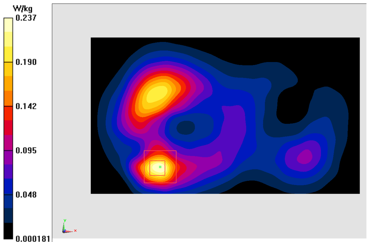
Fig.27 2450 MHz
