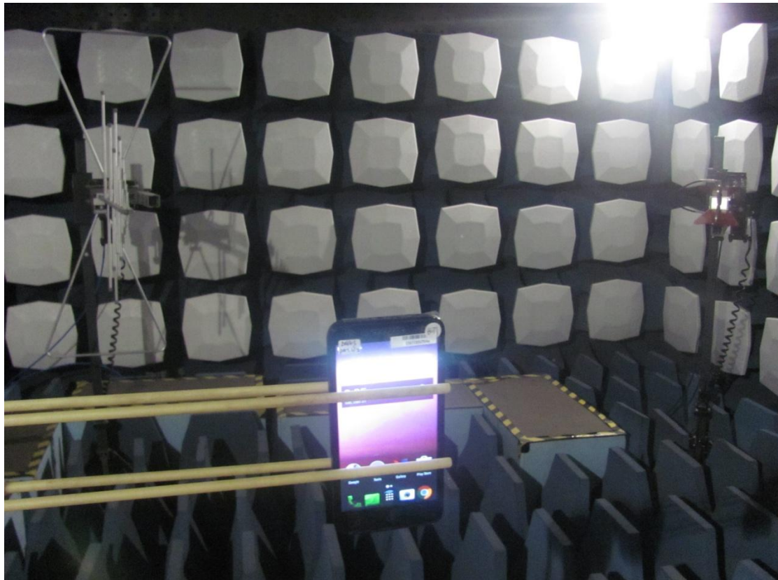
Radiated Spurious Emission_New
