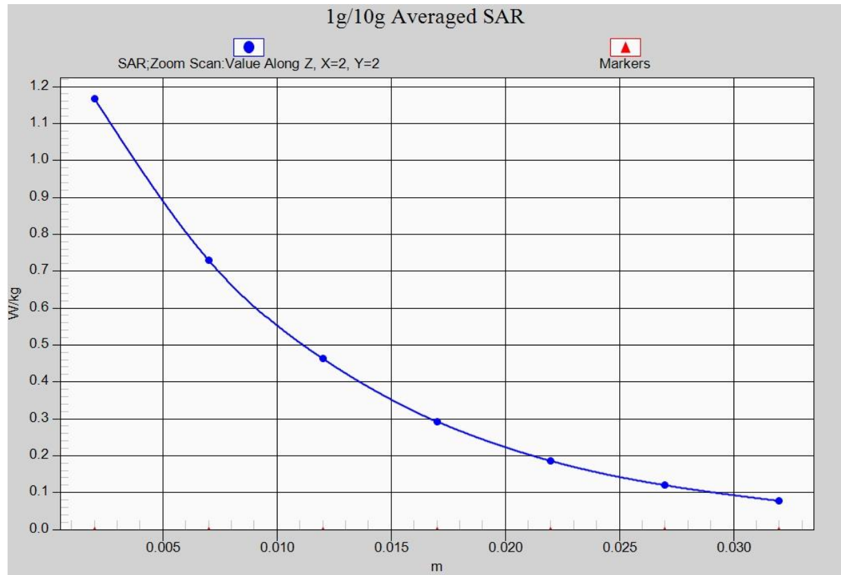
Fig. 20-1 Z-Scan at power reference point (LTE Band66)
