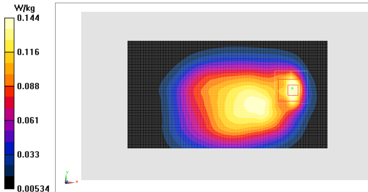
Fig.2 850 MHz
