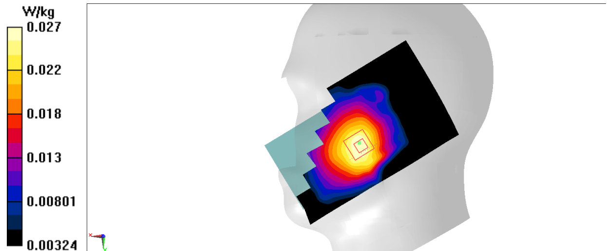
Fig.1 850MHz
