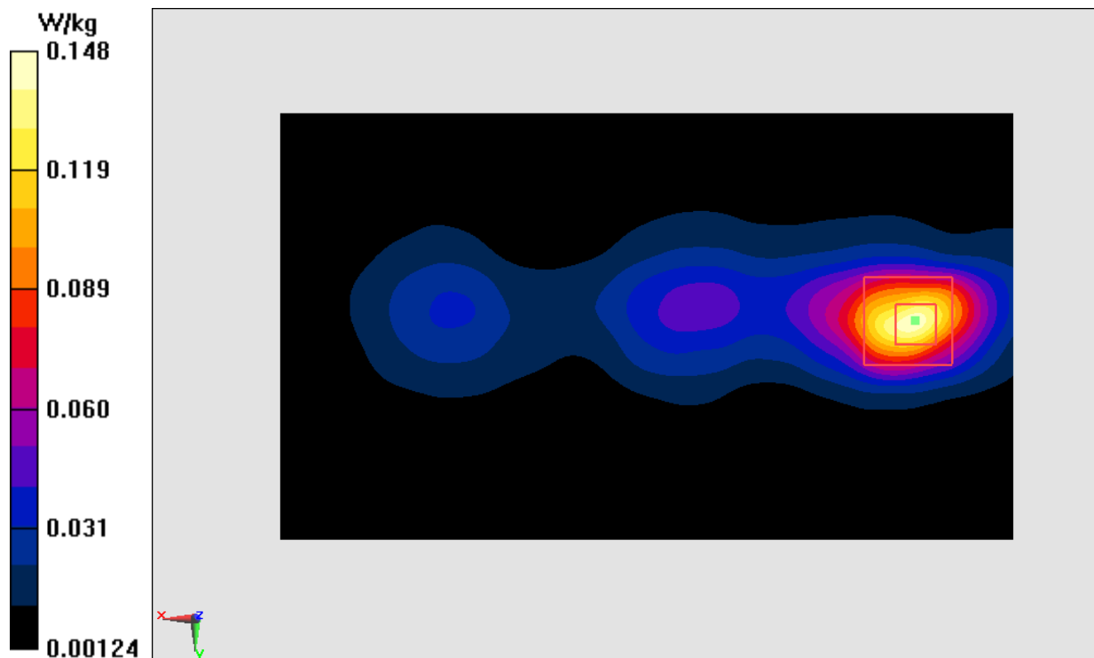
Fig.34 2450 MHz
