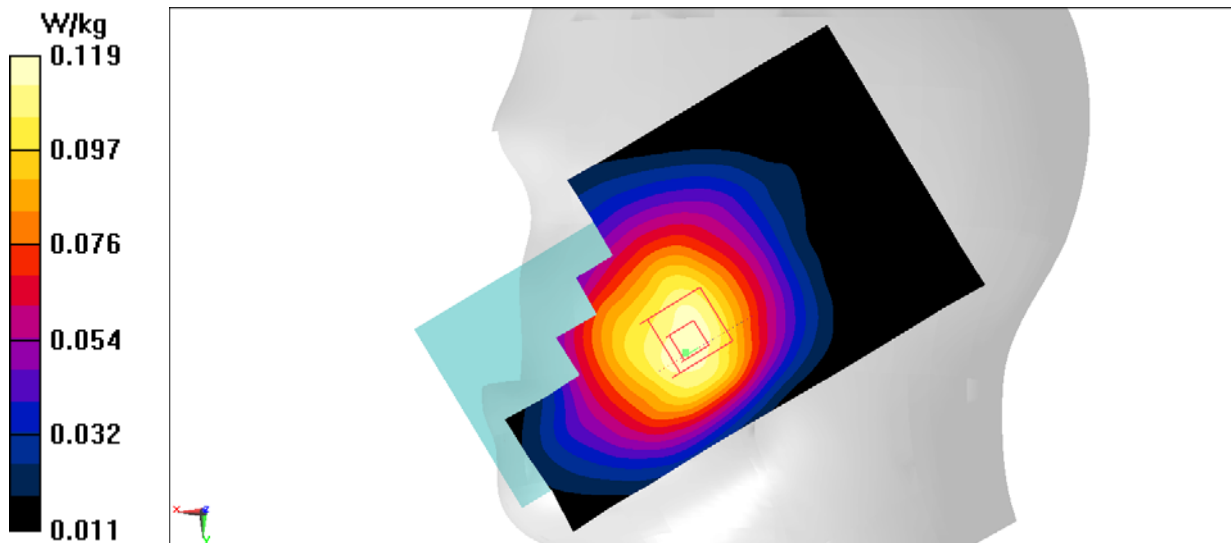
Fig.24 LTE Band12
