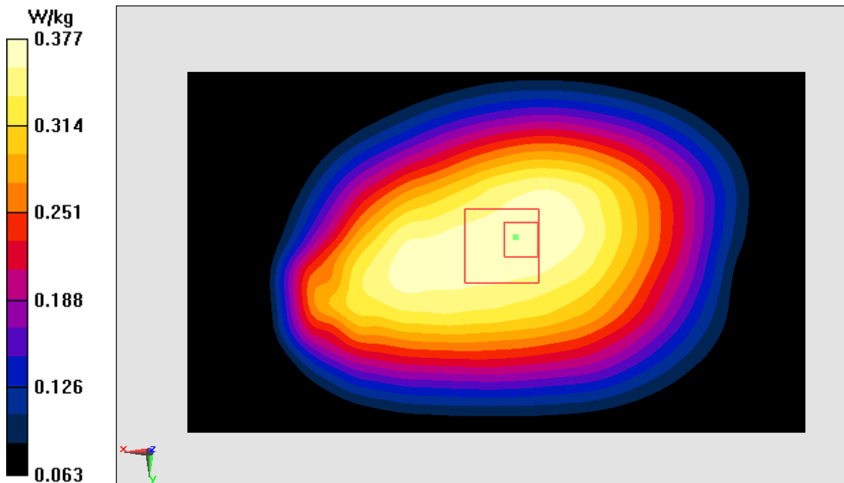
Fig.29 CDMA BC0
