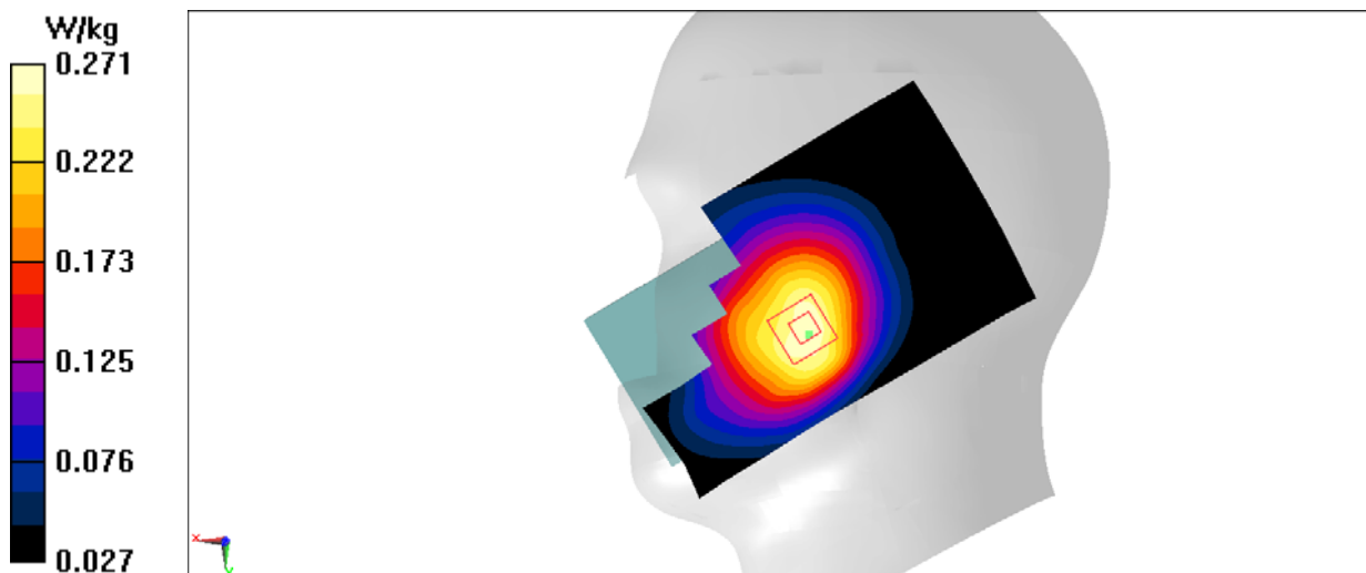
Fig.28 CDMA BC0
