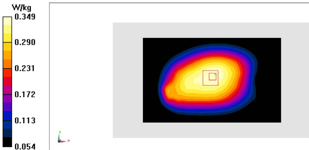
Fig.20 LTE Band5
