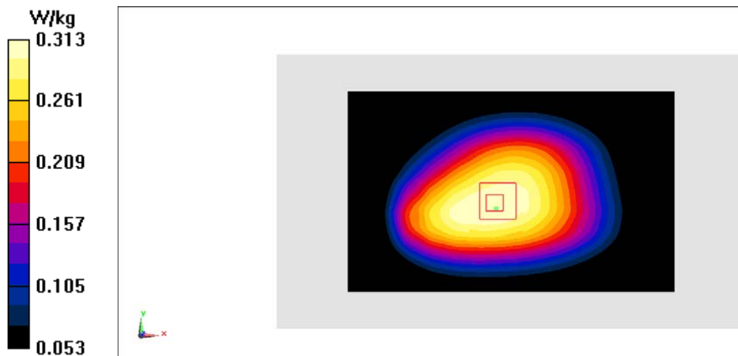
Fig.25 LTE Band12
