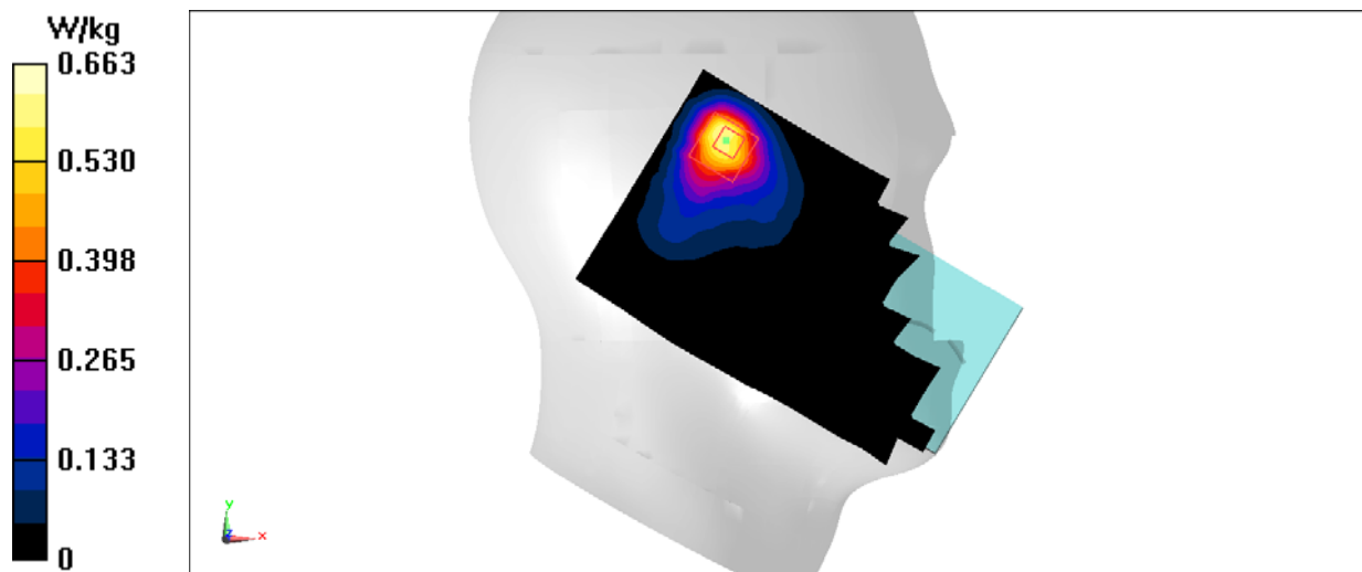
Fig.33 2450 MHz
