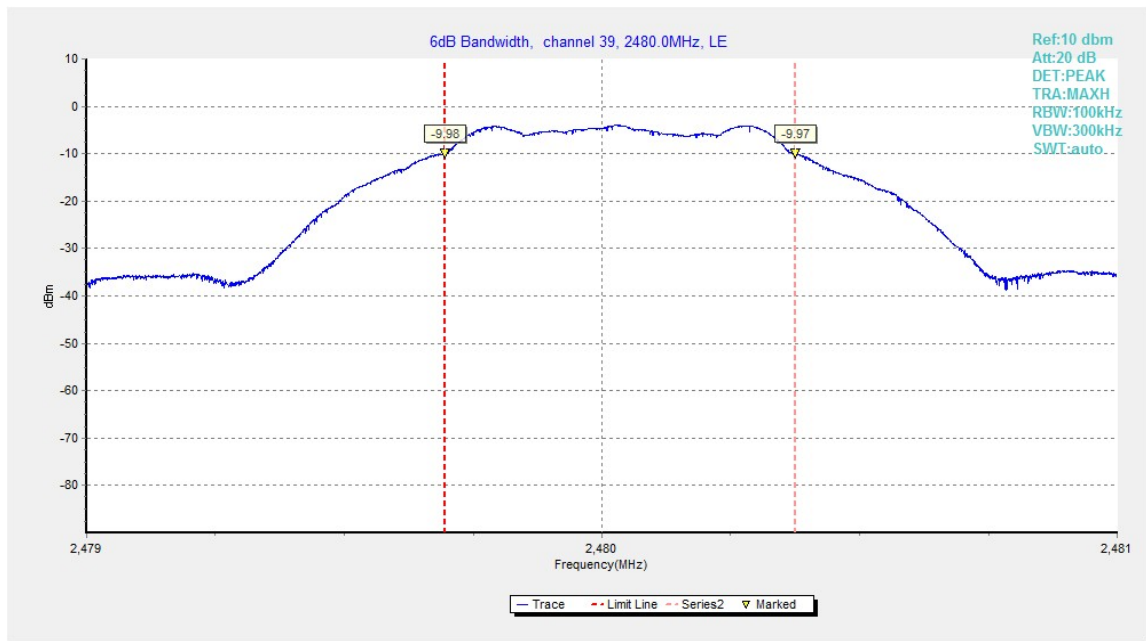
Fig.31. 6dB Bandwidth: GFSK, 2480 MHz
